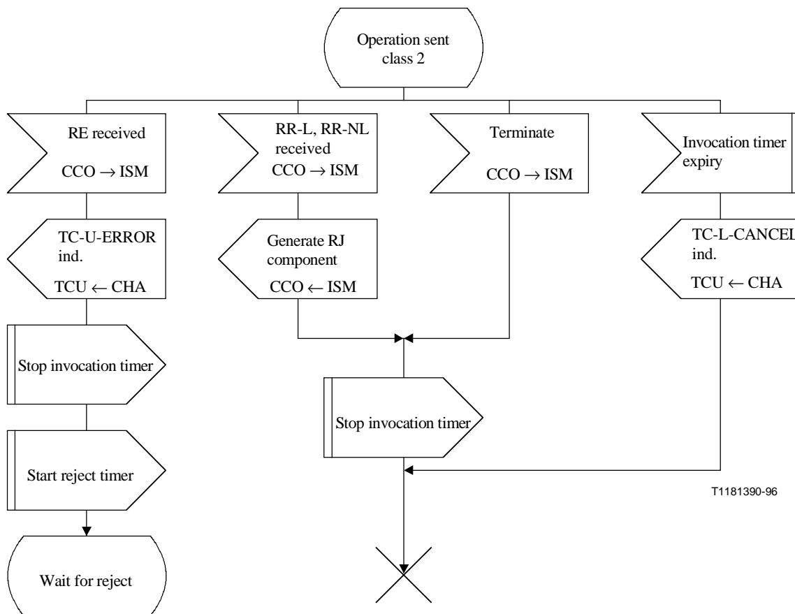
Figure A.7/Q.774 (sheet 4 of 6) – Invocation state machine
