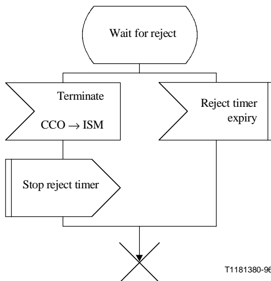
Figure A.7/Q.774 (sheet 3 of 6) – Invocation state machine
