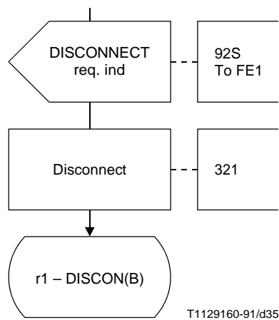
FIGURE 1-21/Q.84 (sheet 9 of 12) FE2 process MCCC
