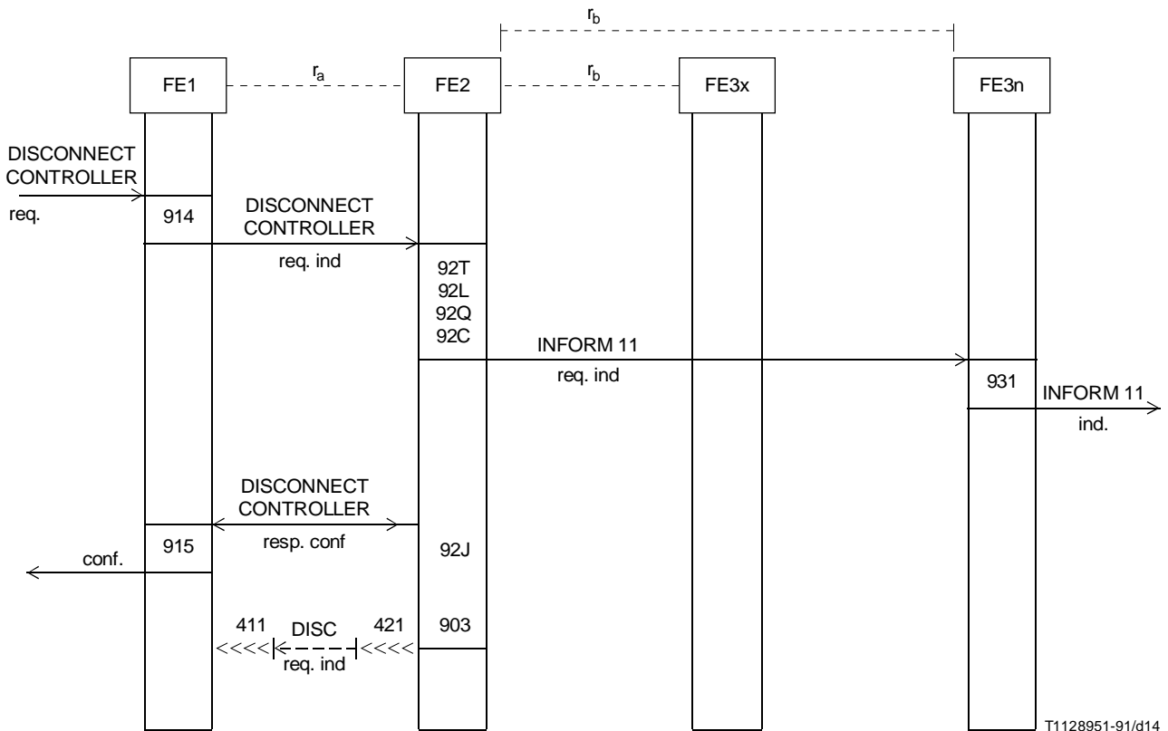
FIGURE 1-14/Q.84 Disconnect controller
