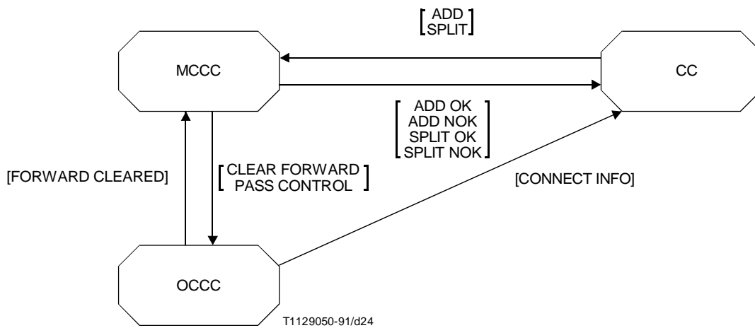
FIGURE 1-19/Q.84 Block diagram for FE2
