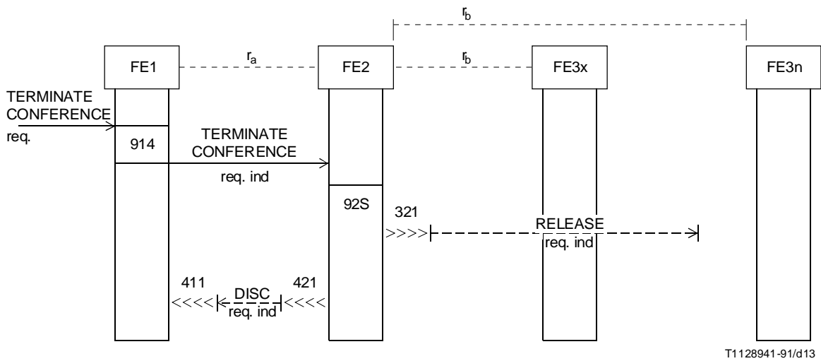
FIGURE 1-13/Q.84 Terminate conference
