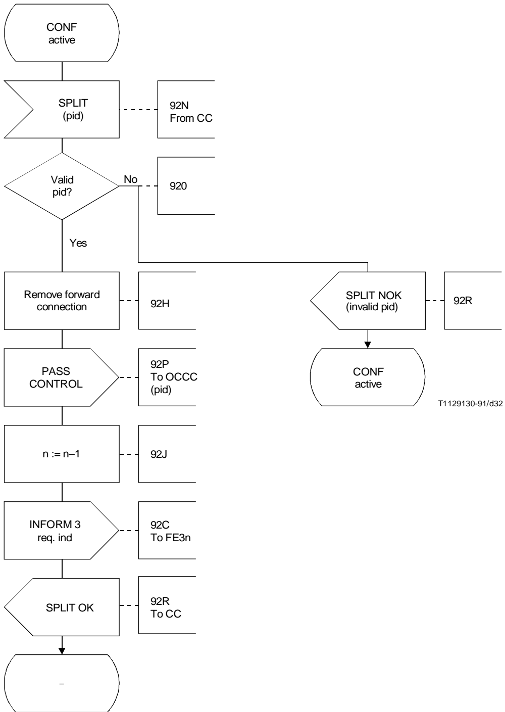
FIGURE 1-21/Q.84 (sheet 6 of 12) FE2 process MCCC
