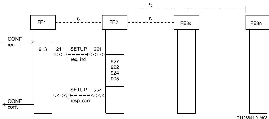
FIGURE 1-3/Q.84 Requesting a new conference call
