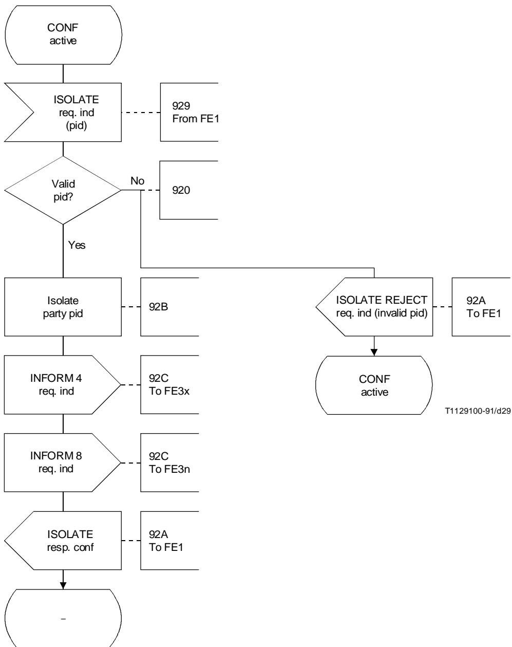
FIGURE 1-21/Q.84 (sheet 3 of 12)
