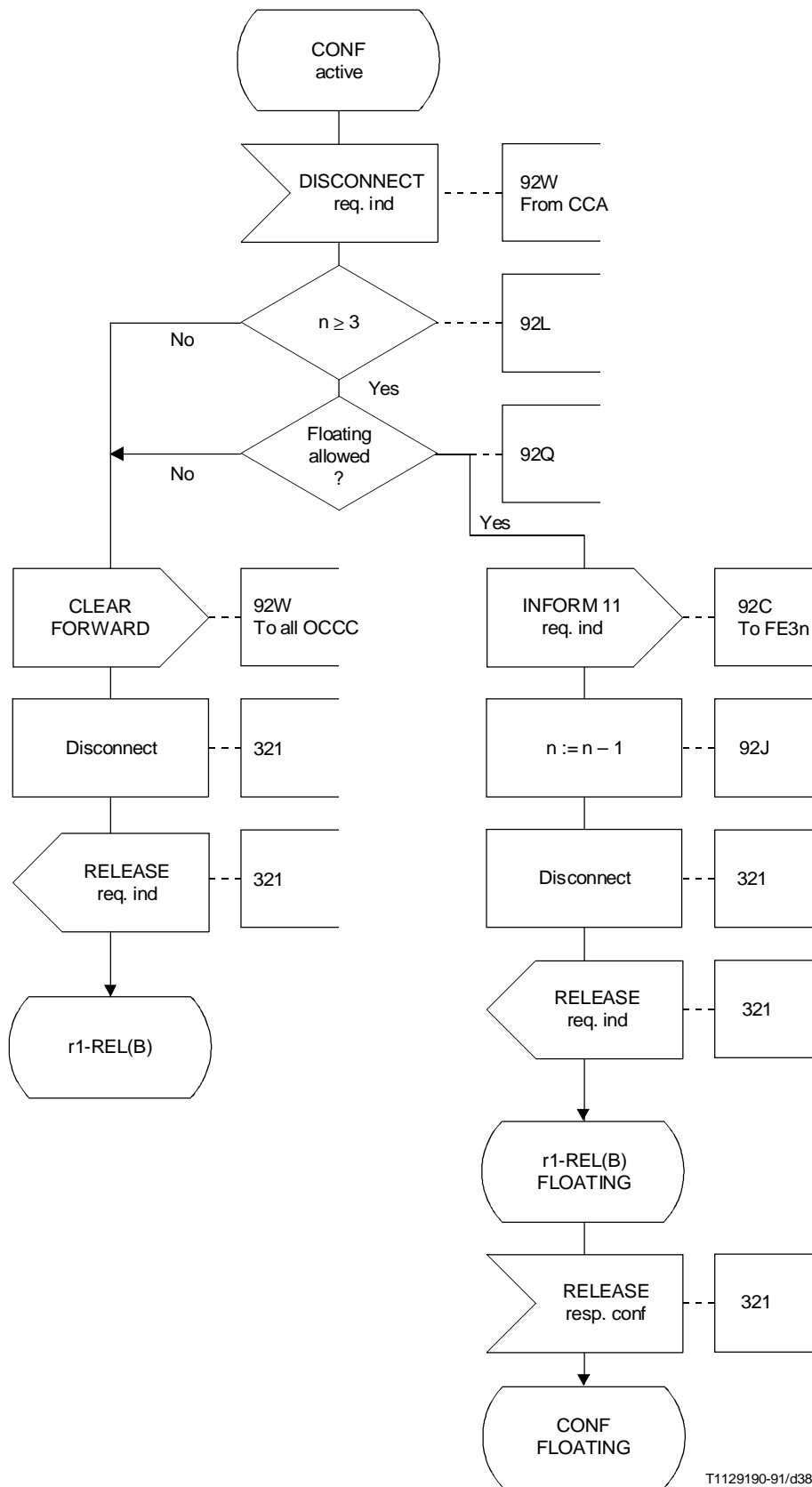
FIGURE 1-21/Q.84 (sheet 12 of 12)
