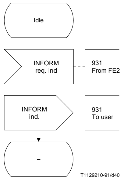
FIGURE 1-23/Q.84 Process FE3
