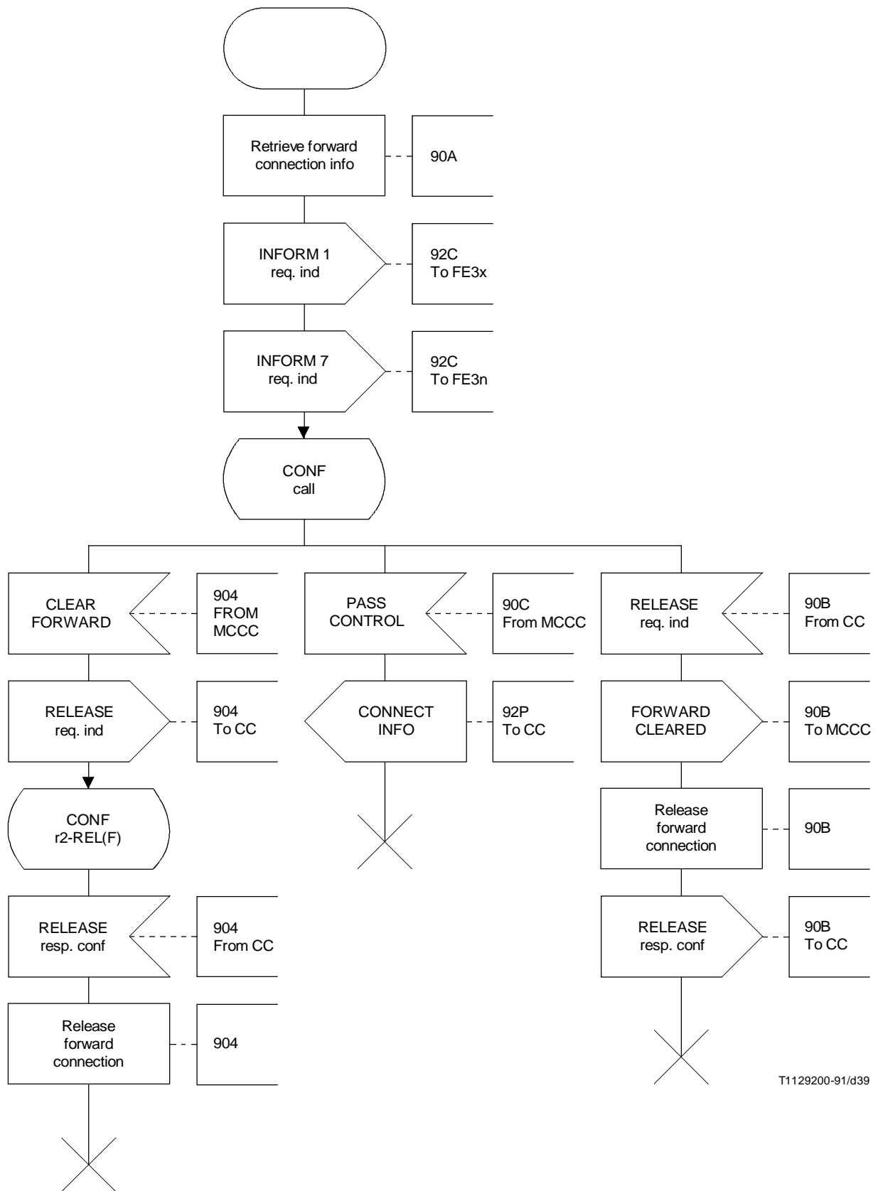
FIGURE 1-22/Q.84 Process OCCC
