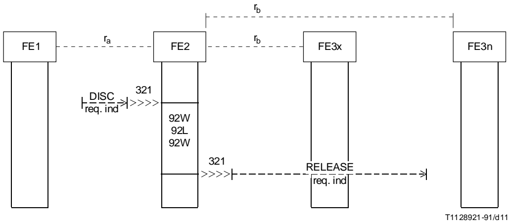
FIGURE 1-11/Q.84 Disconnect when floating is not allowed
