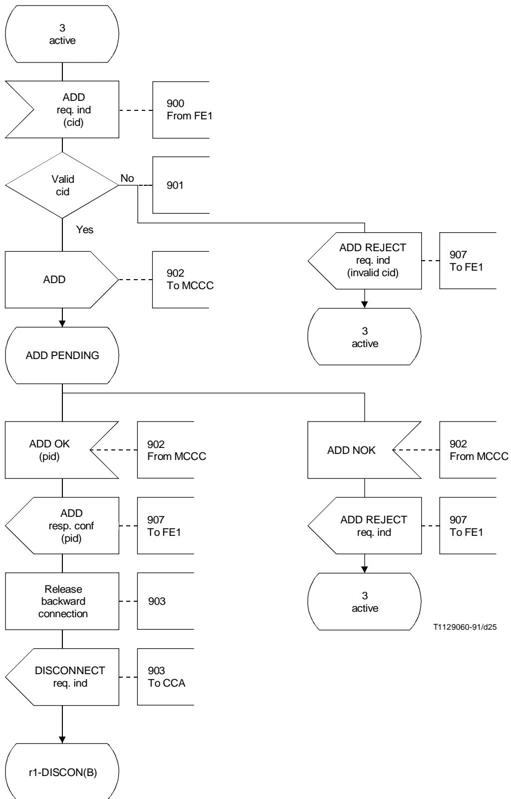
FIGURE 1-20/Q.84 (sheet 1 of 2)
