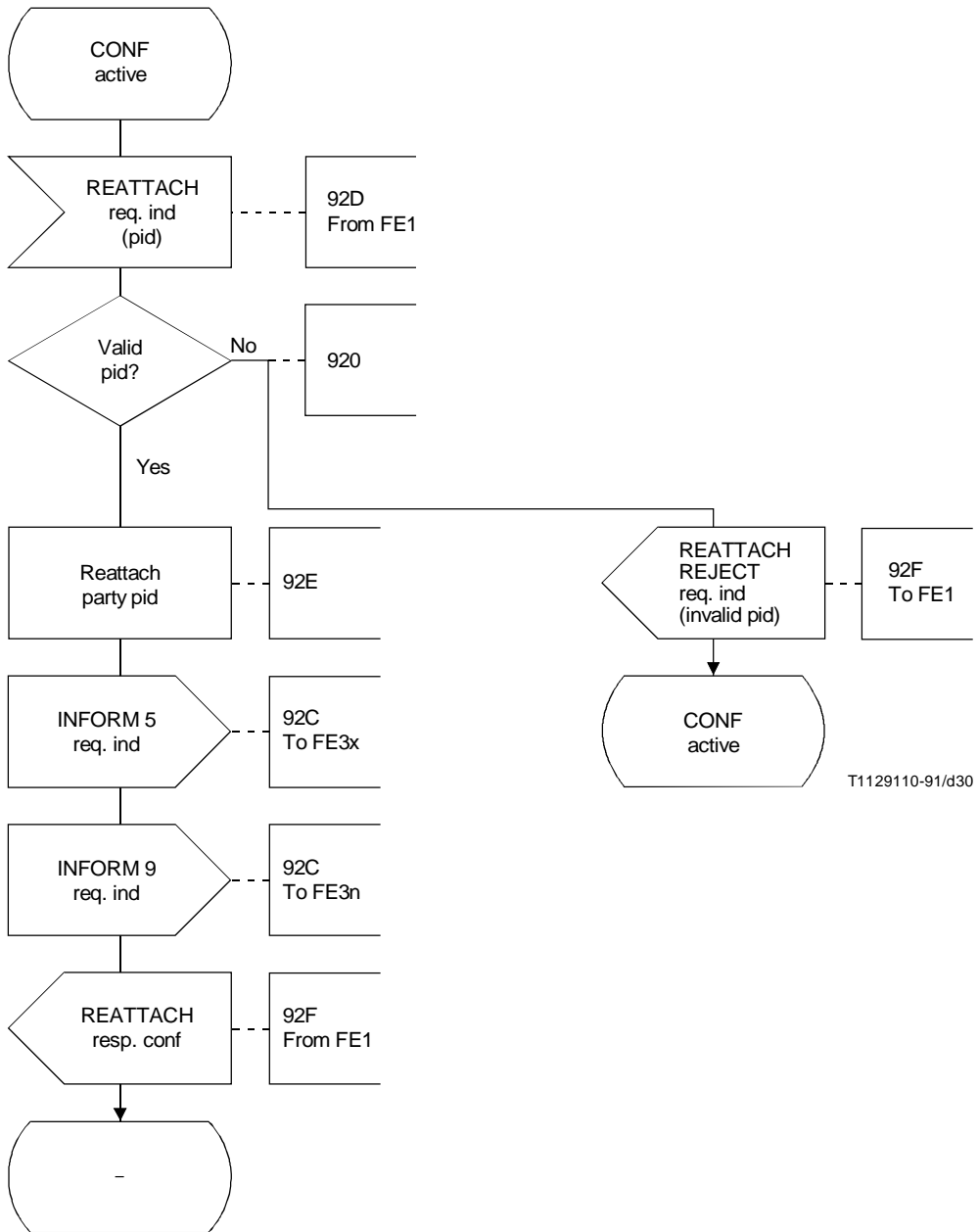
FIGURE 1-21/Q.84 (sheet 4 of 12)
