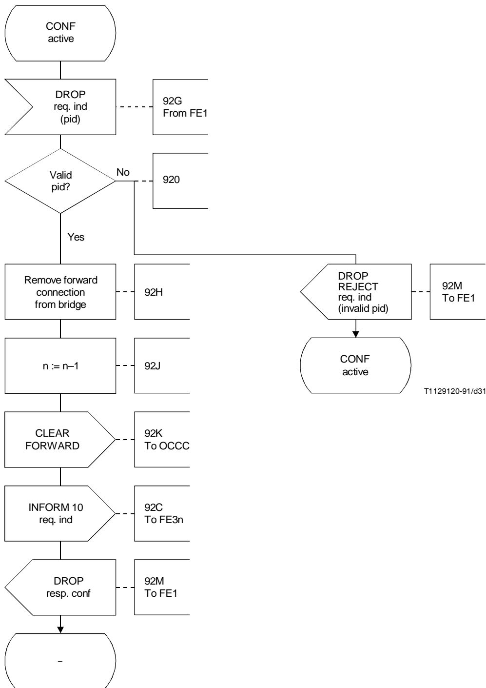
FIGURE 1-21/Q.84 (sheet 5 of 12) FE2 process MCCC
