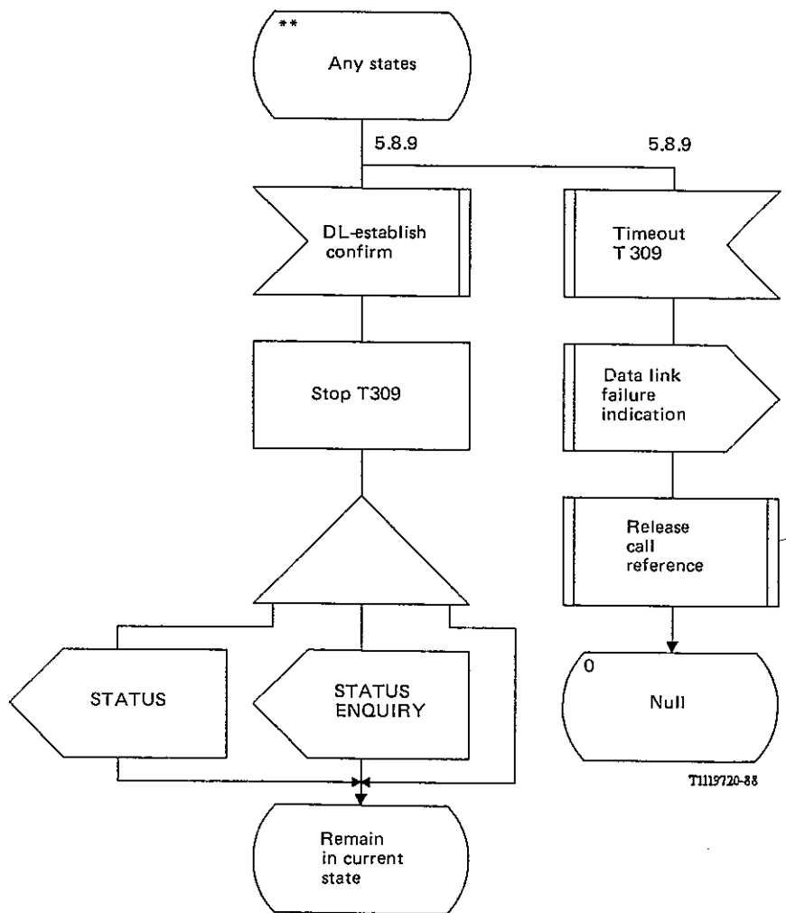
FIGURE A-6/Q.931 (Sheet 27 of 27)
