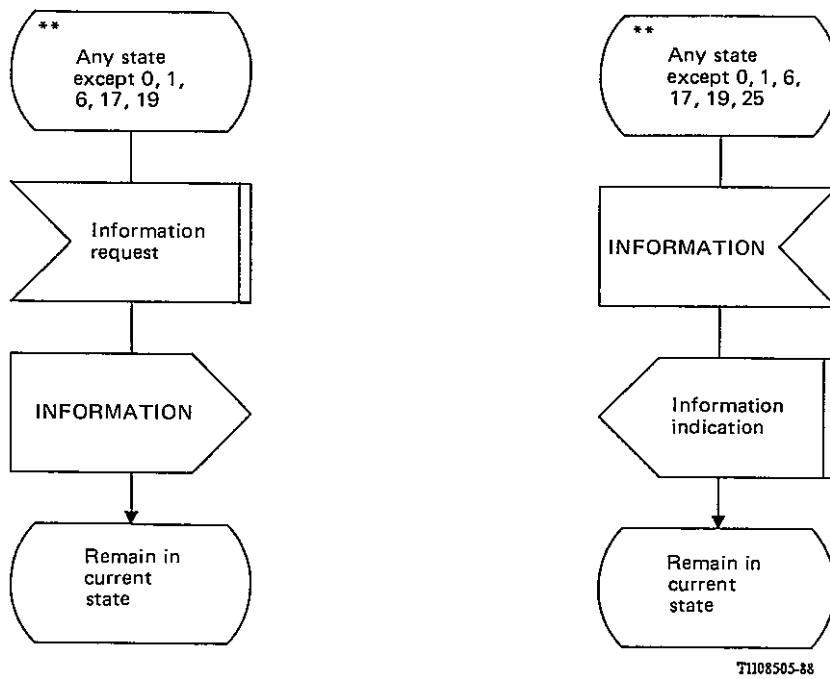
FIGURE A-3/Q.931 (Sheet 18 of 25)
