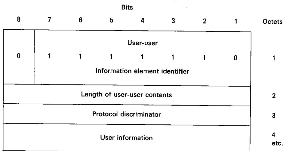
FIGURE 4-37/Q.931 User-user information element
