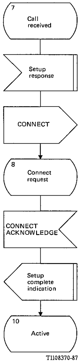
b) Incoming setup procedure (2 of 2)
