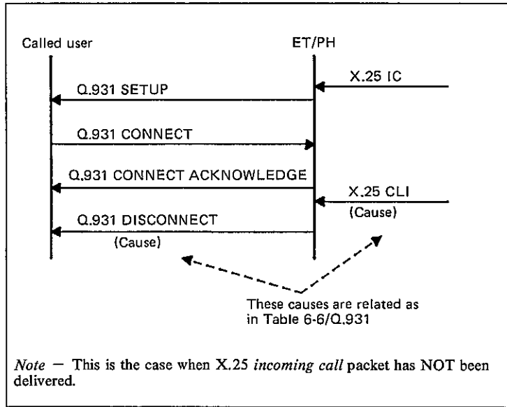
FIGURE II-16/Q.931 Premature clearing of the virtual circuit
