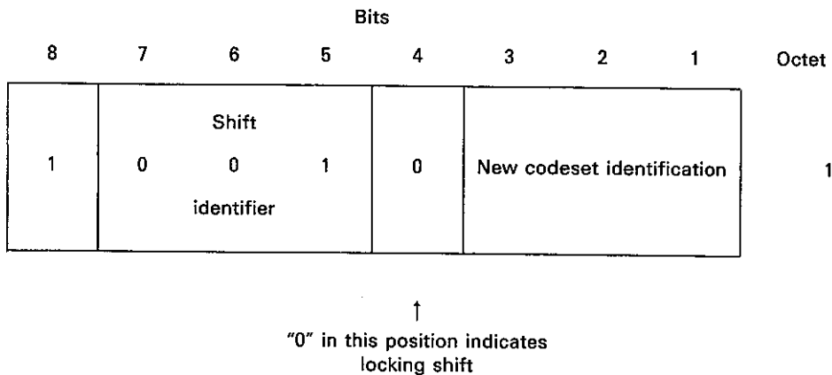
FIGURE 4-9/Q.931 Locking Shift information element
