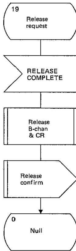
c) Clearing procedure (2 of 2)
