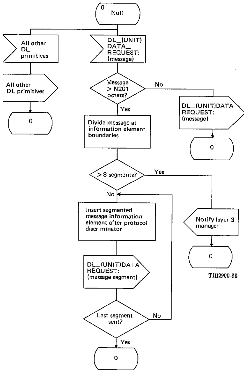
FIGURE K-4/Q.931 Message segmenter SDL
