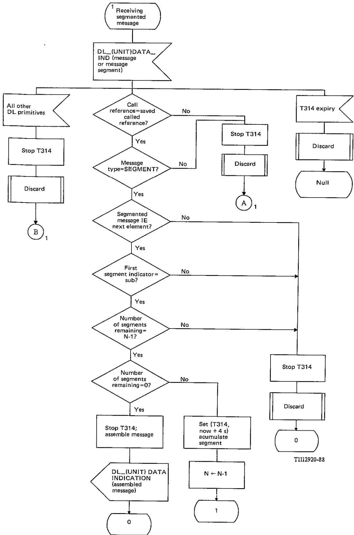
FIGURE K-5/Q.931 (Sheet 2 of 3)
