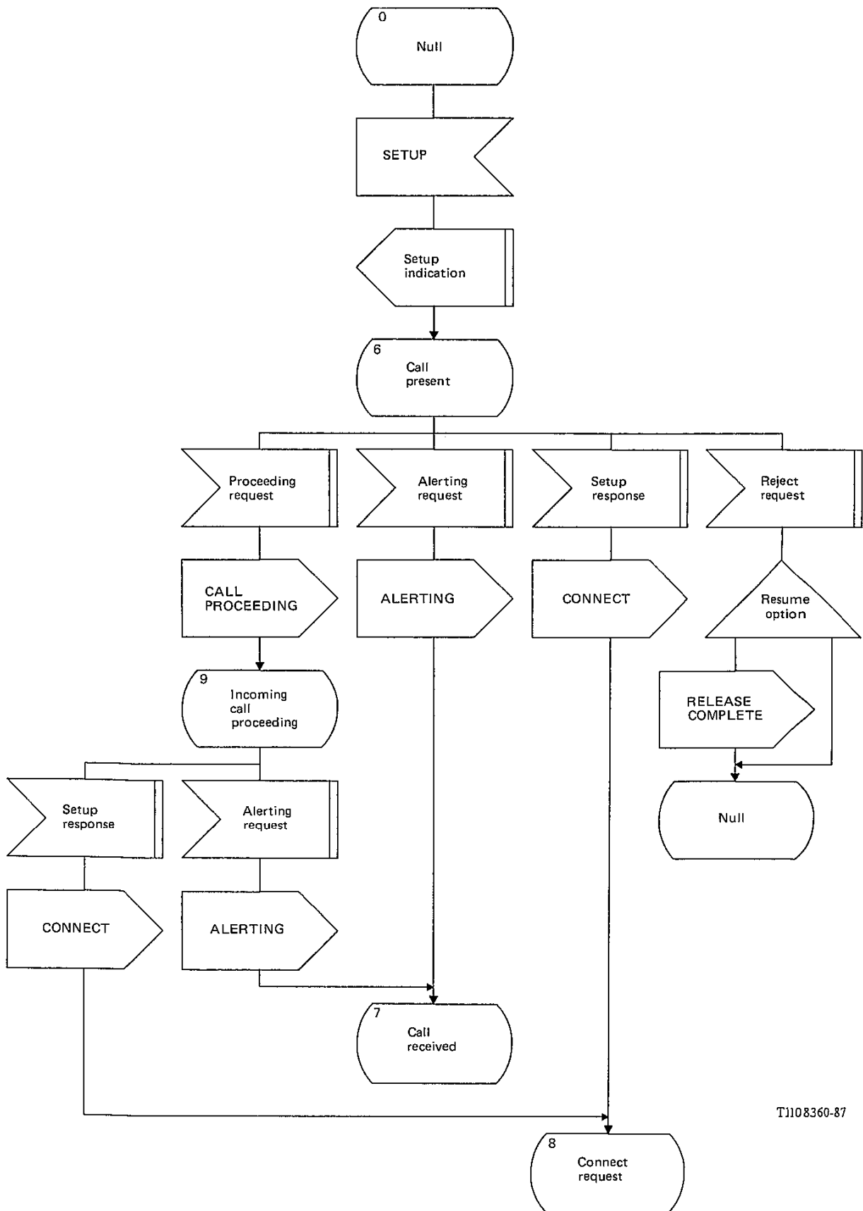
b) Incoming setup procedure (1 of 2)
