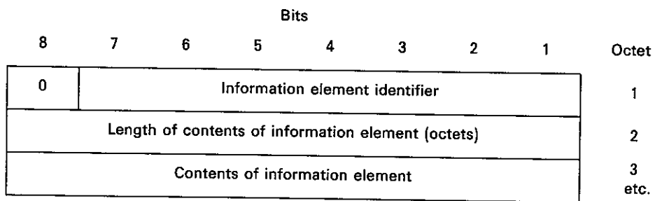
c) Variable length information element format
