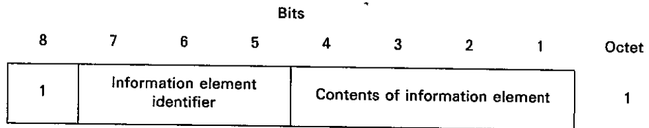
a) Single octet information element format (type 1)
