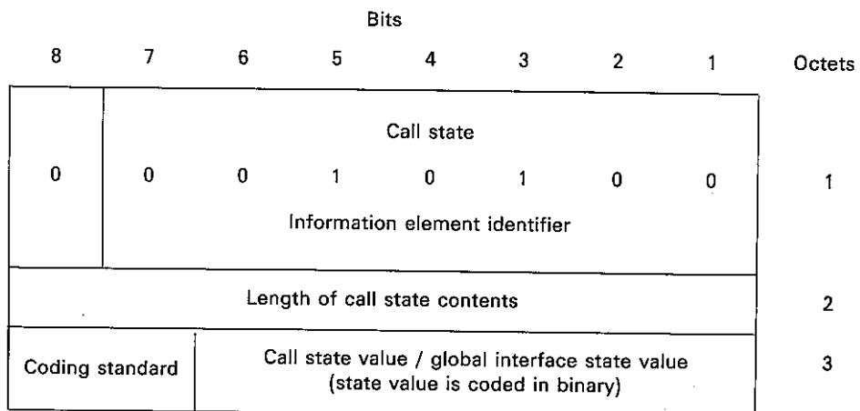
FIGURE 4-13/Q.931 Call state information element
