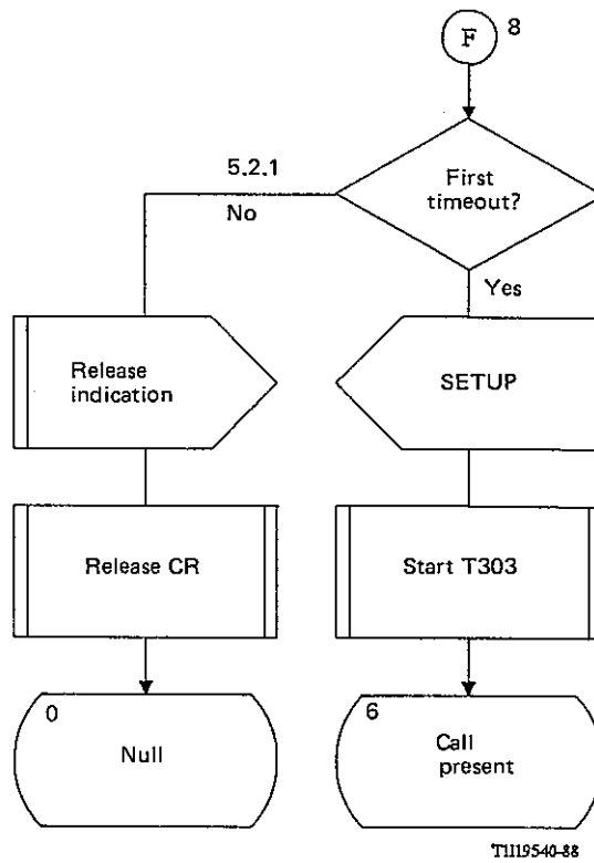
FIGURE A-6/Q.931 (Sheet 9 of 27) Detailed protocol control (network side) point-point
