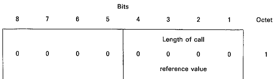
FIGURE 4-4/Q.931 Dummy call reference
