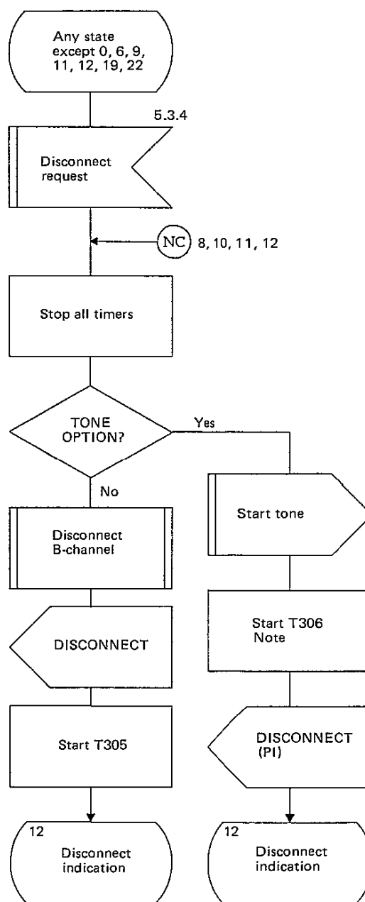
FIGURE A-6/Q.931 (Sheet 22 of 27) Detailed protocol control (network side) point-point
