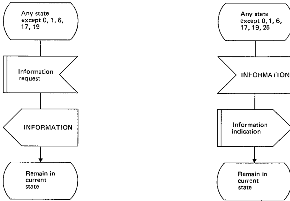
FIGURE A-6/Q.931 (Sheet 21 of 27) Detailed protocol control (network side) point-point
