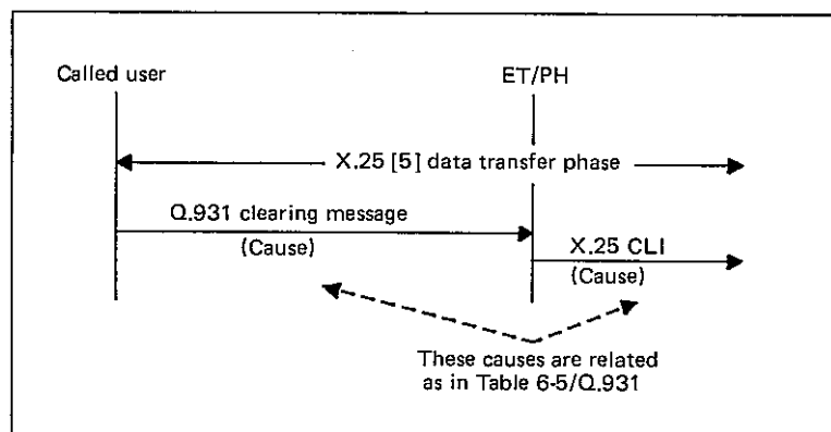
FIGURE II-13/Q.931 Q.931 clearing during X.25 data transfer phase
