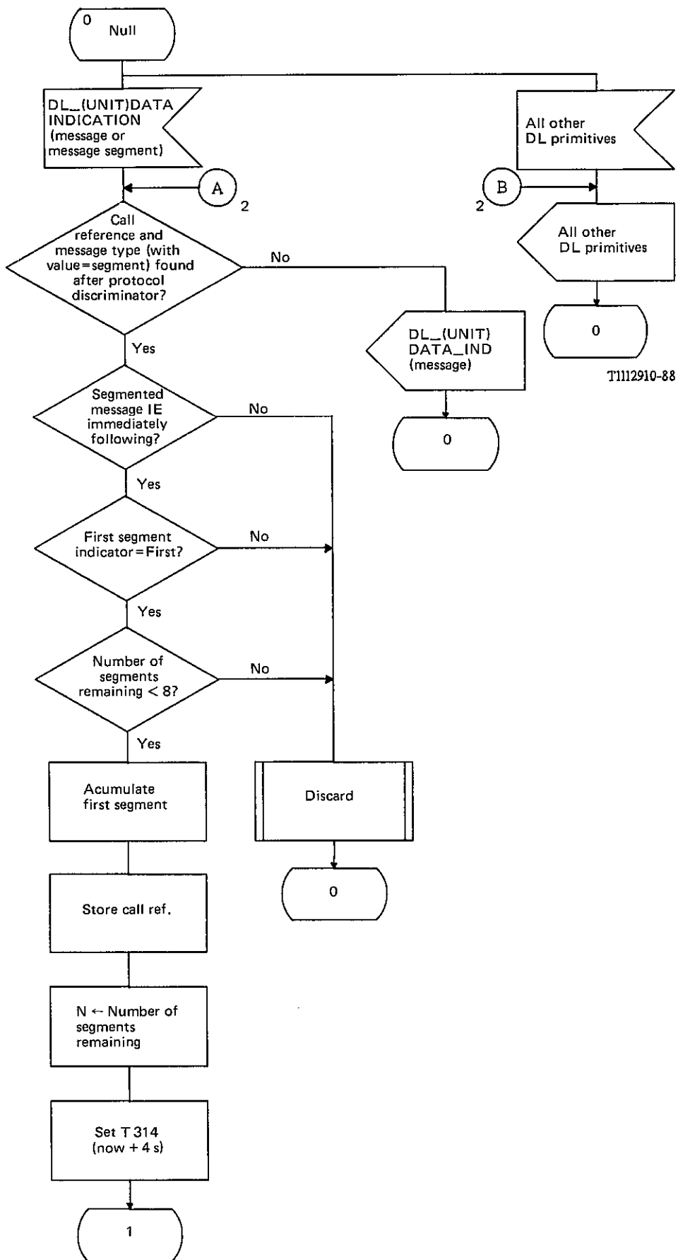
FIGURE K-5/Q.931 (Sheet 1 of 3)
