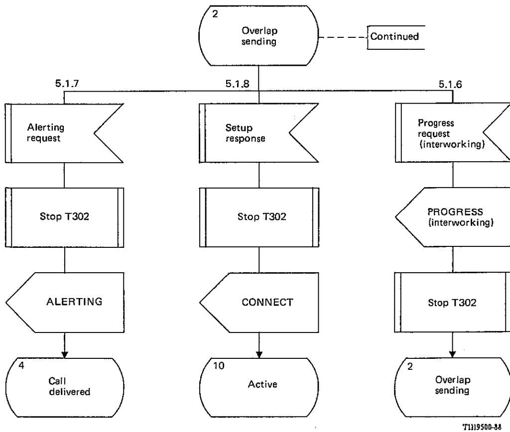
FIGURE A-6/Q.931 (Sheet 5 of 27)
