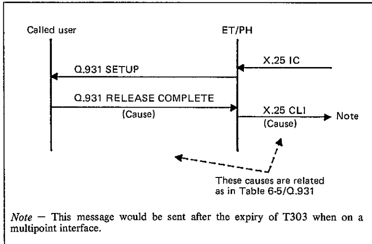
FIGURE II-12/Q.931 Call rejection by called party
