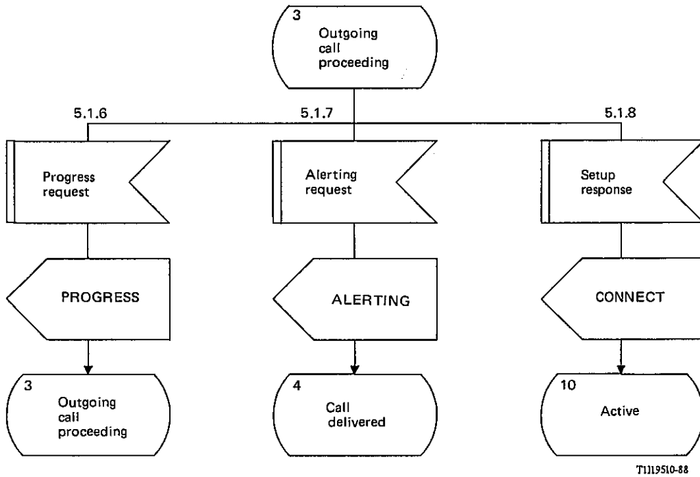
FIGURE A-6/Q.931 (Sheet 6 of 27) Detailed protocol control (network side) point-point
