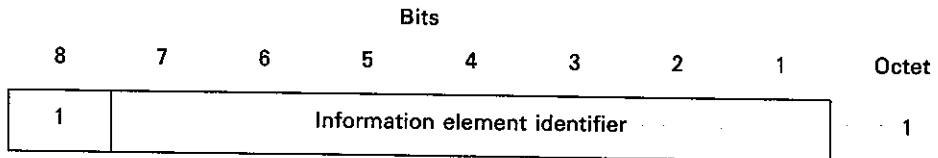
b) Single octet information element format (type 2)
