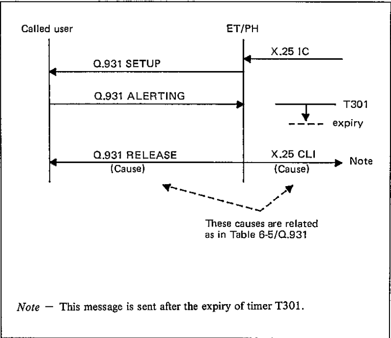
FIGURE II-11/Q.931 Expiry of timer T301
