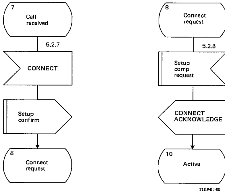
b) Incoming setup procedure (2 of 2)
