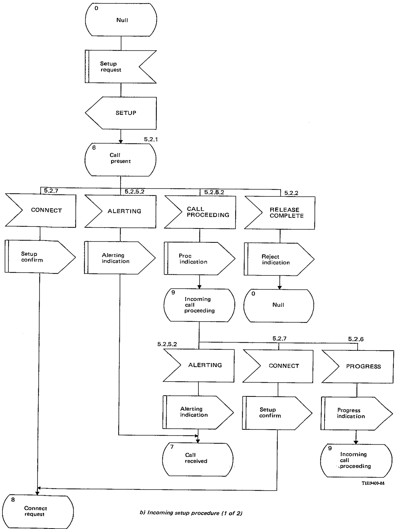
FIGURE A-5/Q.931 (Sheet 3 of 8) Overview protocol control (network side) point-point
