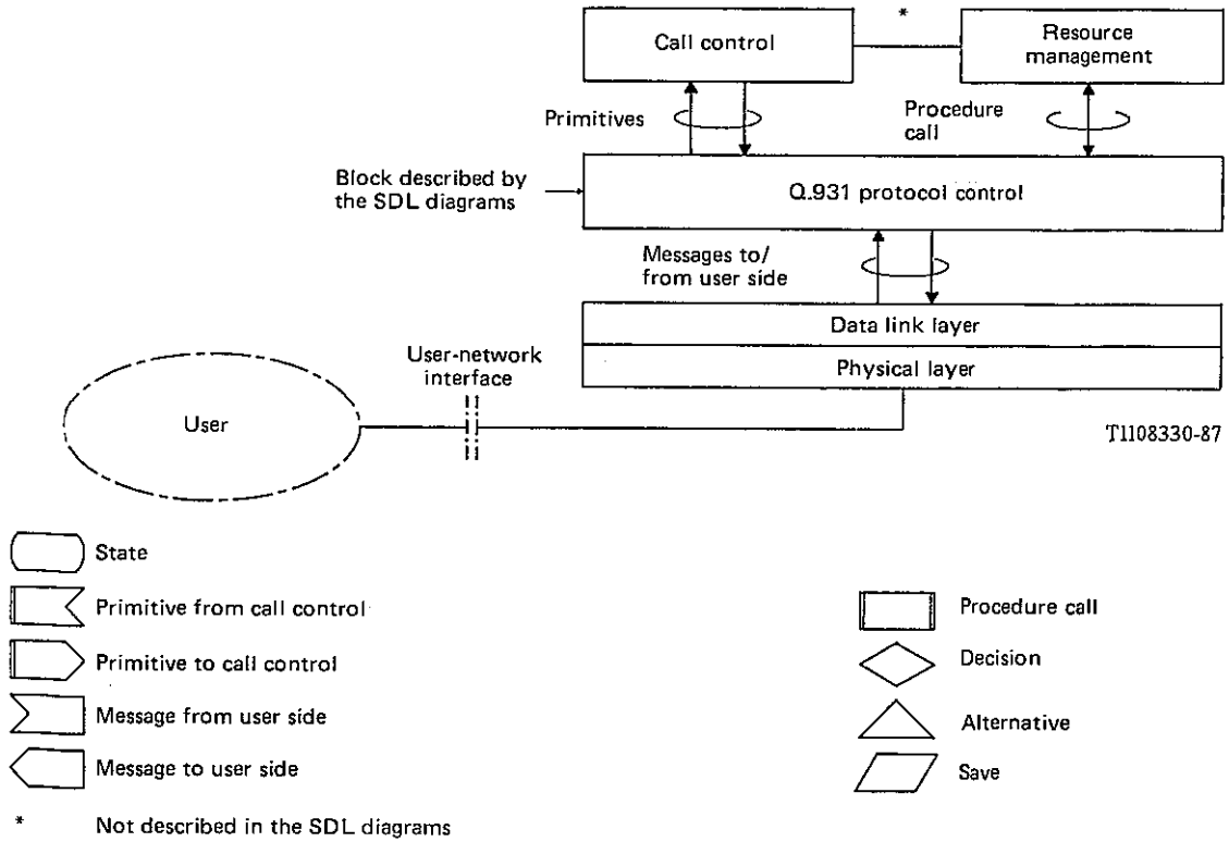
FIGURE A-1/Q.931 (Sheet 2 of 2) Key to Q.931 protocol control SDL diagrams (user side)
