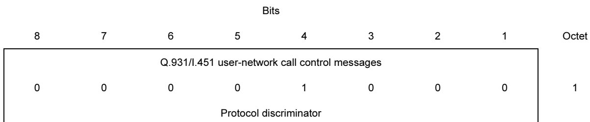
FIGURE 4-2/Q.931
