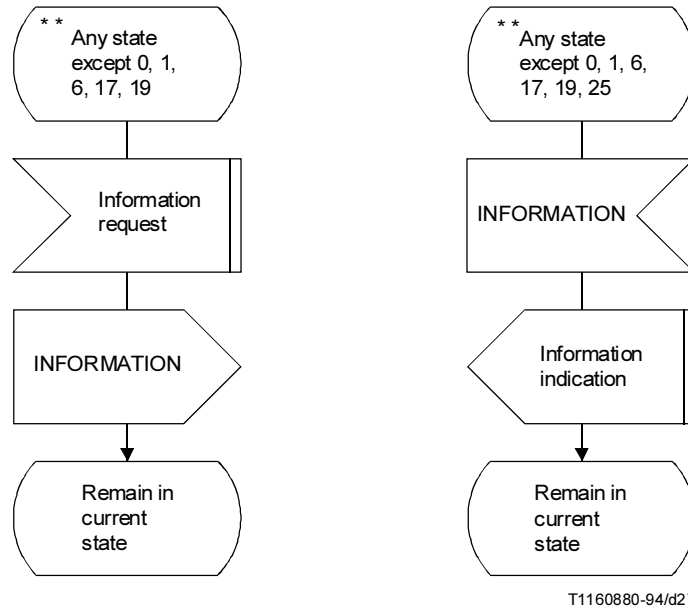
FIGURE A.3/Q.931 (Sheet 18 of 25) Detailed protocol control (user side)
