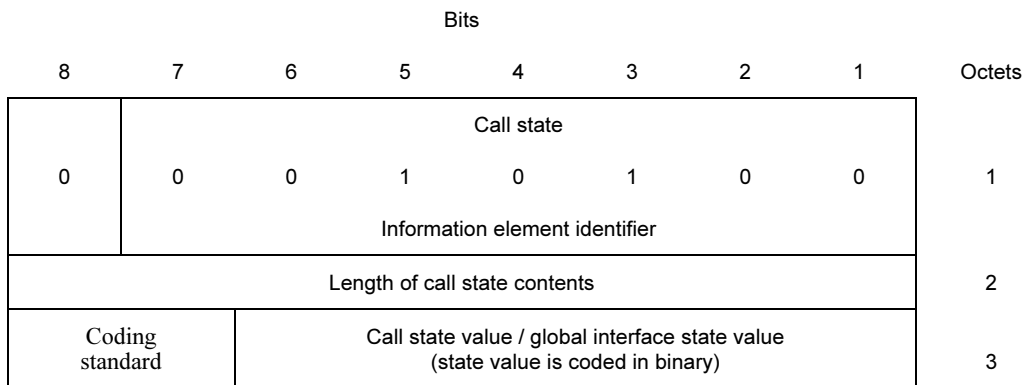
FIGURE 4-13/Q.931
