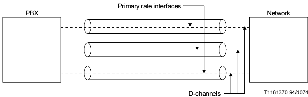
FIGURE F.1/Q.931
