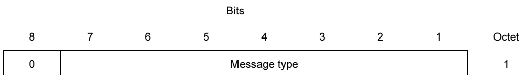
FIGURE 4-6/Q.931
