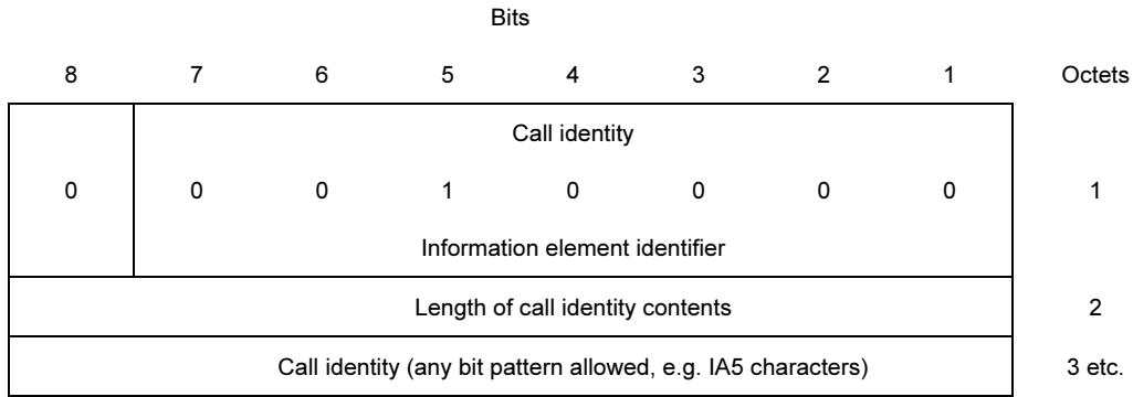
FIGURE 4-12/Q.931
