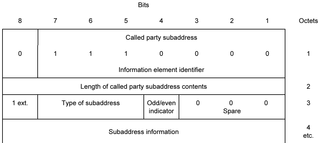
FIGURE 4-15/Q.931
