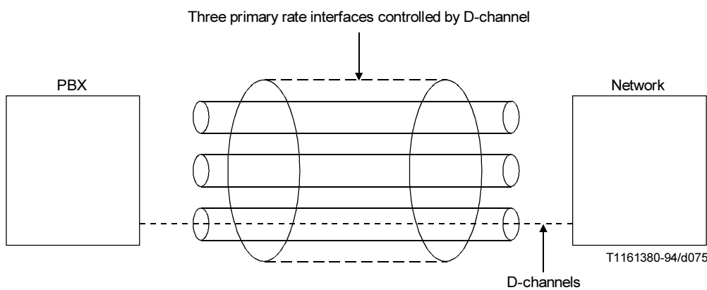
FIGURE F.2/Q.931
