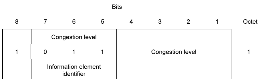
FIGURE 4-20/Q.931
