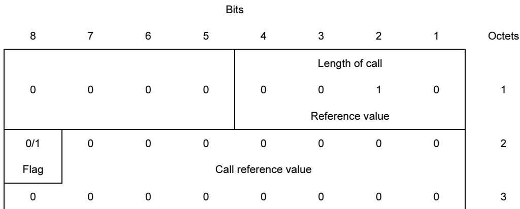
b) Two octet call reference value
