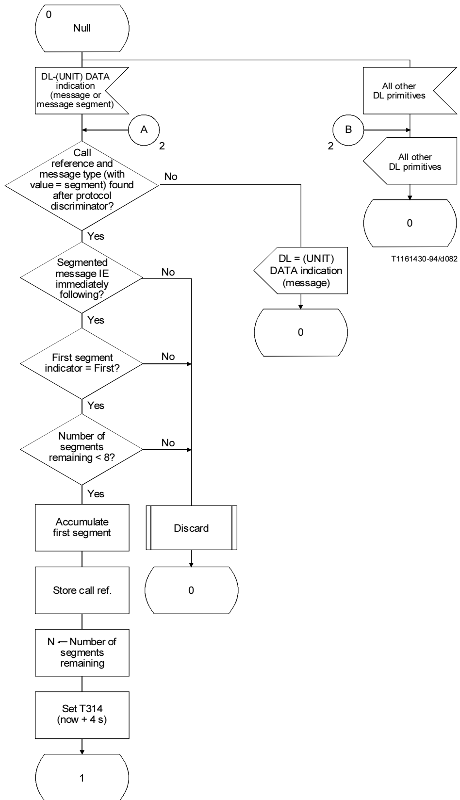
FIGURE H.5/Q.931 (Sheet 1 of 3)
