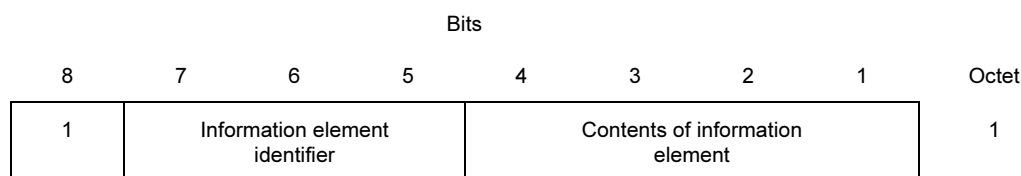
a) Single octet information element format (type 1)
