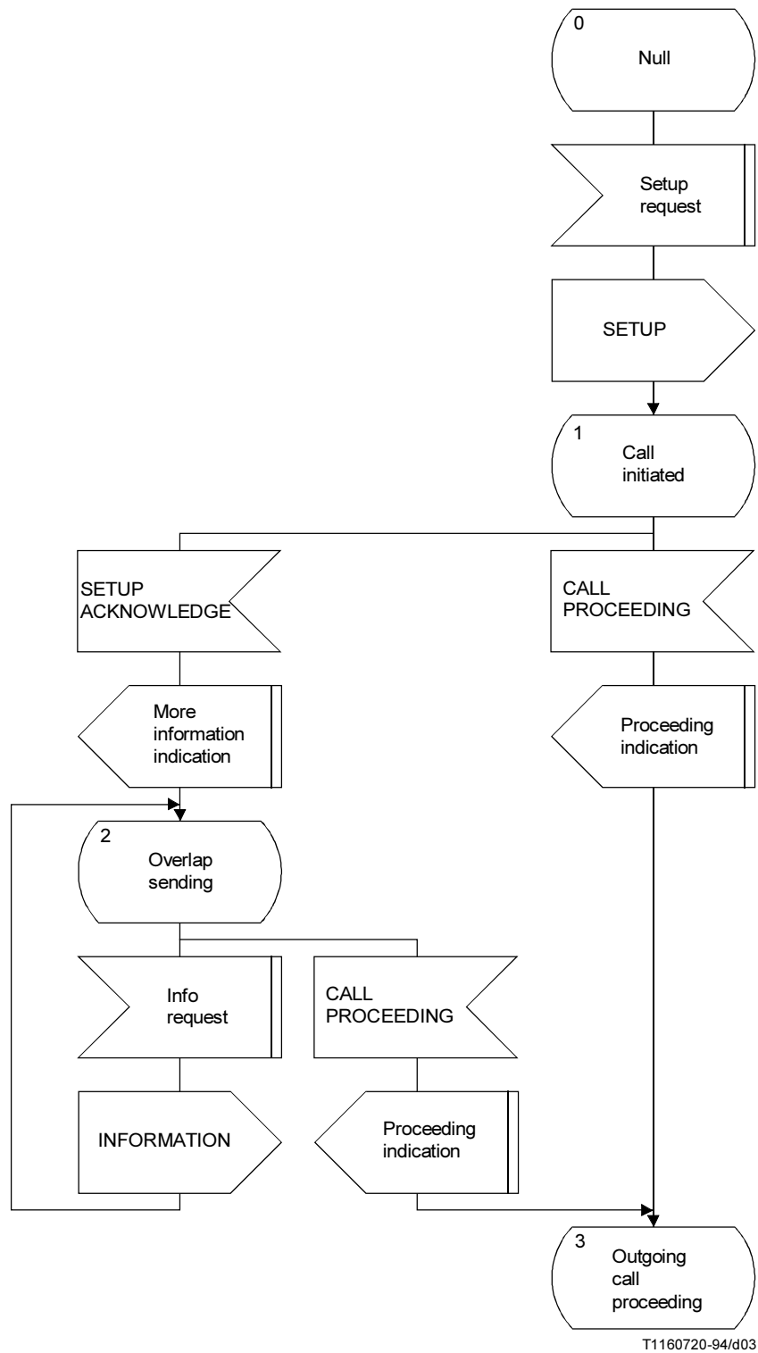
a) Outgoing set-up procedure (1 of 2)
