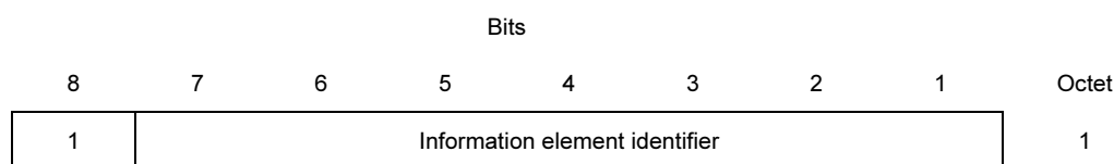
b) Single octet information element format (type 2)
