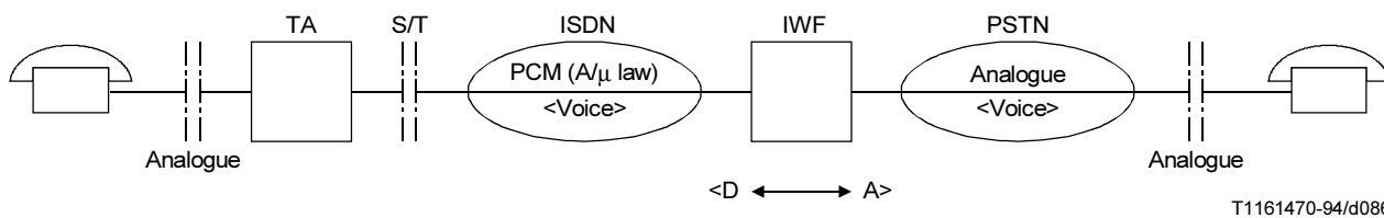
FIGURE I.2/Q.931
