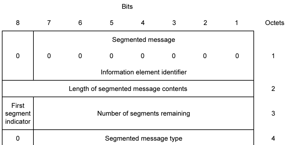
FIGURE 4-32/Q.931
