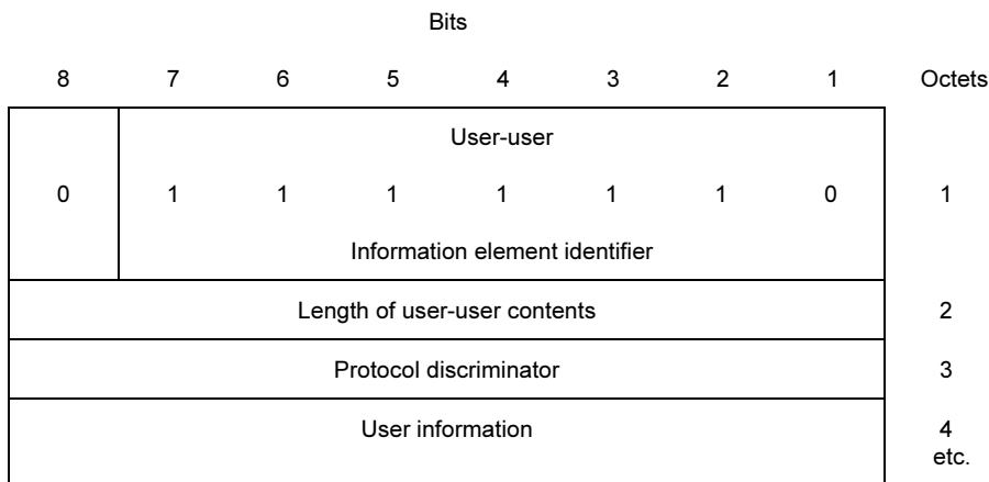
FIGURE 4-36/Q.931
