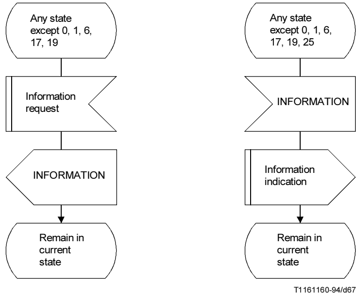
FIGURE A.6/Q.931 (Sheet 21 of 27) Detailed protocol control (network side) point-point
