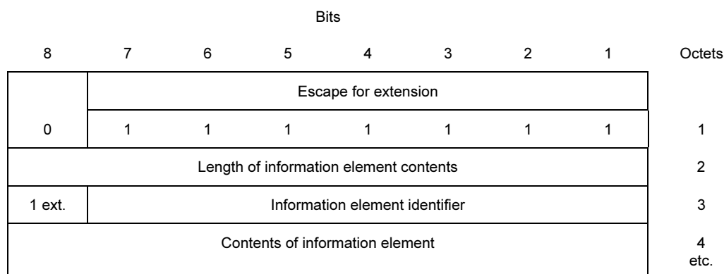
FIGURE 4-8/Q.931
