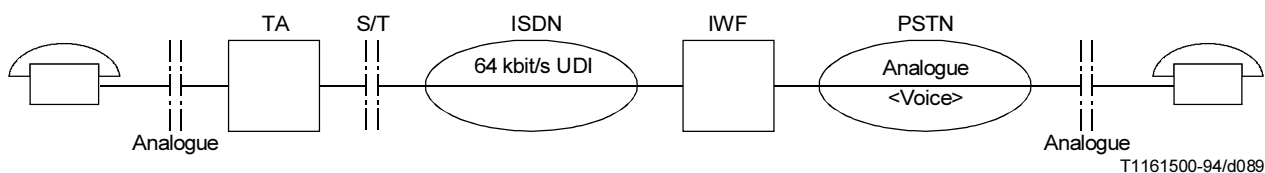
FIGURE I.5/Q.931
