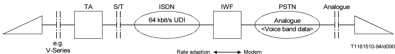
FIGURE I.6/Q.931
