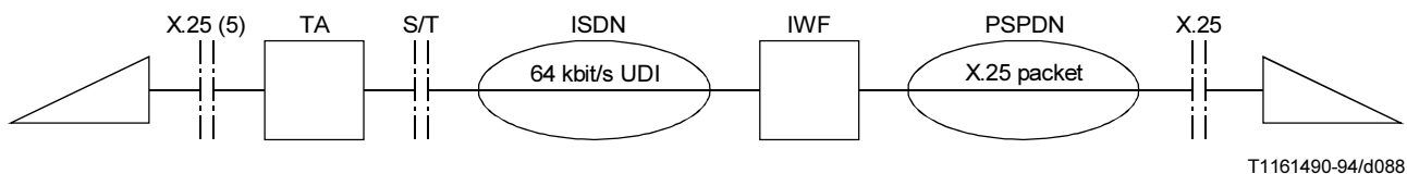
FIGURE I.4/Q.931
