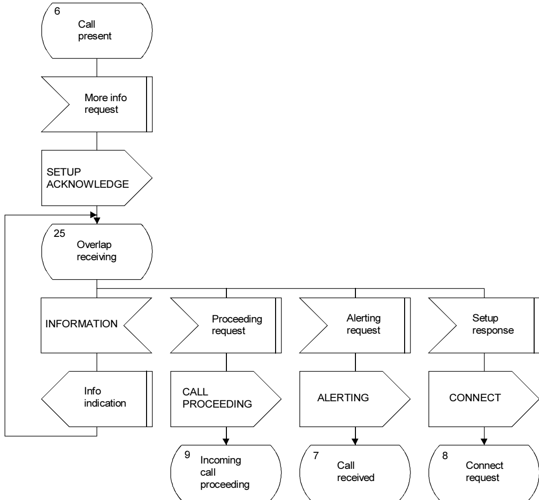
c) Overlap receiving procedure
