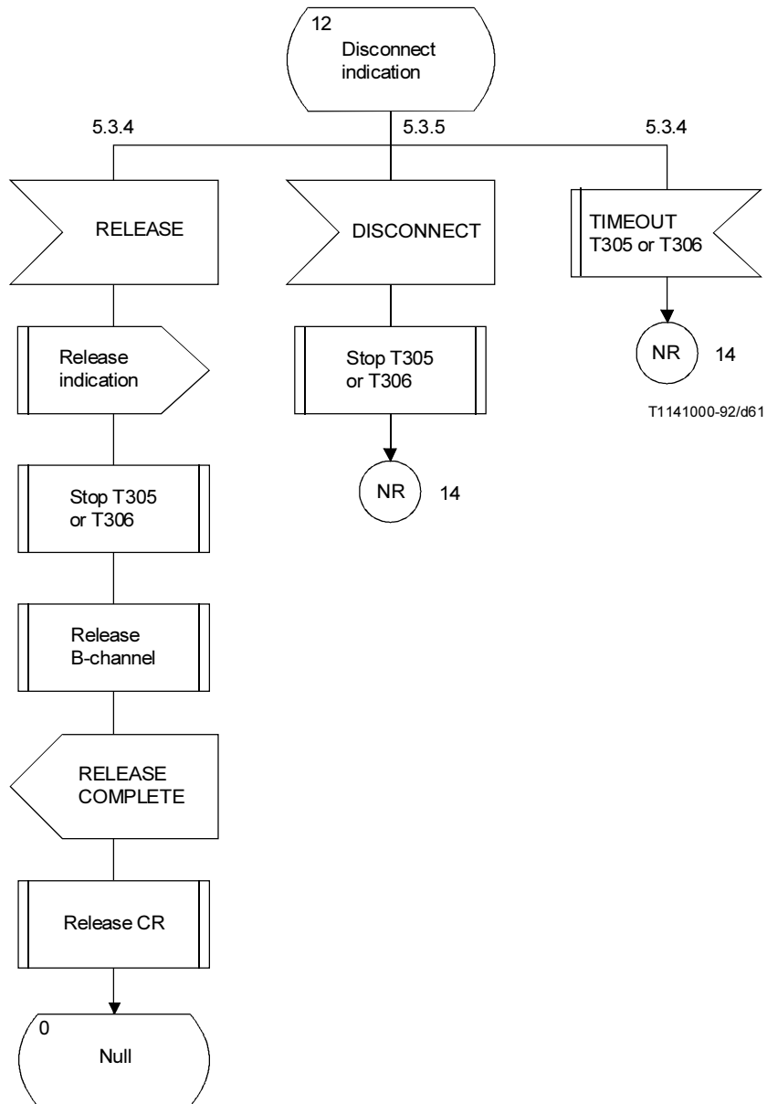
FIGURE A.6/Q.931 (Sheet 15 of 27)
