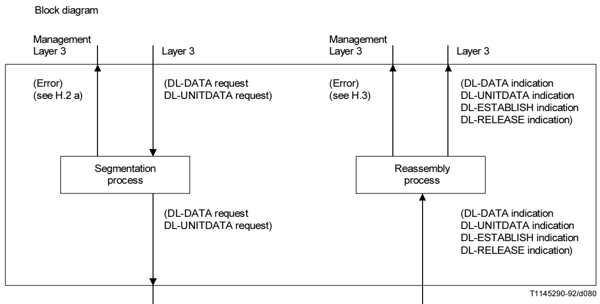
FIGURE H.3/Q.931
