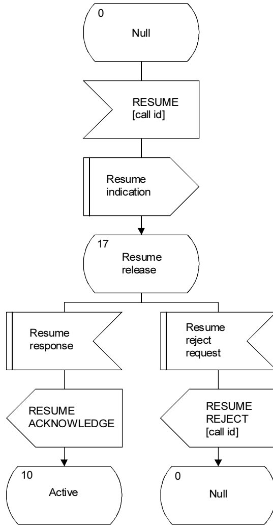
d) Resume procedure
