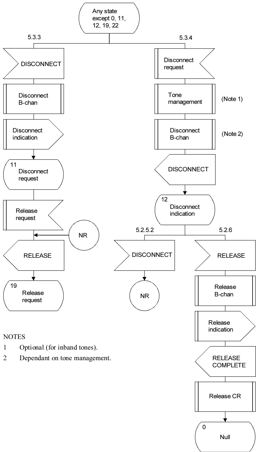
c) Clearing procedure (1 of 2)
