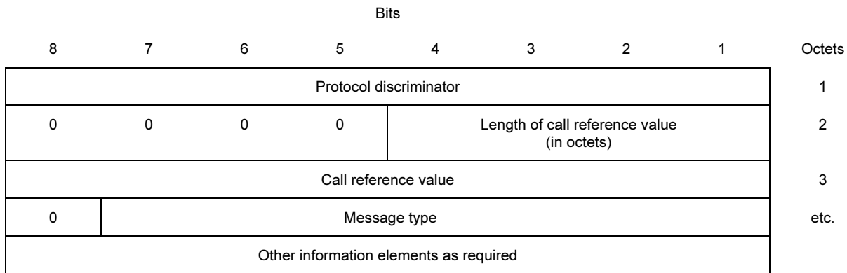
FIGURE 4-1/Q.931
