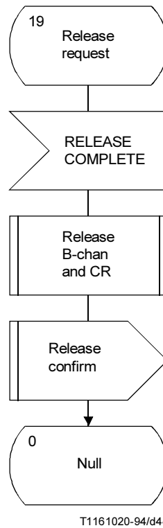
c) Clearing procedure (2 of 2)
