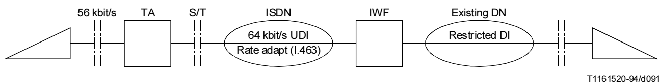
FIGURE I.7/Q.931
