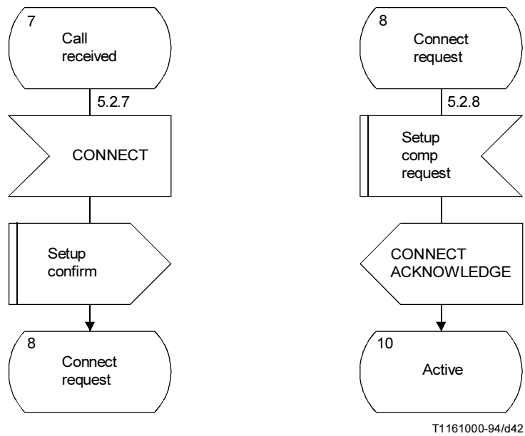
b) Incoming set-up procedure (2 of 2)
