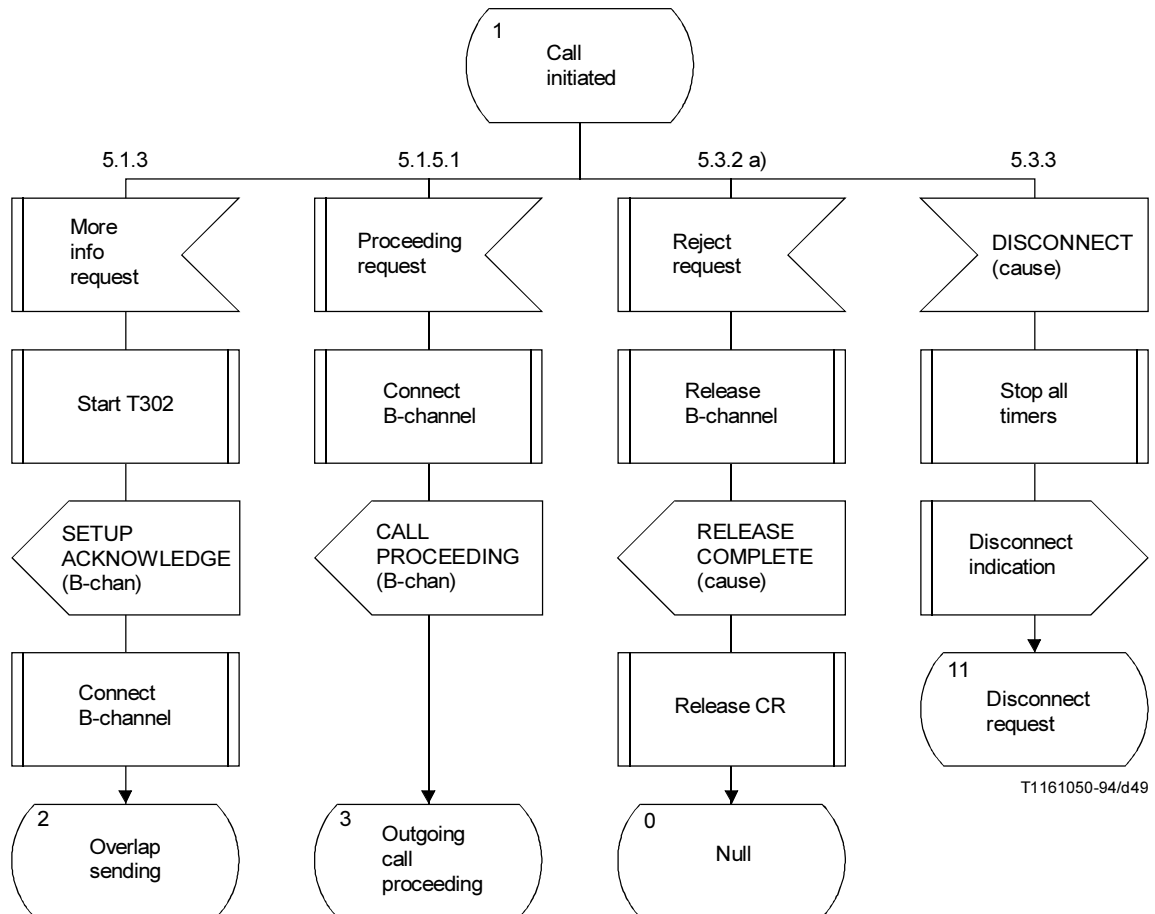
FIGURE A.6/Q.931 (Sheet 3 of 27) Detailed protocol control (network side) point-point
