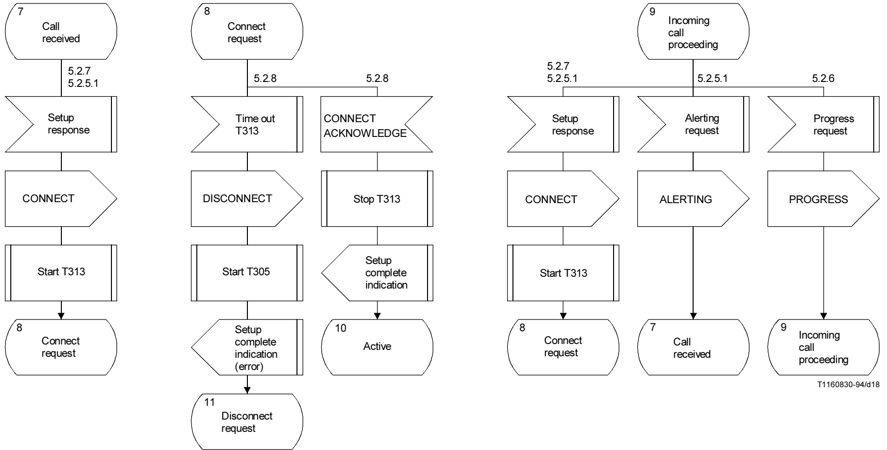
FIGURE A.3/Q.931 (Sheet 9 of 25) Detailed protocol control (user side)
