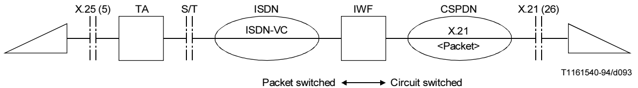
FIGURE I.9/Q.931
