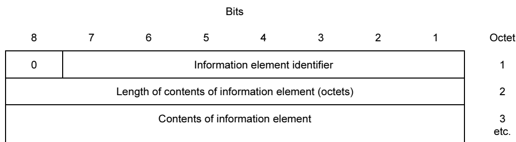
c) Variable length information element format
