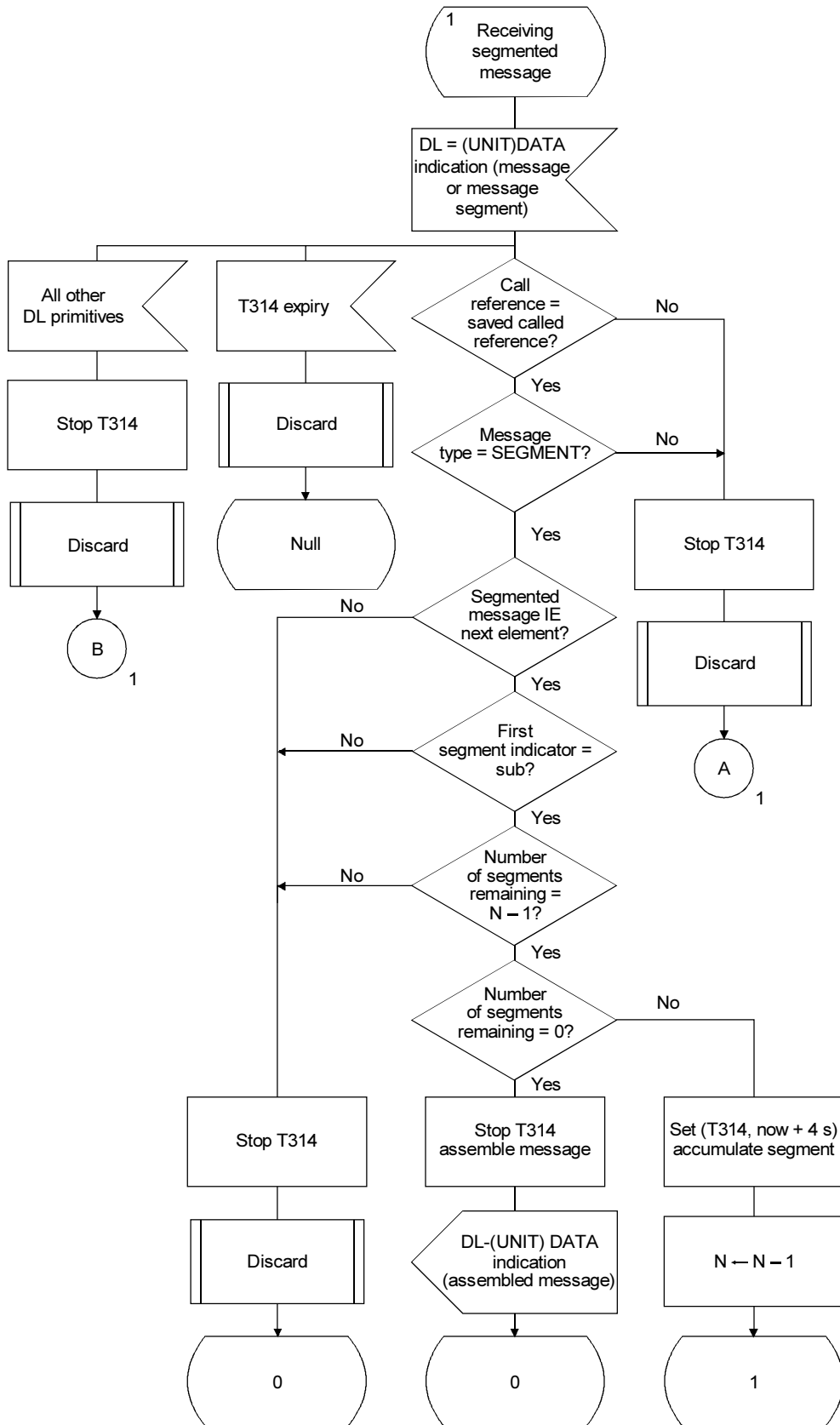
FIGURE H.5/Q.931 (Sheet 2 of 3)
