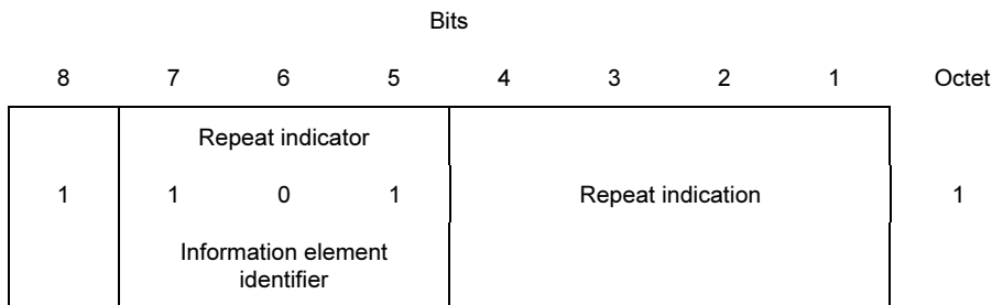
FIGURE 4-30/Q.931
