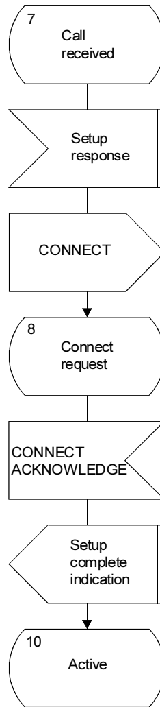
b) Incoming set-up procedure (2 of 2)
