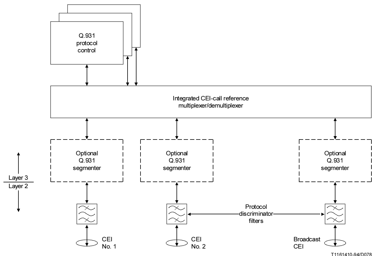
FIGURE H.1/Q.931
