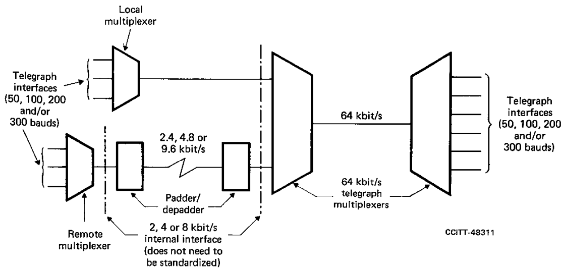
FIGURE 1/R.111
