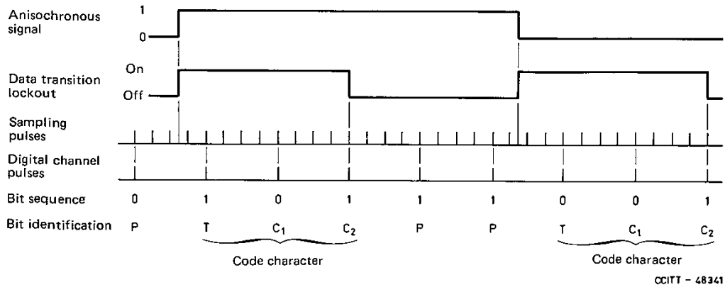
FIGURE A-1/R.111 Transition coding process
