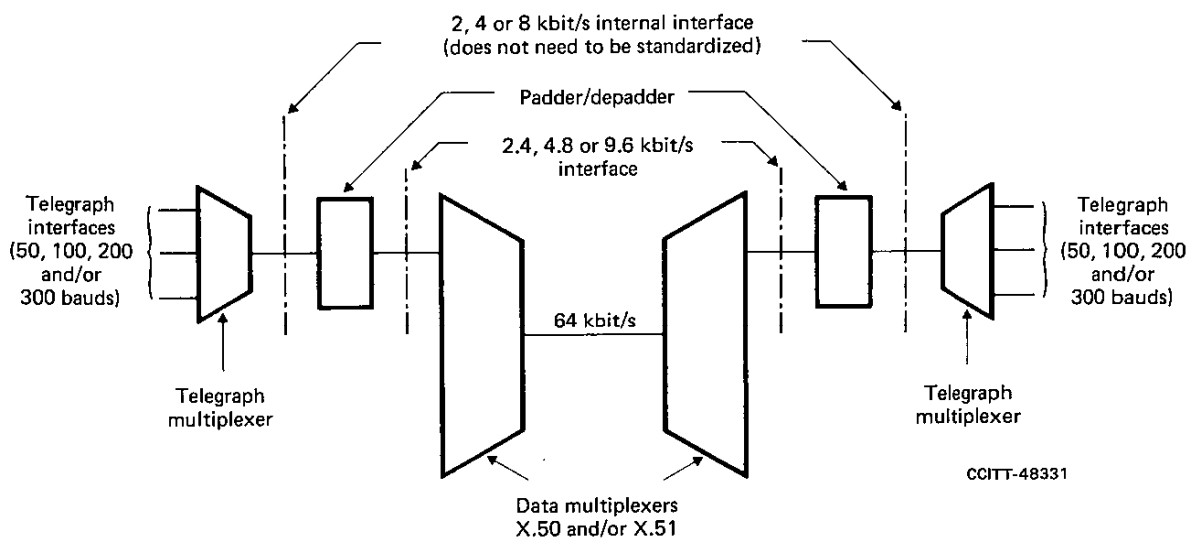
FIGURE 3/R.111
