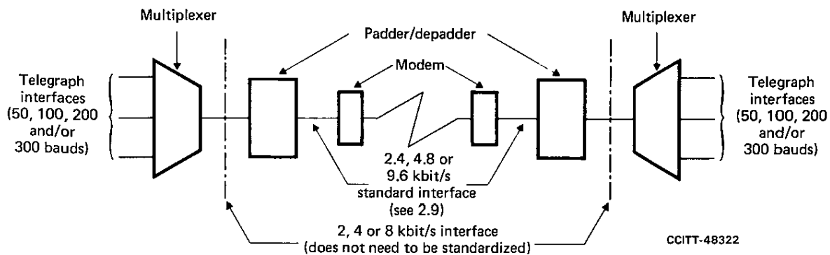
FIGURE 2/R.111
