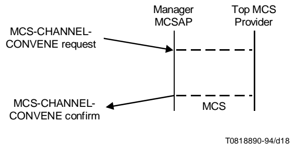
FIGURE 18/T.122 MCS-CHANNEL-CONVENE
