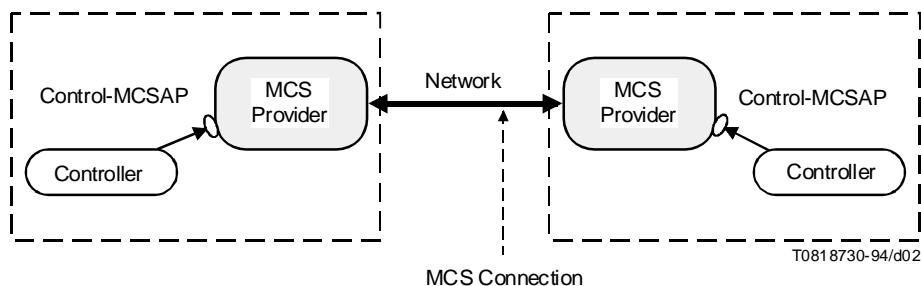
FIGURE 2/T.122 MCS Connection Phase
