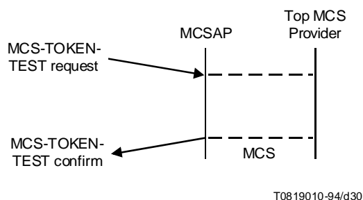
FIGURE 30/T.122 MCS-TOKEN-TEST
