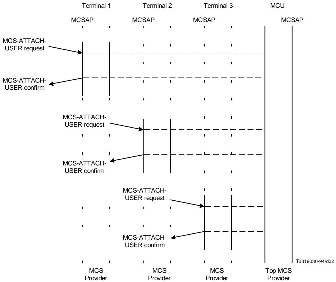
FIGURE 32/T.122 MCS Domain Establishment
