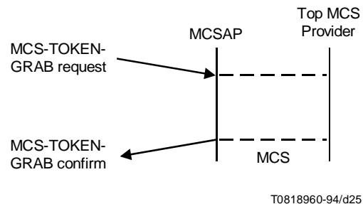
FIGURE 25/T.122 MCS-TOKEN-GRAB
