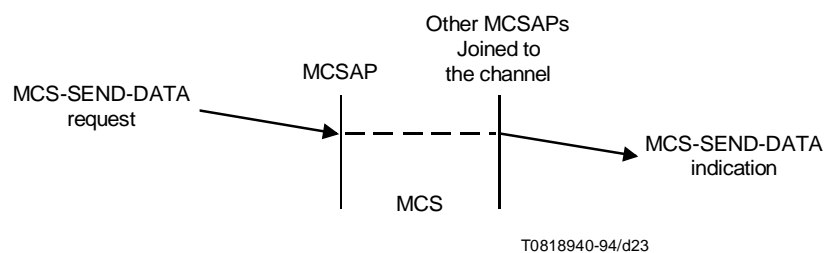
FIGURE 23/T.122 MCS-SEND-DATA
