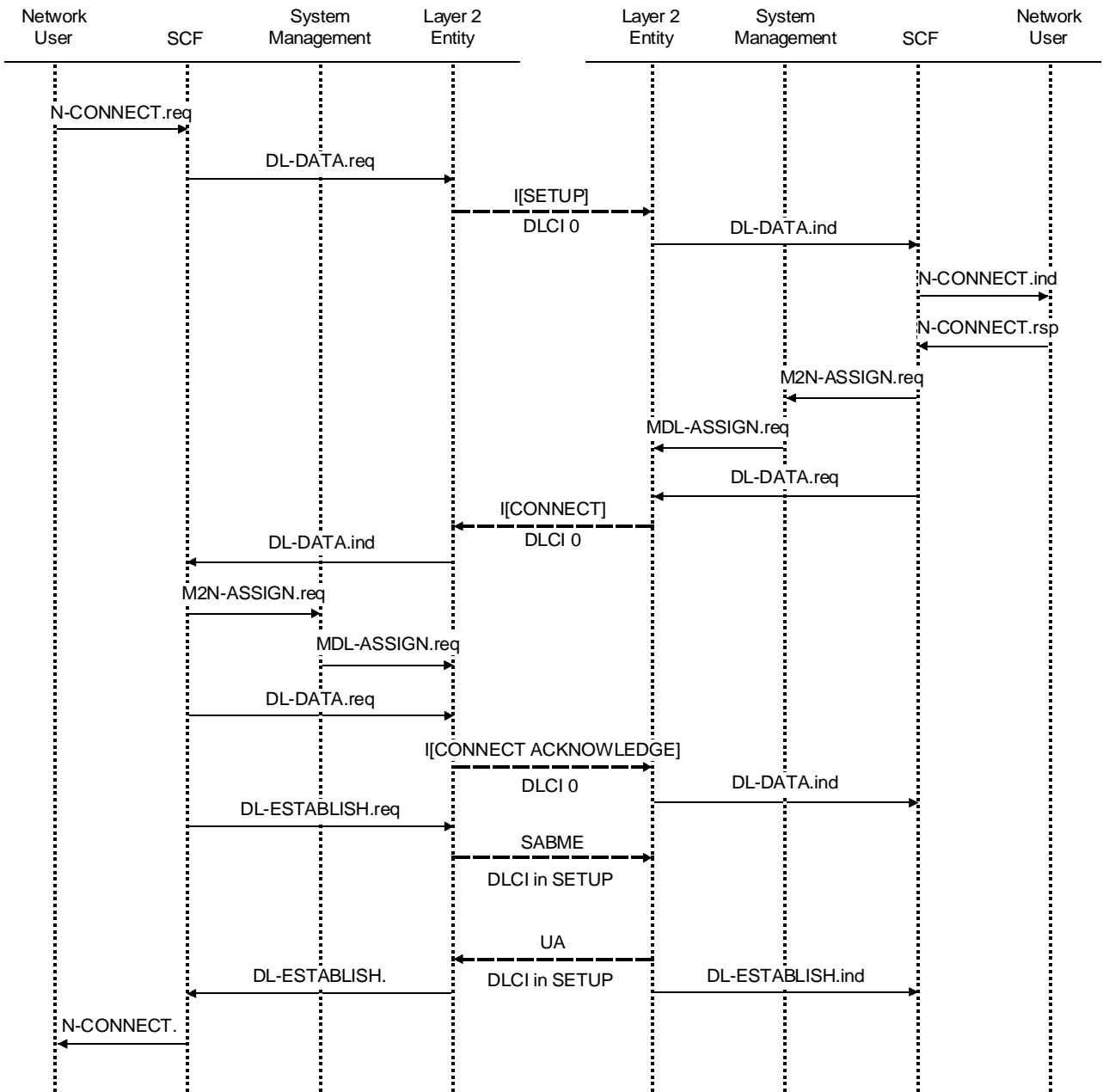
FIGURE 15/T.123 Sequence of actions for N-CONNECT
