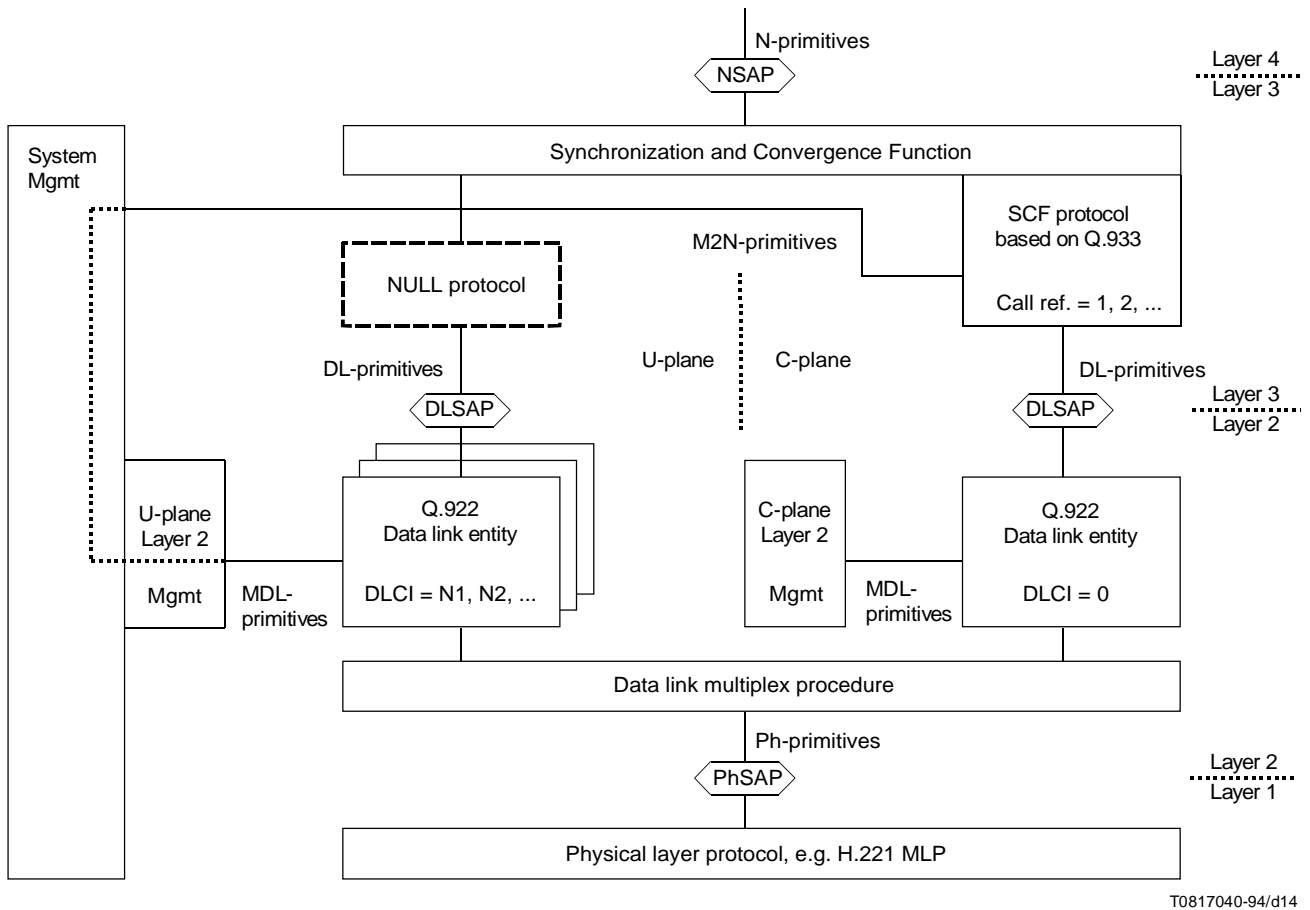
FIGURE 14/T.123 Architectural model of the SCF
