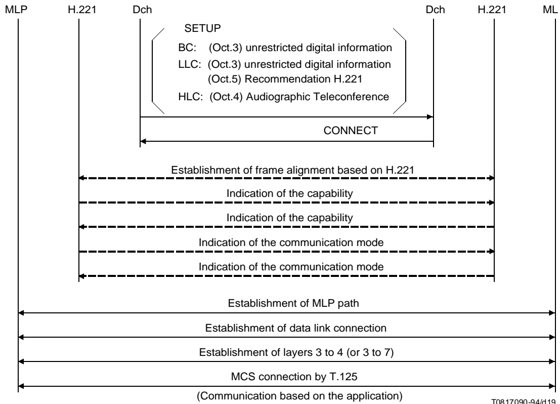
FIGURE I.1/T.123 Communication establishment sequence for AGC terminals
