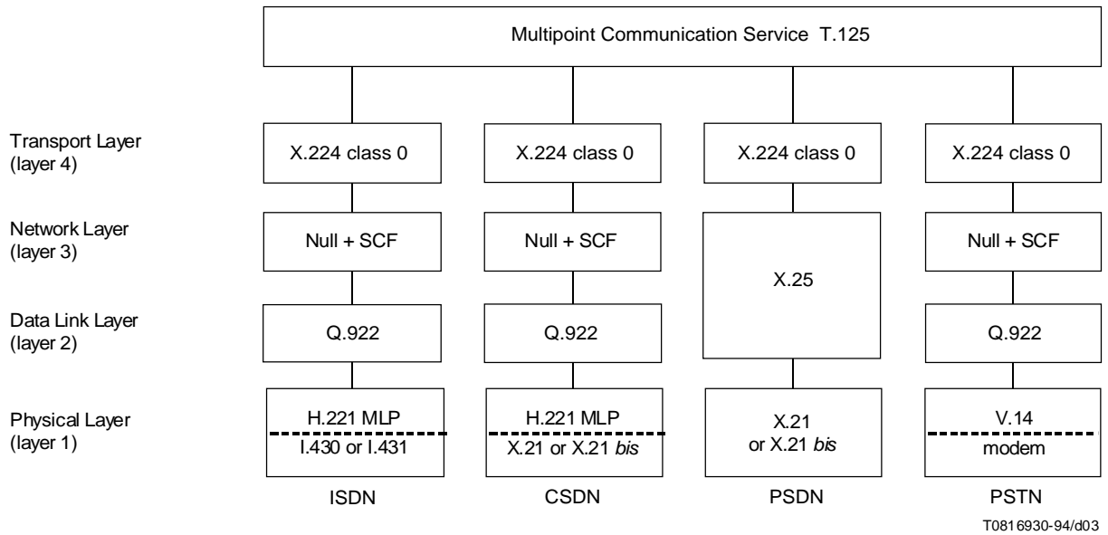
FIGURE 3/T.123 Basic mode profiles general structure
