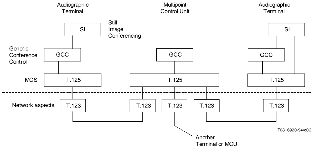
FIGURE 2/T.123 Framework of the AGC protocol suite
