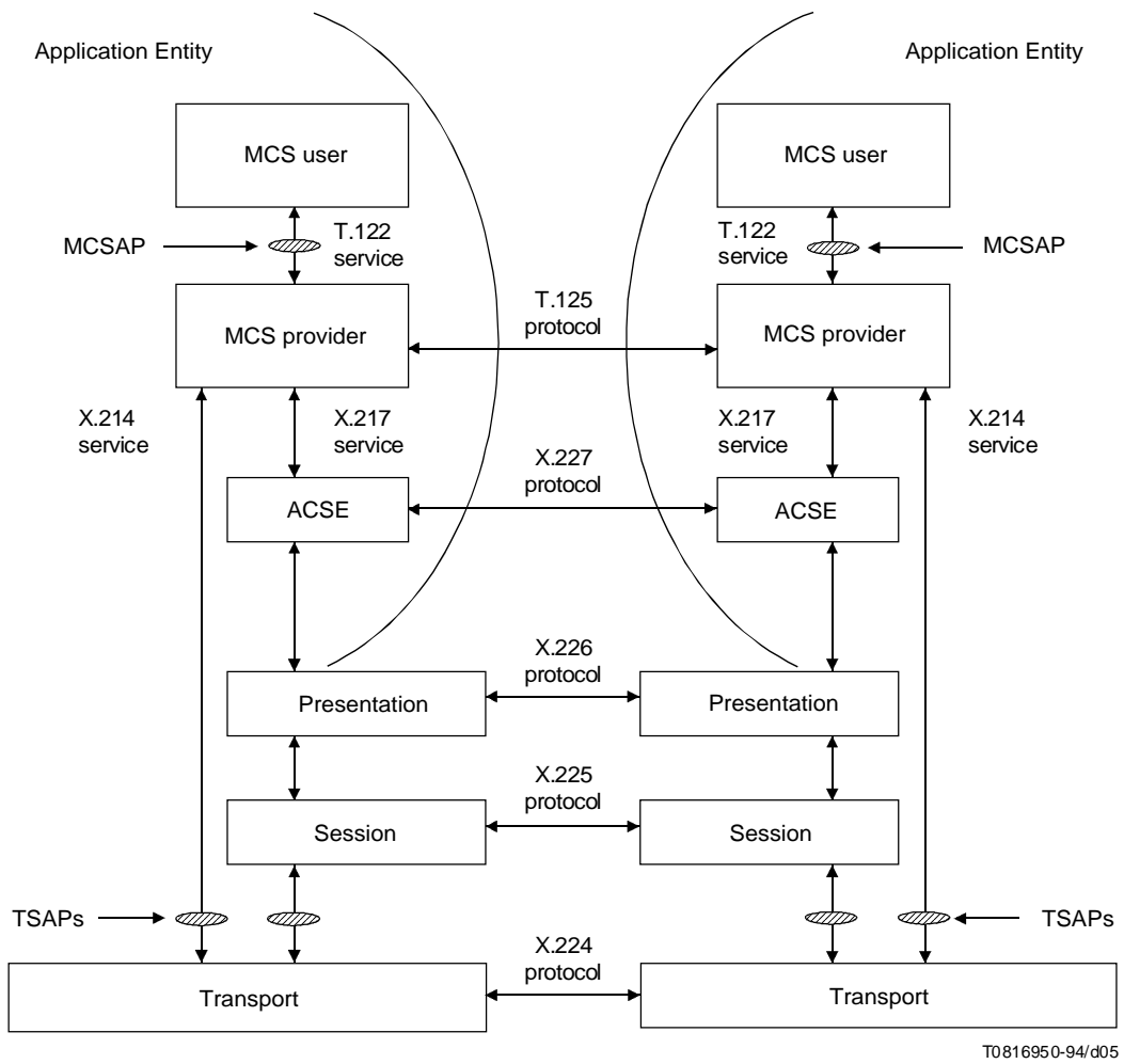
FIGURE 5/T.123 Location of an MCS provider in the OSI reference model
