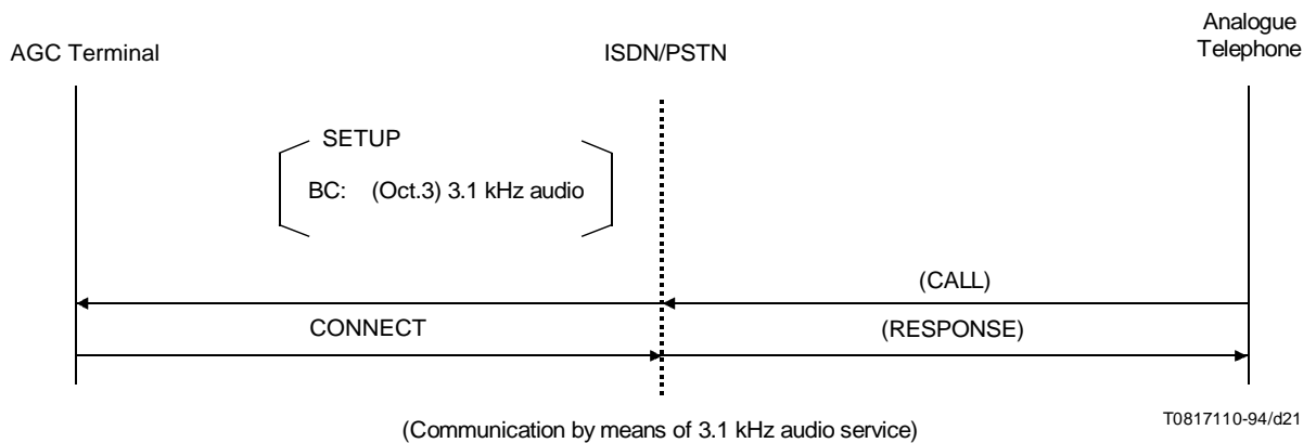
2) Call from Analogue Telephone to AGC Terminal
