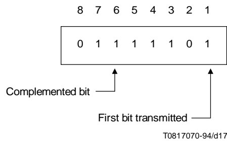
FIGURE 17/T.123 Control escape octet for start-stop transparency
