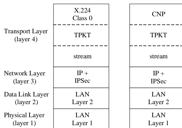
Figure B.12/T.123 – Extended profiles using IPSec for security services
