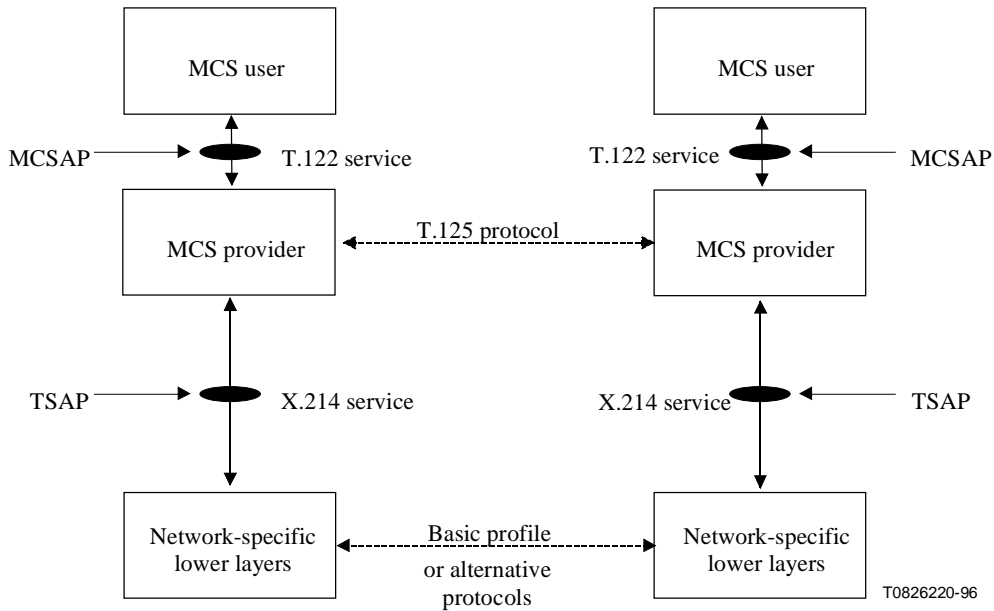
Figure 4/T.123 – Location of an MCS provider in the OSI reference model
