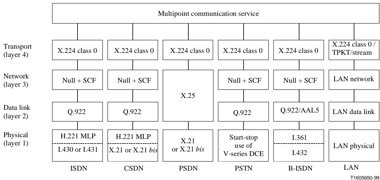
Figure 3/T.123 – Basic profiles general structure
