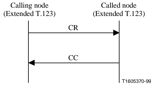
Figure B.6/T.123 – Call between extended T.123 nodes – Existing network connection selected
