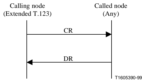
Figure B.8/T.123 – Call refusal
