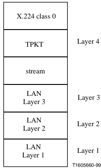
Figure 10/T.123 – LAN basic profile
