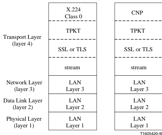
Figure B.11/T.123 – Extended profiles using SSL or TLS for security services
