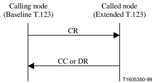
Figure B.4/T.123 – Call from baseline T.123 to extended T.123
