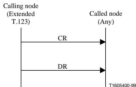
Figure B.9/T.123 – Abandoned call attempt
