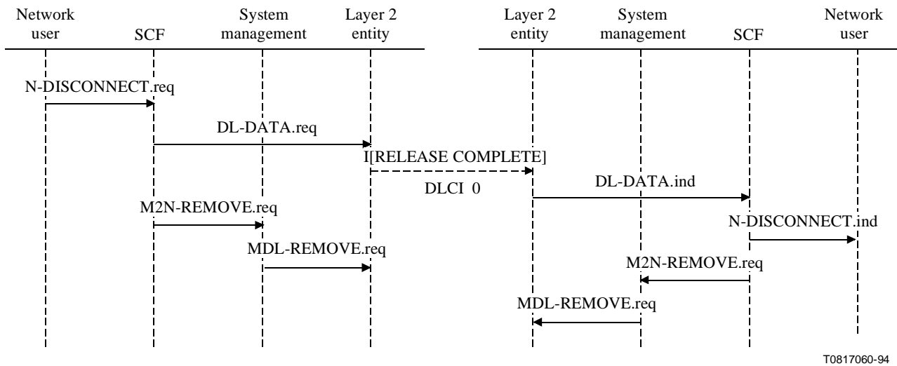
Figure 14/T.123 – Sequence of actions for N-DISCONNECT
