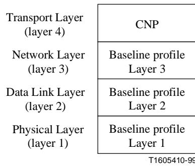
Figure B.10/T.123 – Extended profile using CNP for reliable transport service
