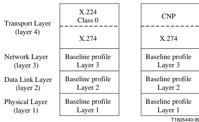
Figure B.13/T.123 – Extended profiles using X.274 for security services
