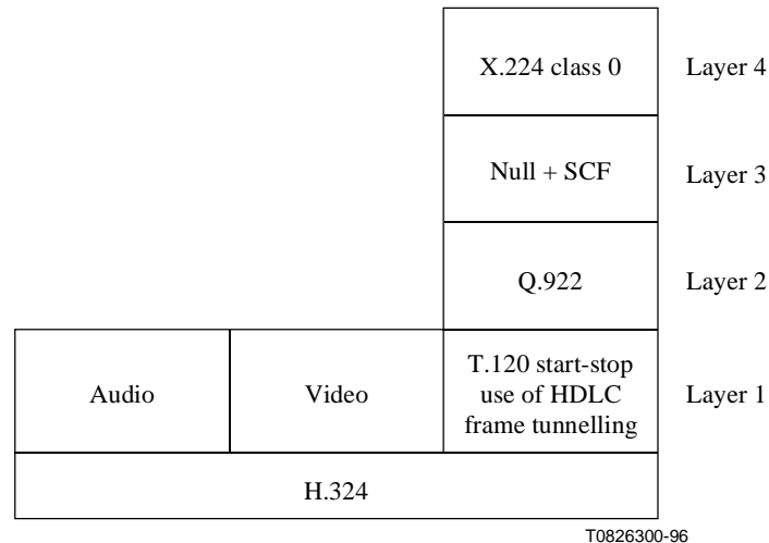
Figure 19/T.123 – Alternative profile for PSTN based on Recommendation H.324
