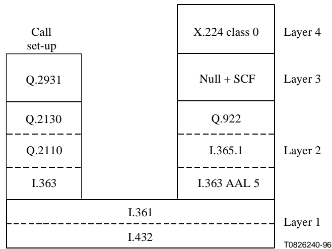
Figure 9/T.123 – B-ISDN basic profile
