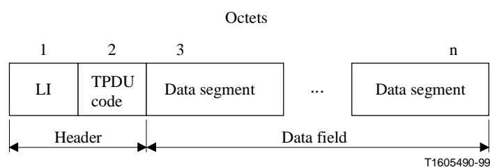
Figure B.19/T.123 – CNP Data TPDU structure
