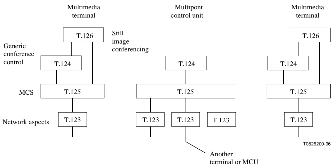
Figure 2/T.123 – Framework of the T.120 protocol suite
