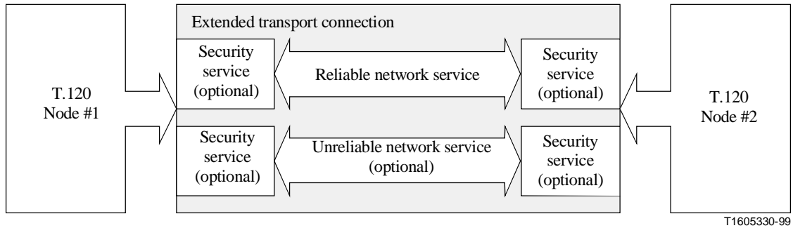
Figure B.2/T.123 – Extended transport connection model
