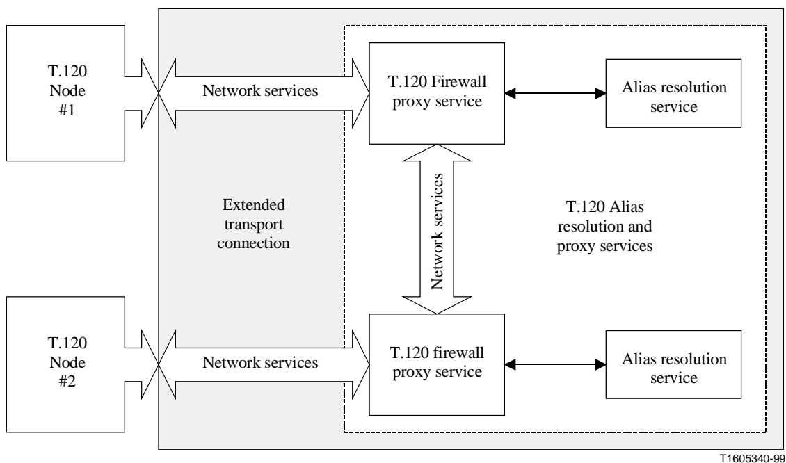
Figure B.3/T.123 – Example of extended transport connection via T.120 proxy
