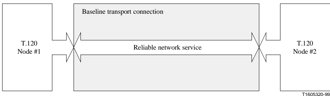
Figure B.1/T.123 – Baseline transport connection model
