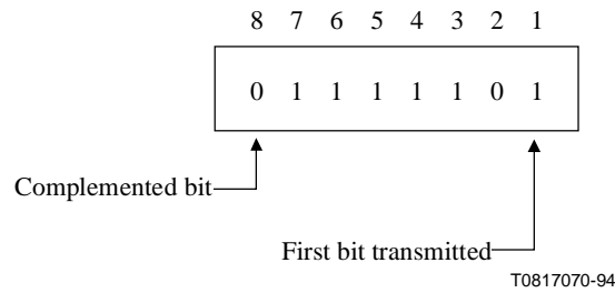
Figure 15/T.123 – Control escape octet for start-stop transparency
