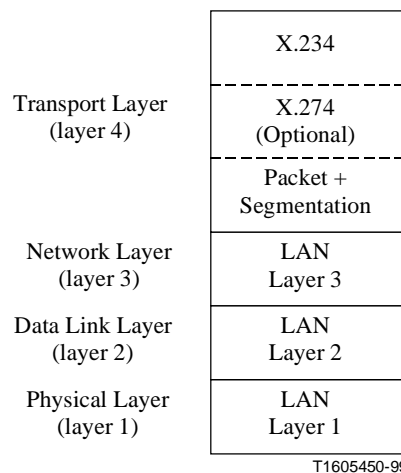
Figure B.15/T.123 – Unreliable LAN profile
