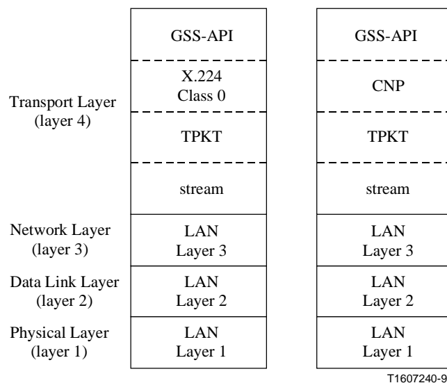
Figure B.14/T.123 – Extended profiles using GSS-API for security services
