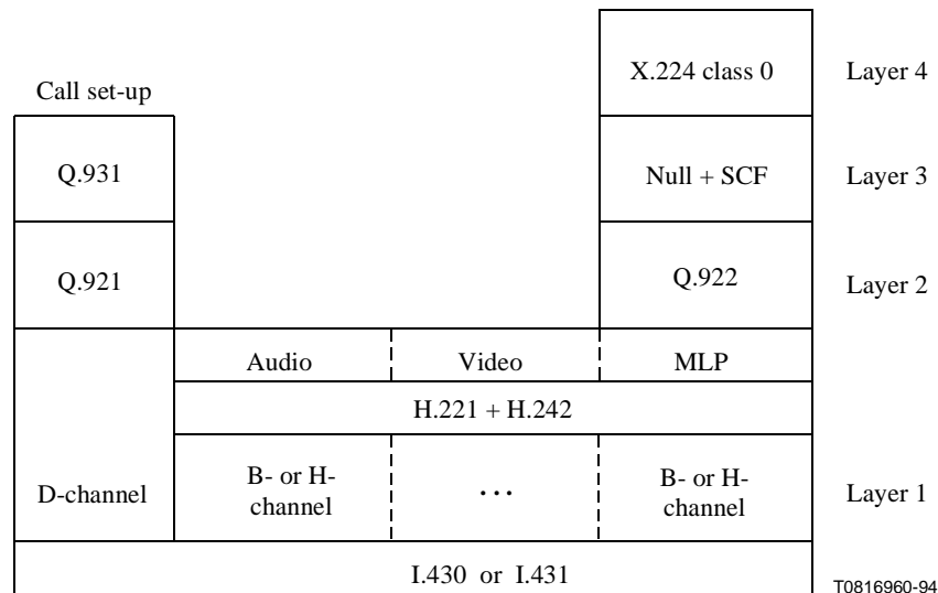
Figure 5/T.123 – ISDN basic profile
