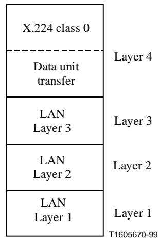
Figure 21/T.123 – Alternative profile for LAN based on data unit transfer
