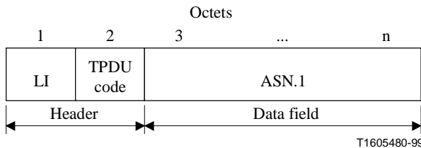
Figure B.18/T.123 – CNP Control TPDU structure
