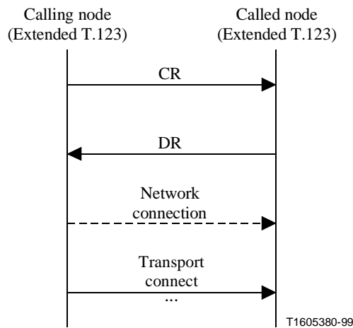
Figure B.7/T.123 – Call between extended T.123 nodes – Reconnection selected
