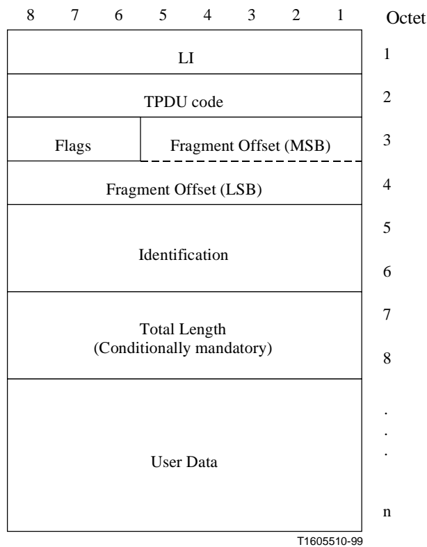
Figure B.21/T.123 – Unreliable SAR TPDU structure
