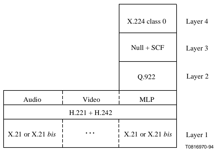
Figure 6/T.123 – CSDN basic profile
