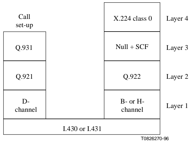
Figure 16/T.123 – Alternative profile for ISDN based on Recommendation Q.922
