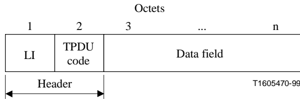
Figure B.17/T.123 – CNP general TPDU structure
