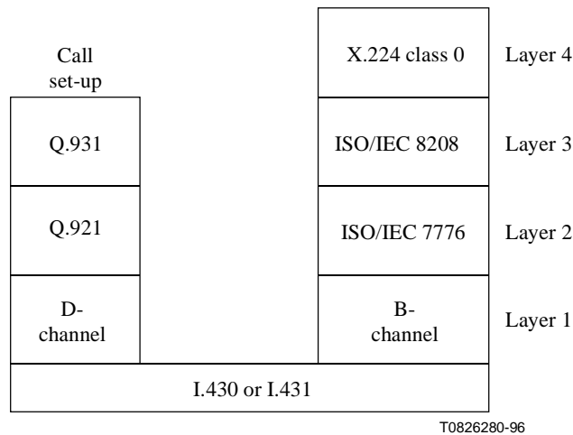
Figure 17/T.123 – Alternative profile for ISDN based on Recommendation T.90
