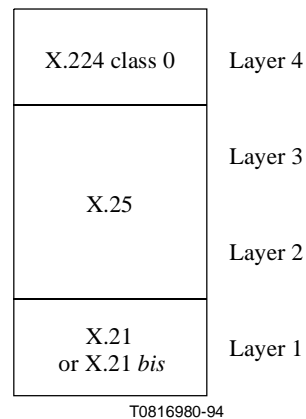
Figure 7/T.123 – PSDN basic profile
