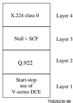
Figure 8/T.123 – PSTN basic profile
