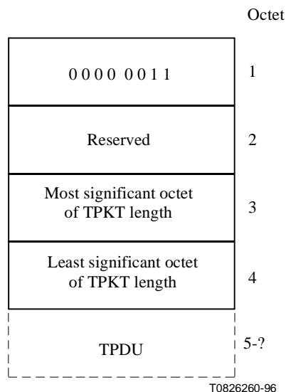
Figure 11/T.123 – Format of the TPKT packet header
