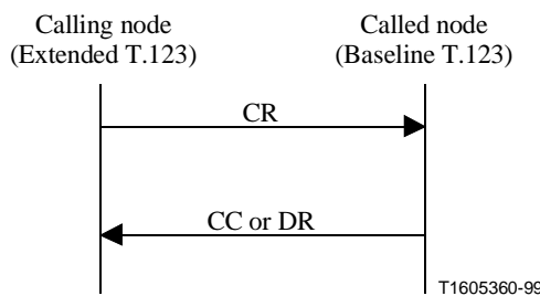
Figure B.5/T.123 – Call from extended T.123 to baseline T.123
