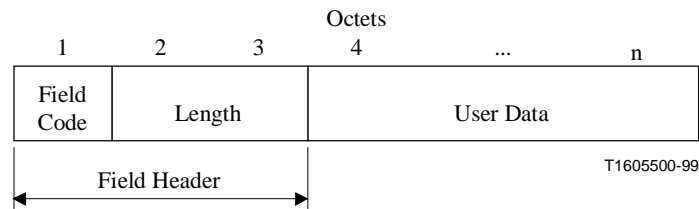
Figure B.20/T.123 – Data Segment structure
