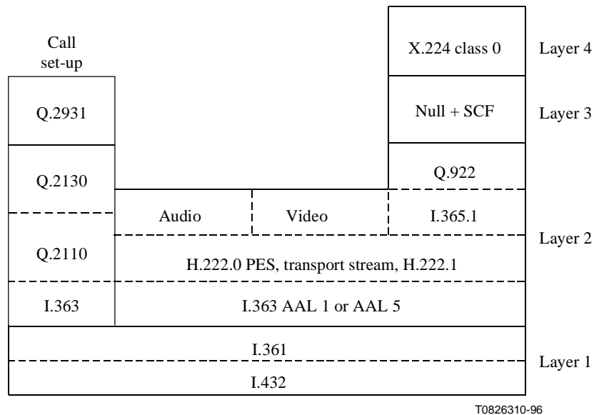
Figure 20/T.123 – Alternative profile for B-ISDN based on Recommendation H.222
