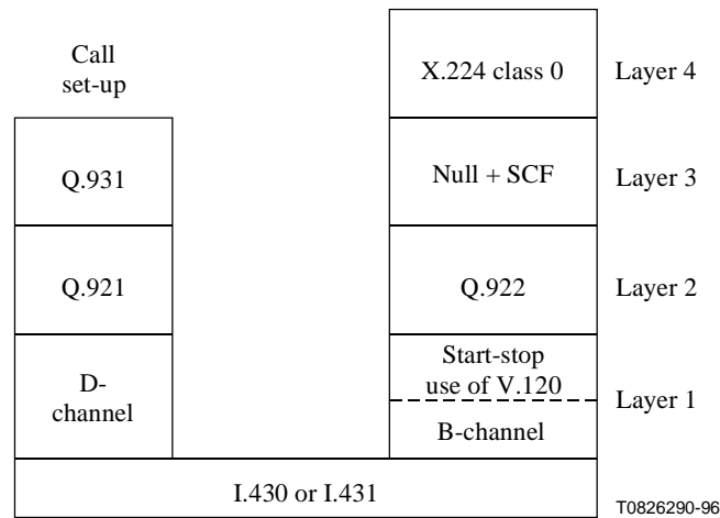
Figure 18/T.123 – Alternative profile for ISDN based on Recommendation V.120
