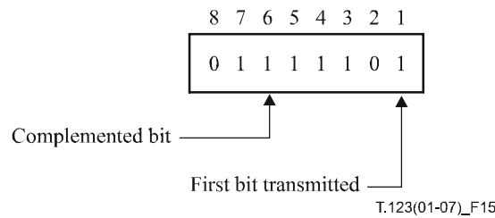
Figure 15 – Control escape octet for start-stop transparency
