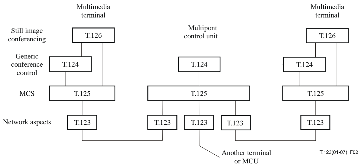
Figure 2 – Framework of the T.120 protocol suite
