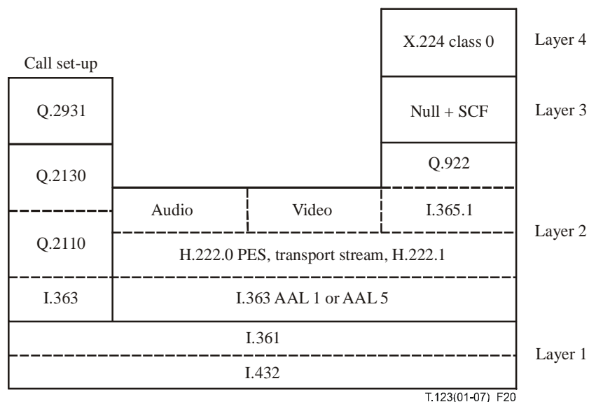
Figure 20 – Alternative profile for B-ISDN based on [ITU-T H.222]
