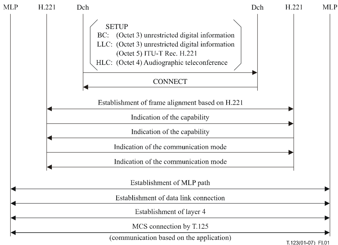
Figure I.1 – Communication establishment sequence for MMC terminals
