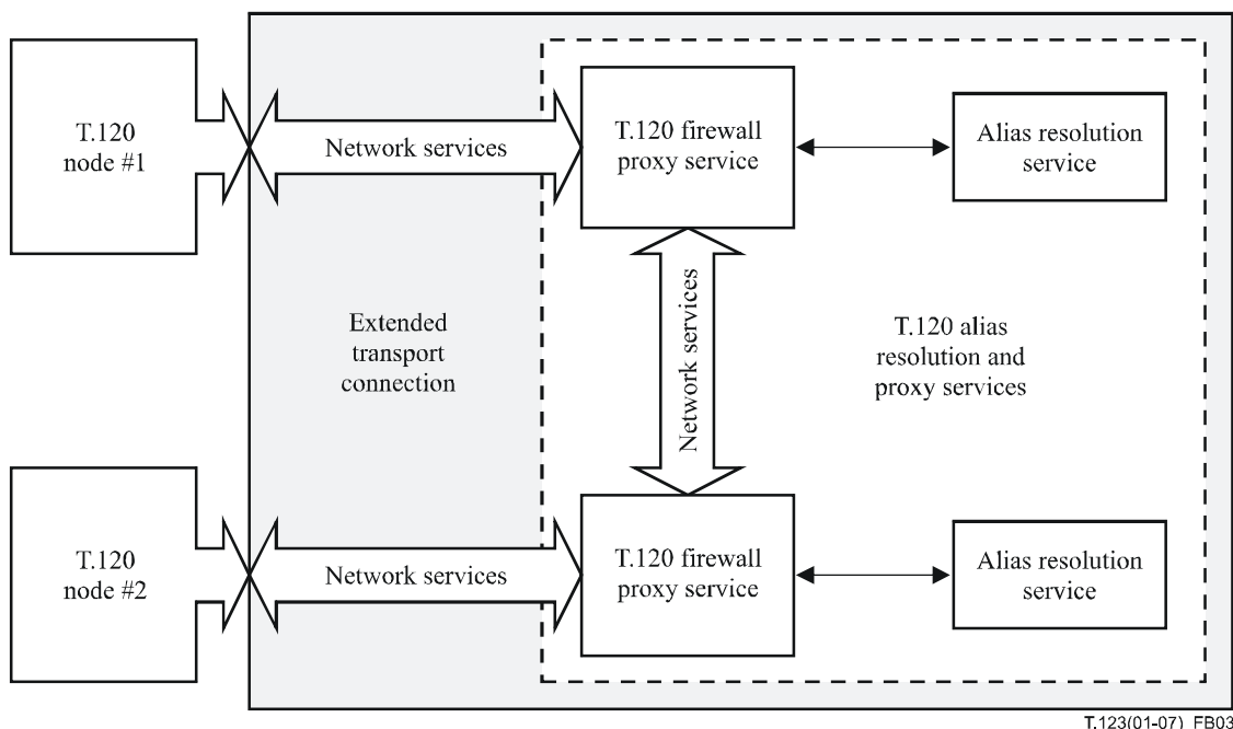
Figure B.3 – Example of extended transport connection via T.120 proxy
