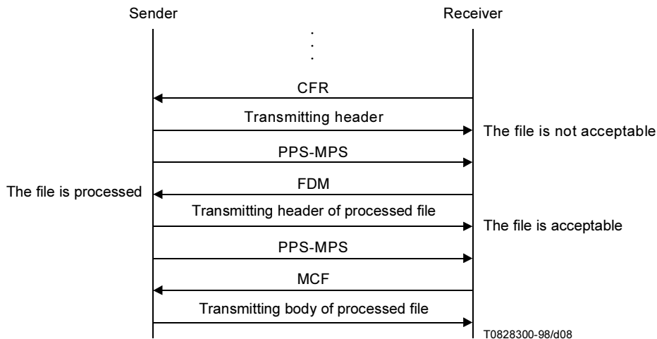
Figure V.5/T.30 – Transmitted file processed on a sender
