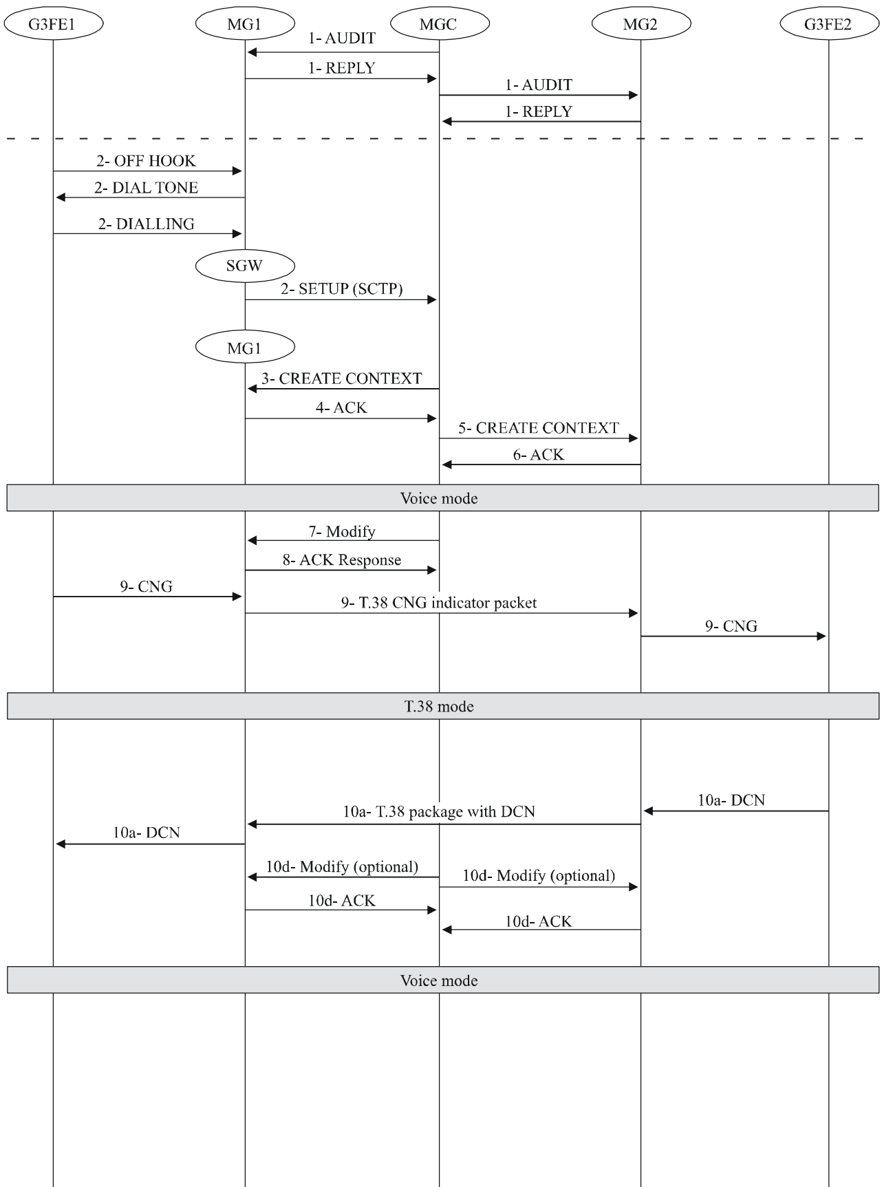
Figure III.3 – Voice to fax call setup with ITU-T H.248 endpoints that support autonomous transition between VoIP and FoIP
