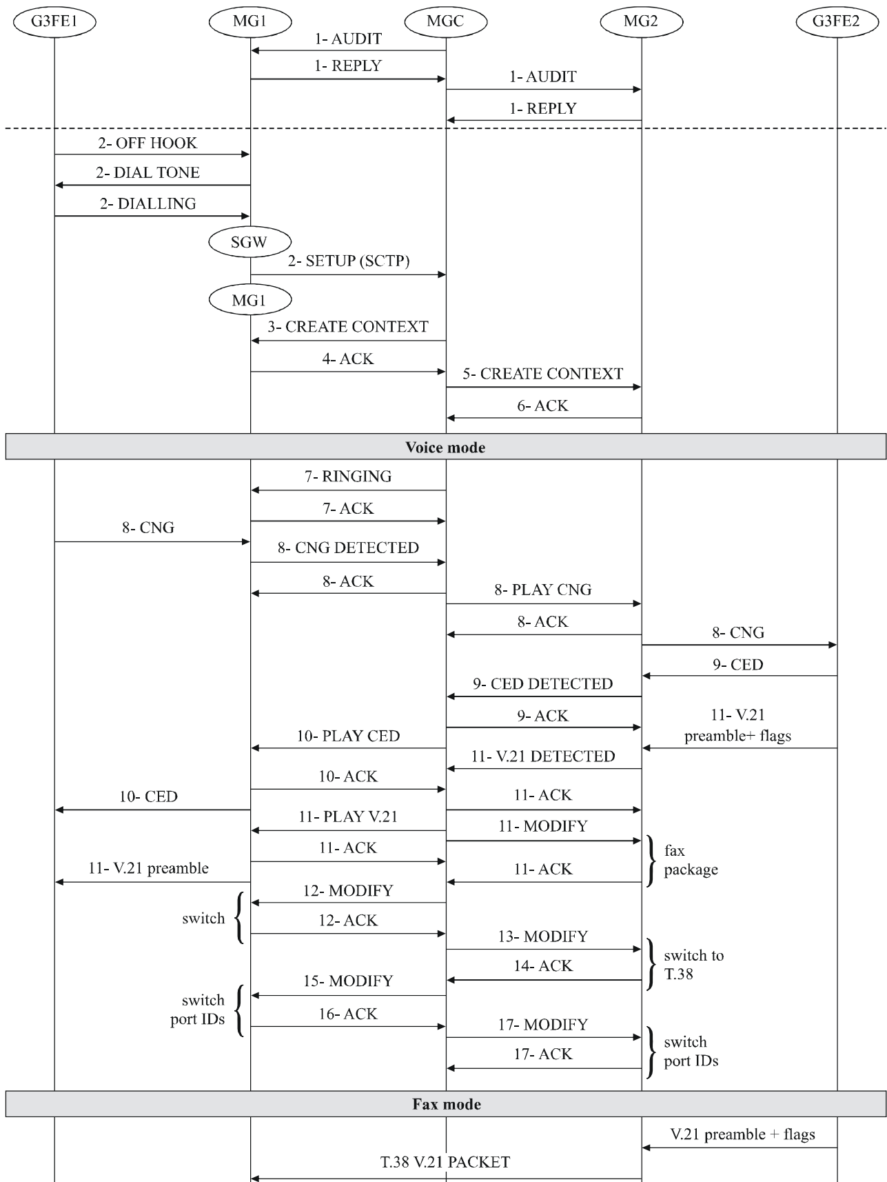
Figure III.1 – Voice to fax call setup with ITU-T H.248 endpoints
