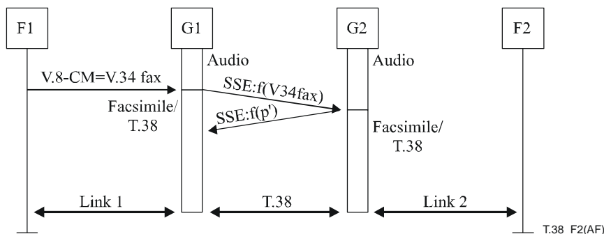
Figure F.2 – ITU-T T.38 FoIP (MoIP transition to ITU-T V.34 fax)
