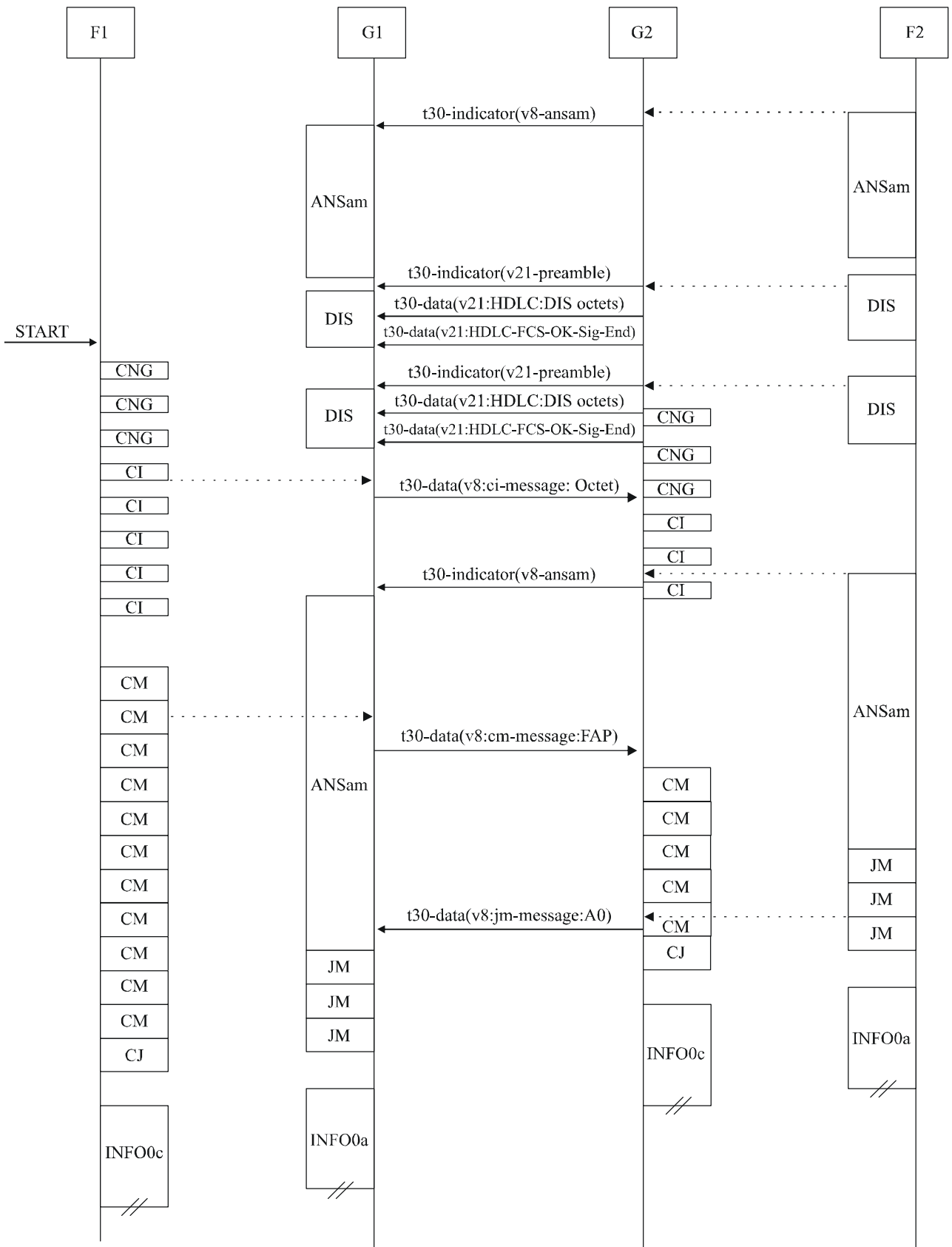
Figure IV.10 – Manual Transmit (DIS has bit 6 set to 1 to indicate ITU-T V.8 capability)
