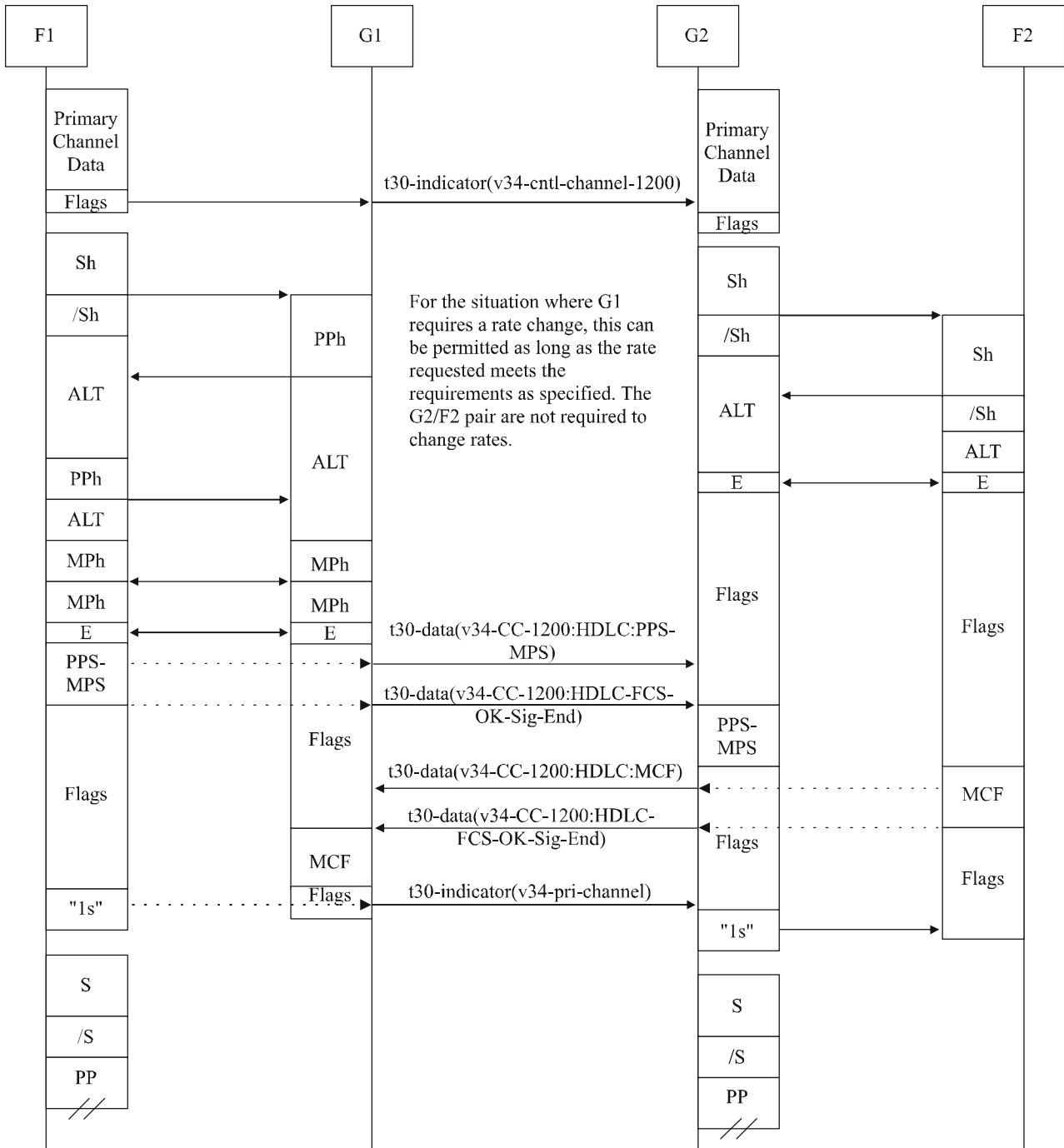
Figure IV.8 – Data rate change sequence when emitting gateway initiates retraining
