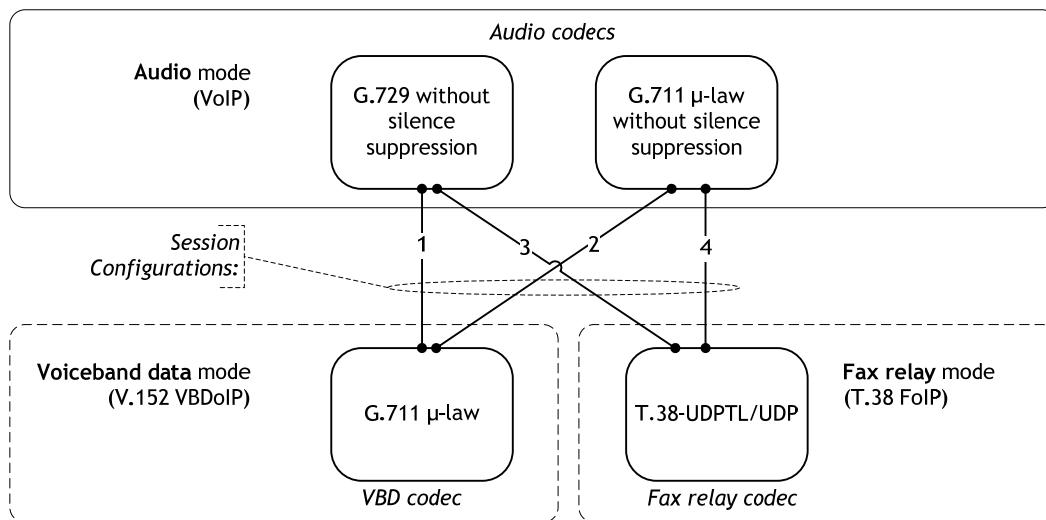
Figure D.6 – Potential session configurations offered in example 5
