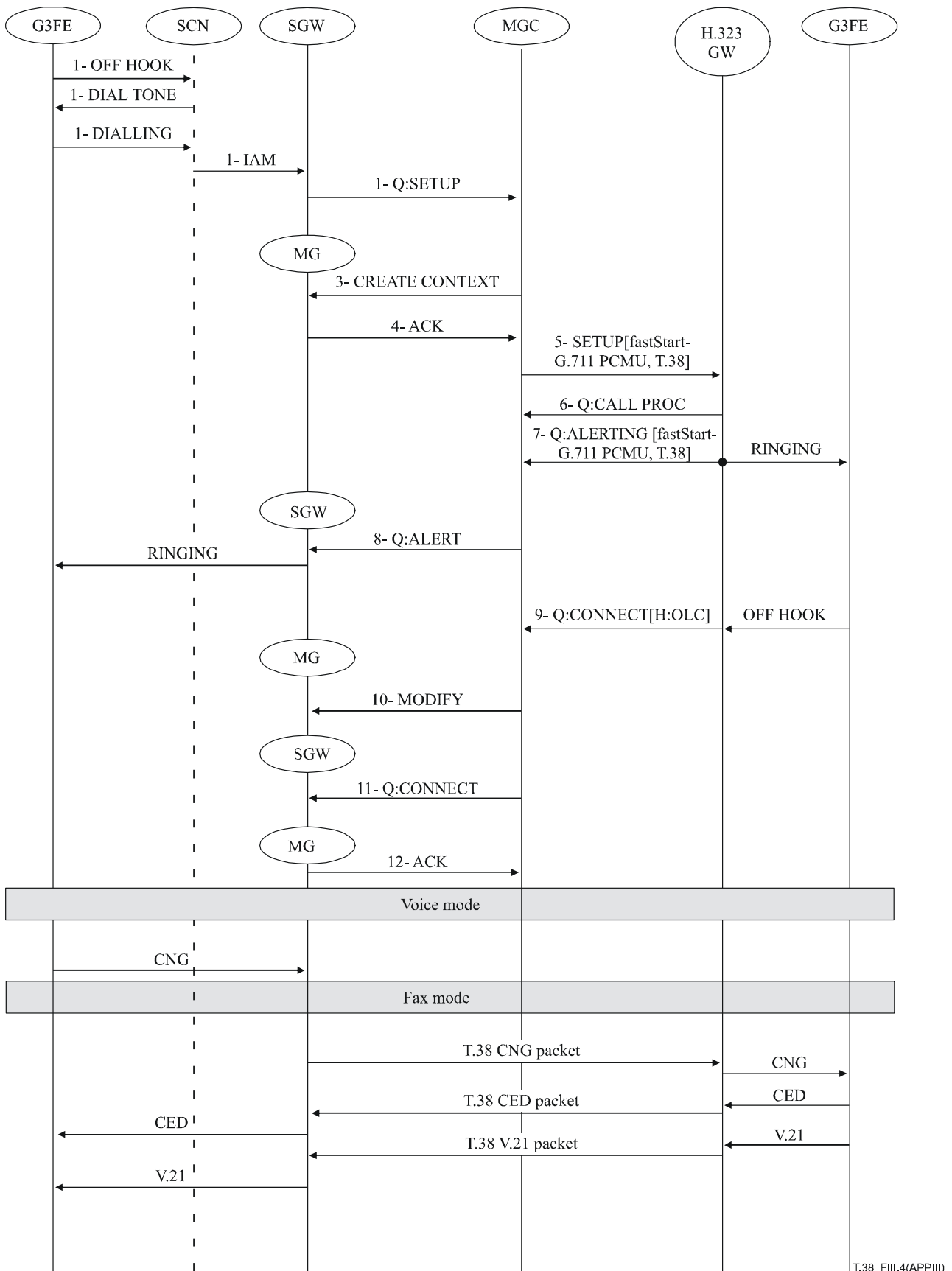
Figure III.4 – Voice to fax call setup with ITU-T H.248 and ITU-T H.323 endpoints that support ITU-T T.38 Autonomous Transition between VoIP and FoIP
