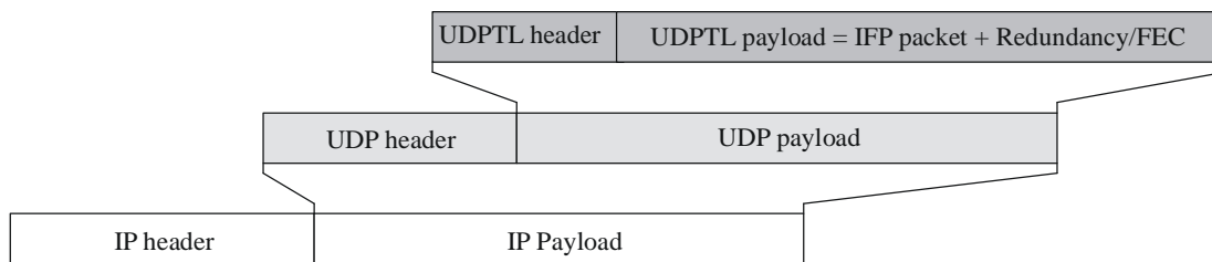
a) Layered model of IFP/UDPTL/UDP/IP packet
