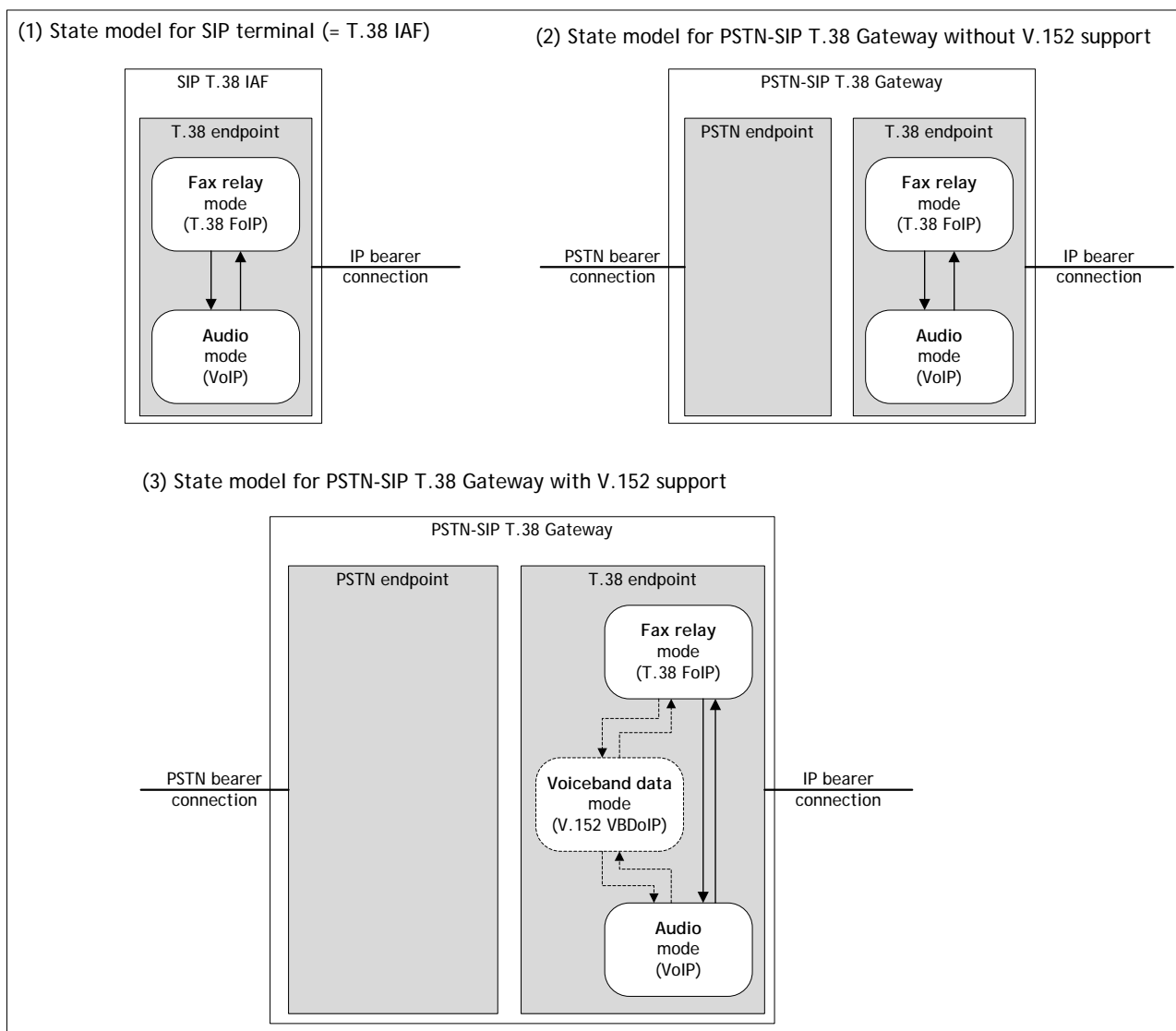
Figure D.1 – State model for the voice and facsimile call – Example ITU-T T.38 SIP equipment
