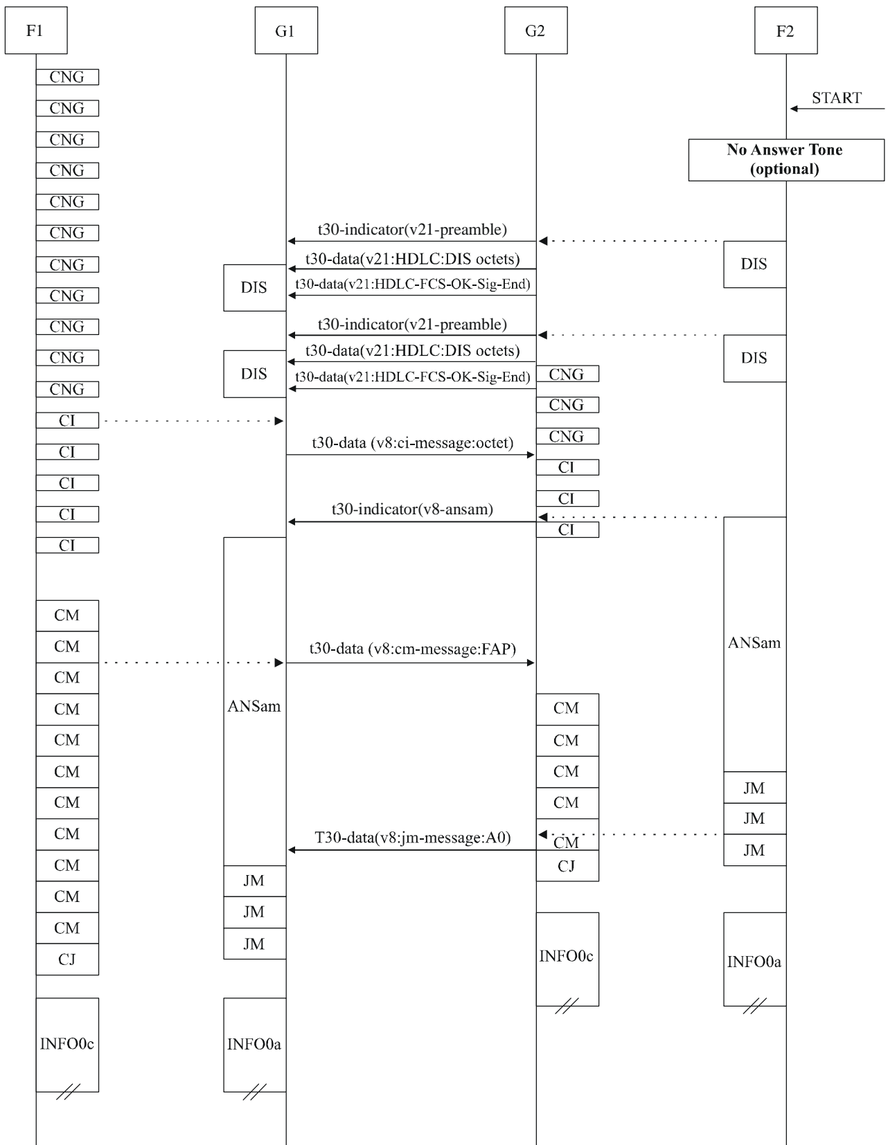
Figure IV.11 – Manual Receive (DIS has bit 6 set to 1 to indicate ITU-T V.8 capability)
