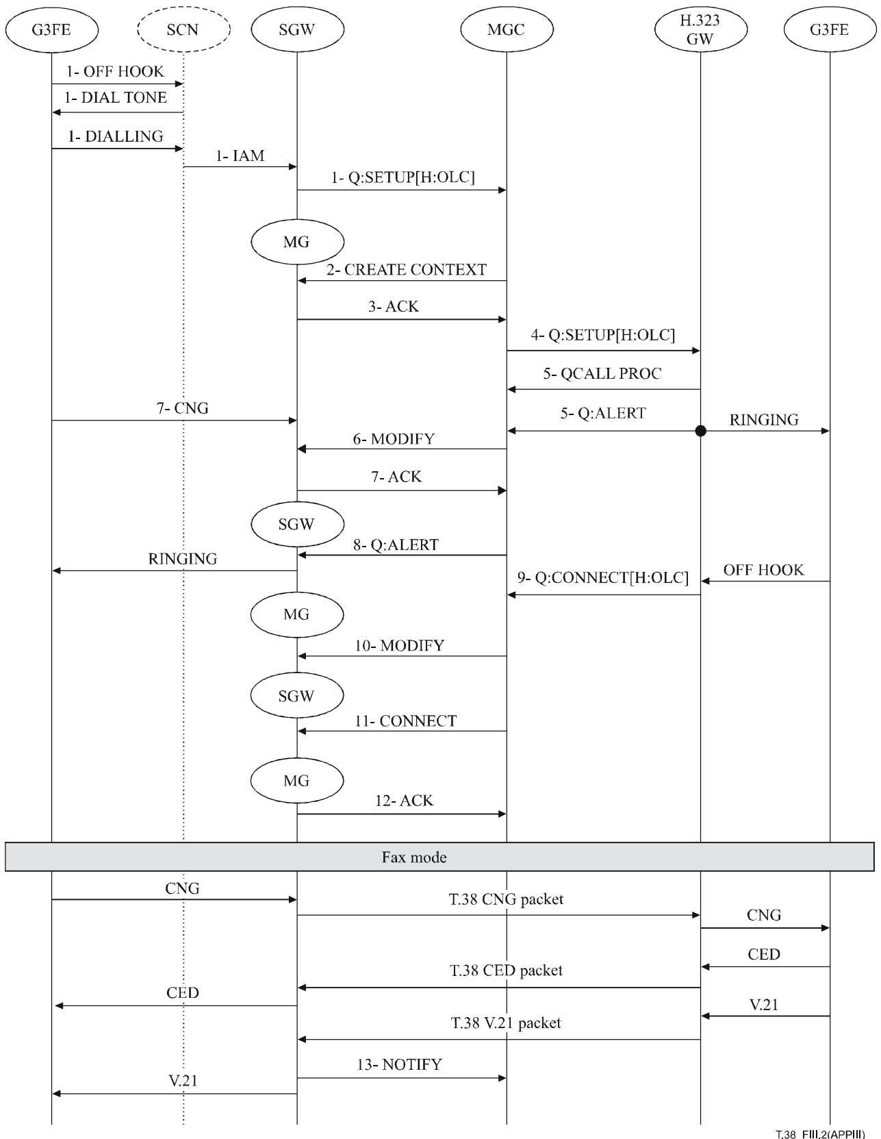
Figure III.2 – Fax-only call setup between ITU-T H.248 and an ITU-T H.323 endpoint
