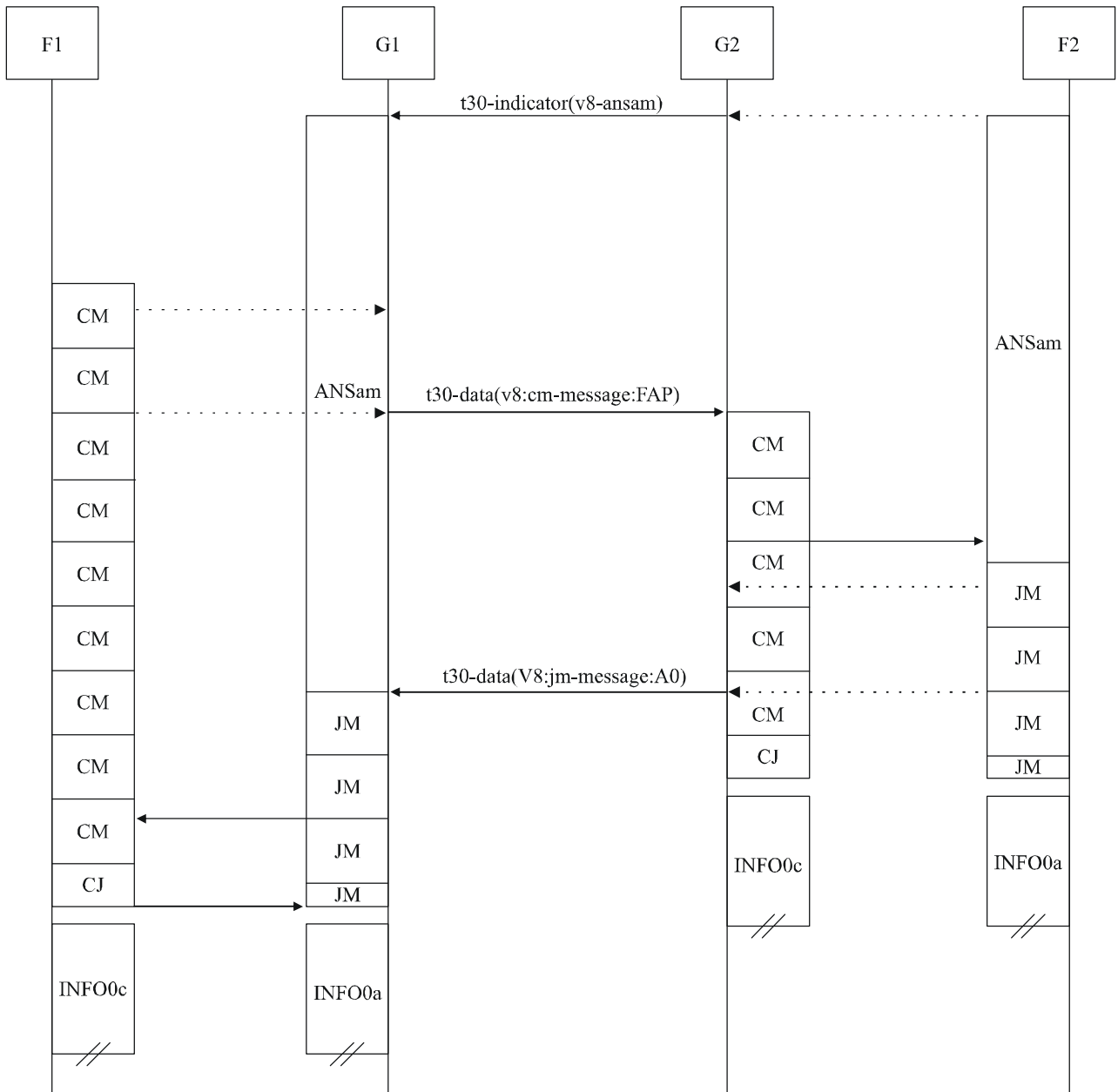
Figure IV.1 – ITU-T V.8 signalling (using profiles and acks)
