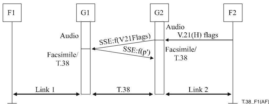
Figure F.1 – ITU-T T.38 FoIP (MoIP transition to ITU-T T.30 fax)
