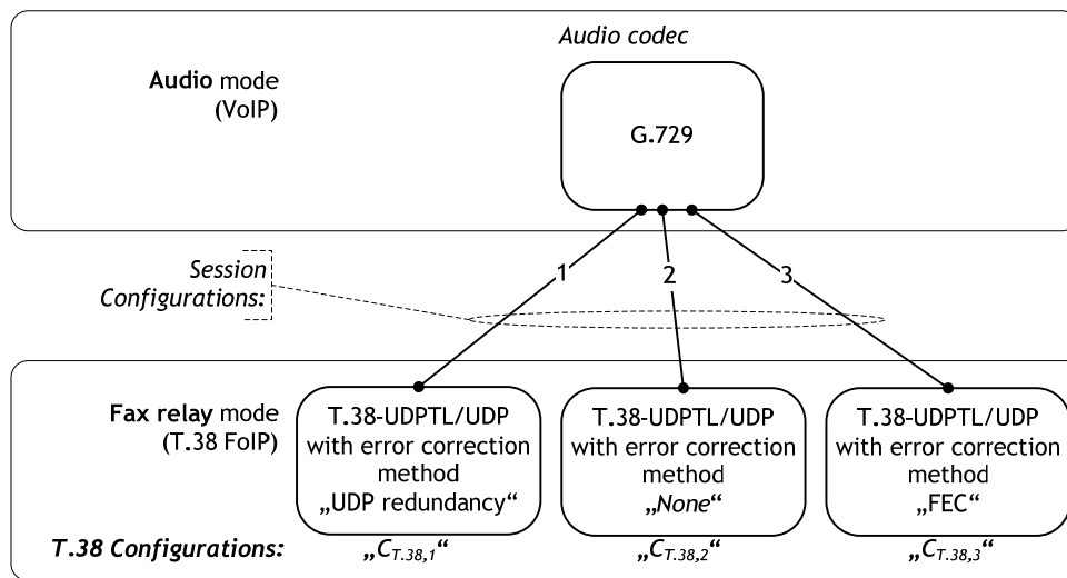
Figure D.7 – Potential session configurations offered in example 6
