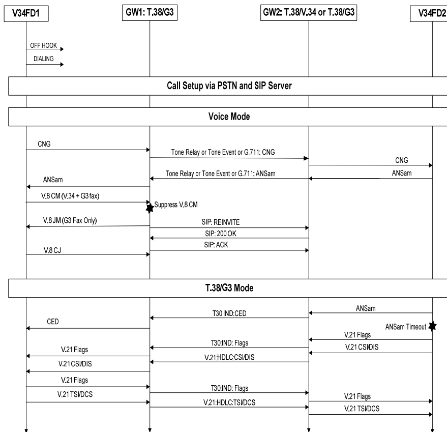
Figure D.2 – Call setup with SIP (fallback from ITU-T V.34 fax to G3), Emitting GW supports G3 only
