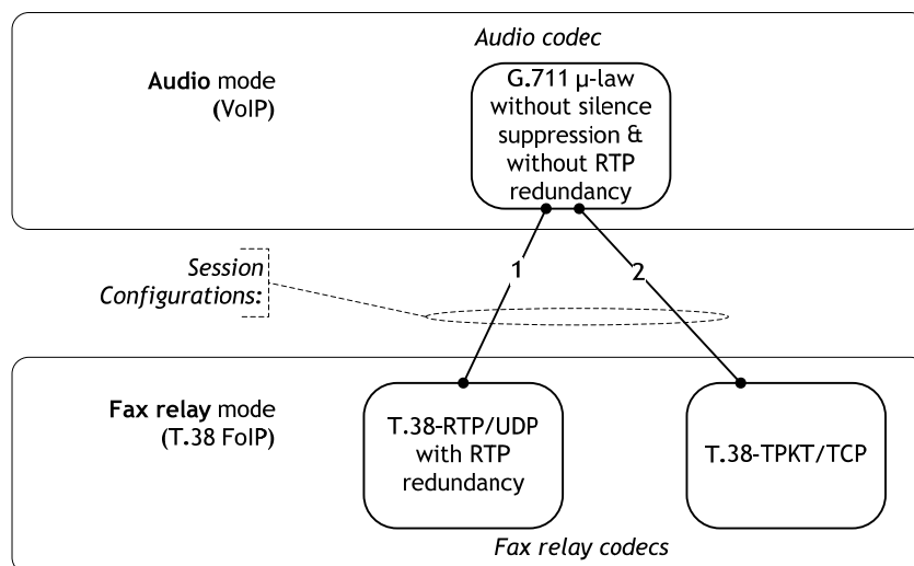
Figure D.4 – Potential session configurations offered in example 3
