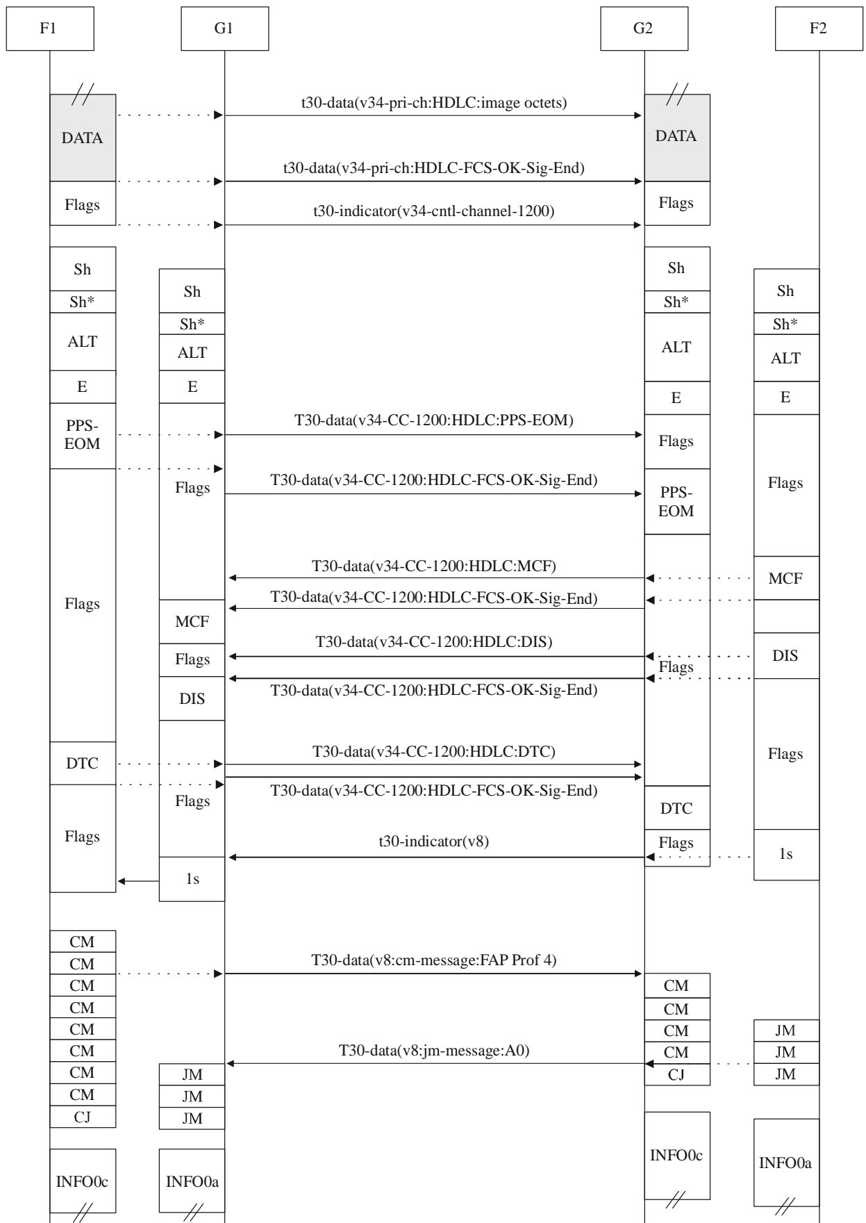
Figure IV.9 – Turn-around polling
