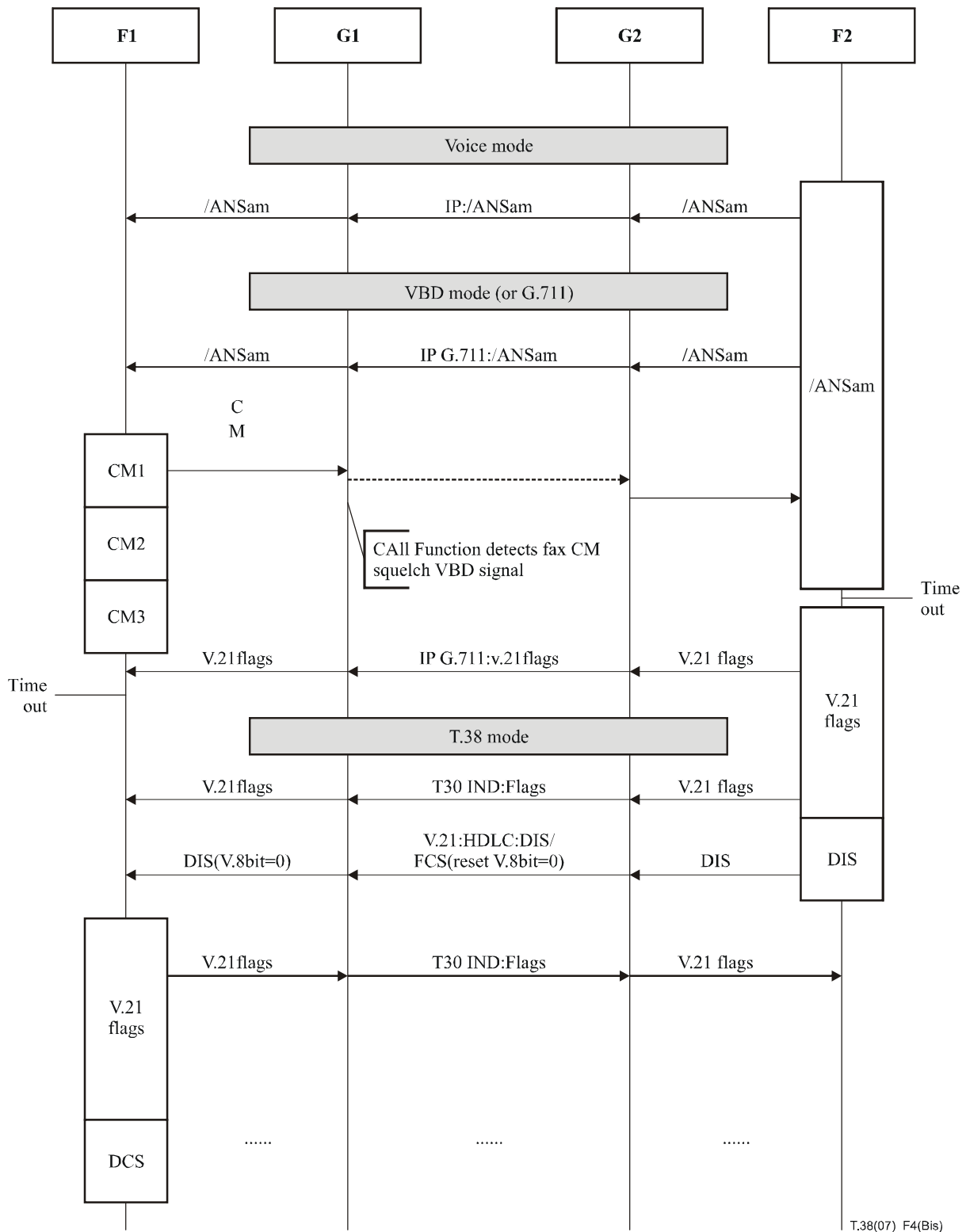
Figure F.4 – ITU-T T.38 FoIP (MoIP fallback and transition to ITU-T T.30 fax by Payload)
