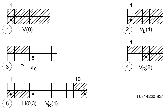
FIGURE 10/T.4 Coding examples: first part of scan line
