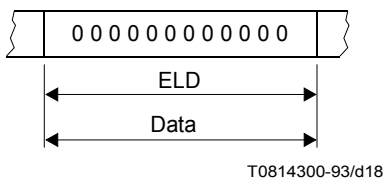
FIGURE B.4/T.4 Data format for the scan line containing 1728 white picture elements
