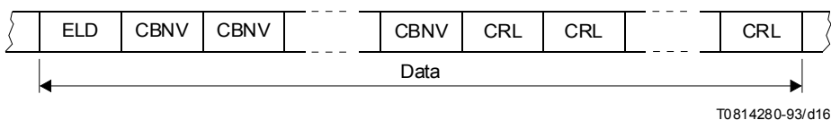
FIGURE B.2/T.4 Data format for the scan line containing several NW-parts
