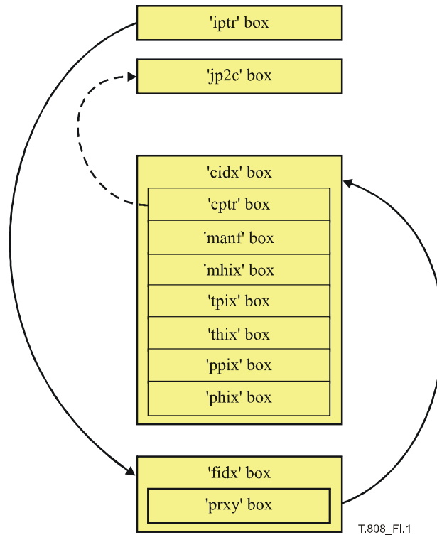
Figure I.1 – Part of an example JPEG 2000 file containing JPIP index boxes
