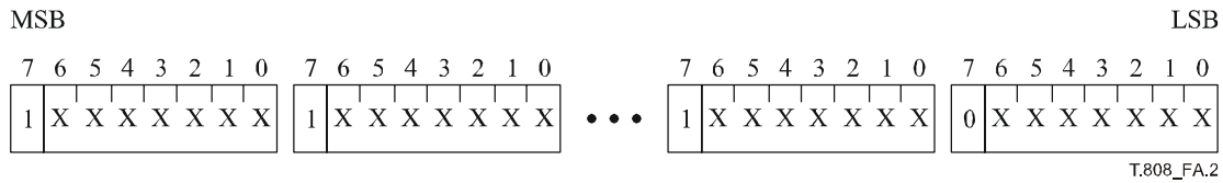
Figure A.2 – VBAS structure
