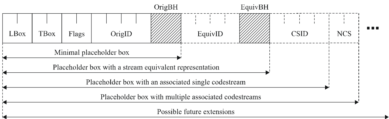
Figure A.11 – Placeholder box structure
