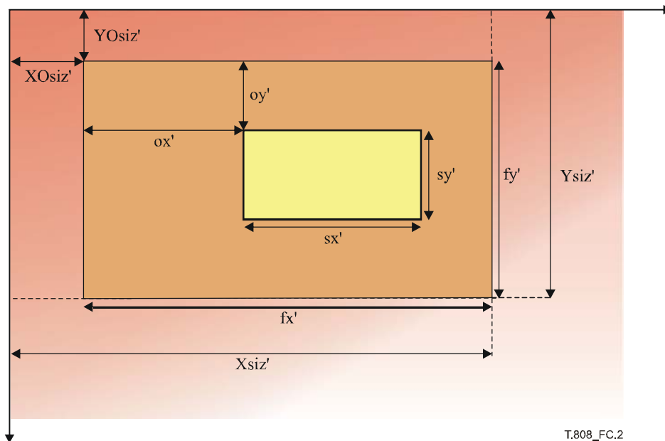
Figure C.2 – Desired region with respect to the subsampled reference grid
