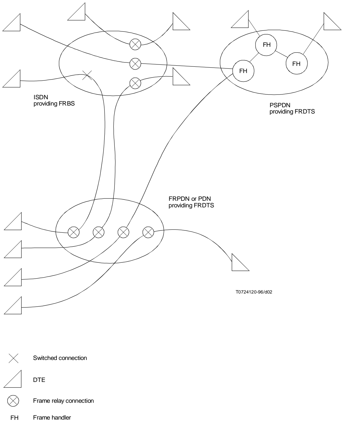
FIGURE 2/X.7 Various networks providing Frame Relay Data Transmission Service (FRDTS) and Frame Relaying Bearer Service (FRBS)
