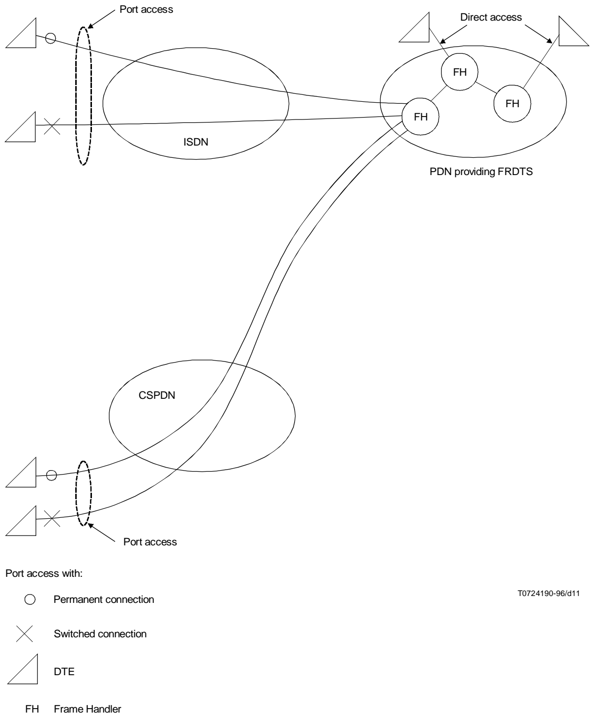
FIGURE 11/X.7 Access mechanisms for frame relay data transmission services
