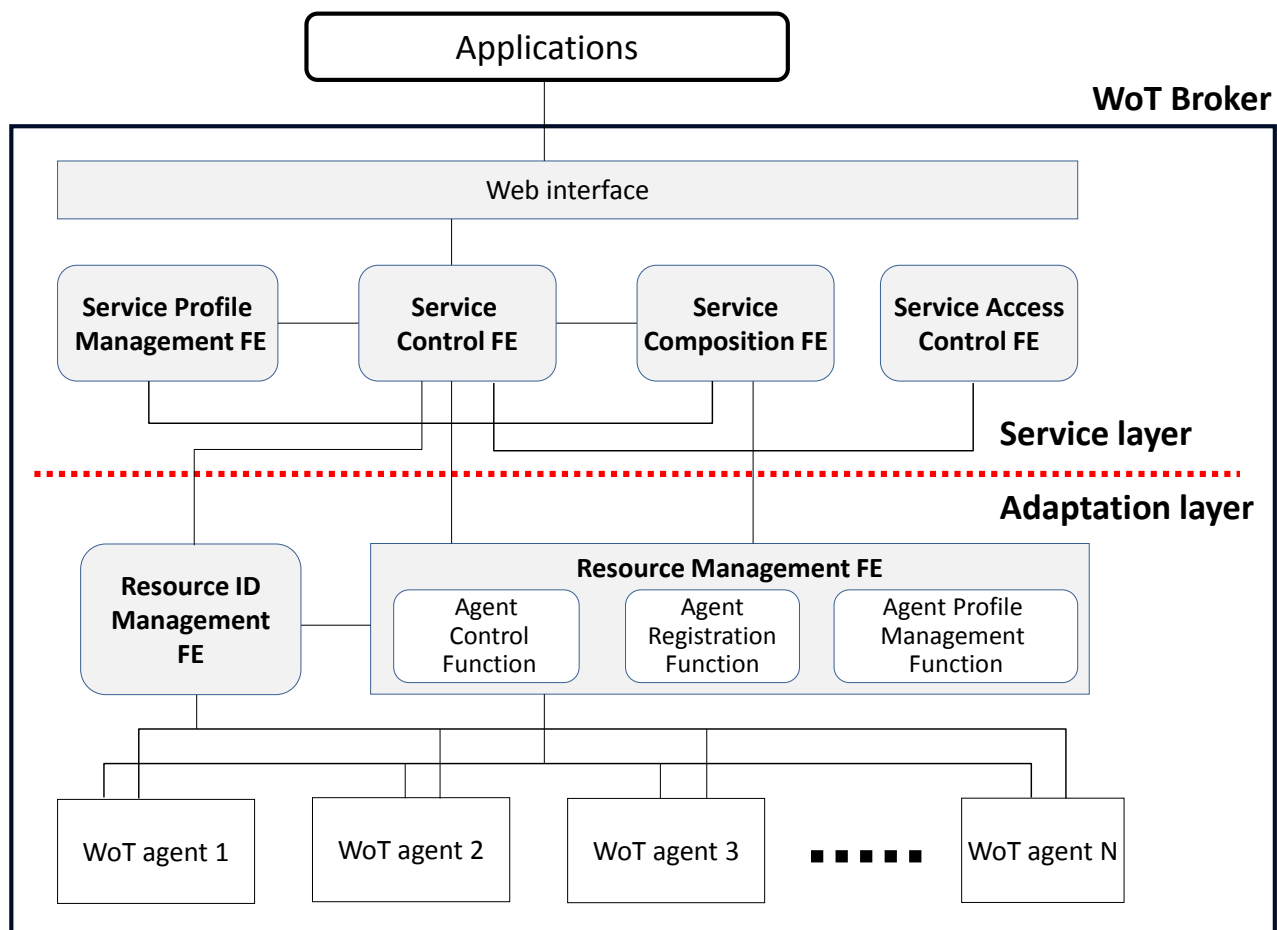
Figure 9-2– Functional architecture of the WoT broker
