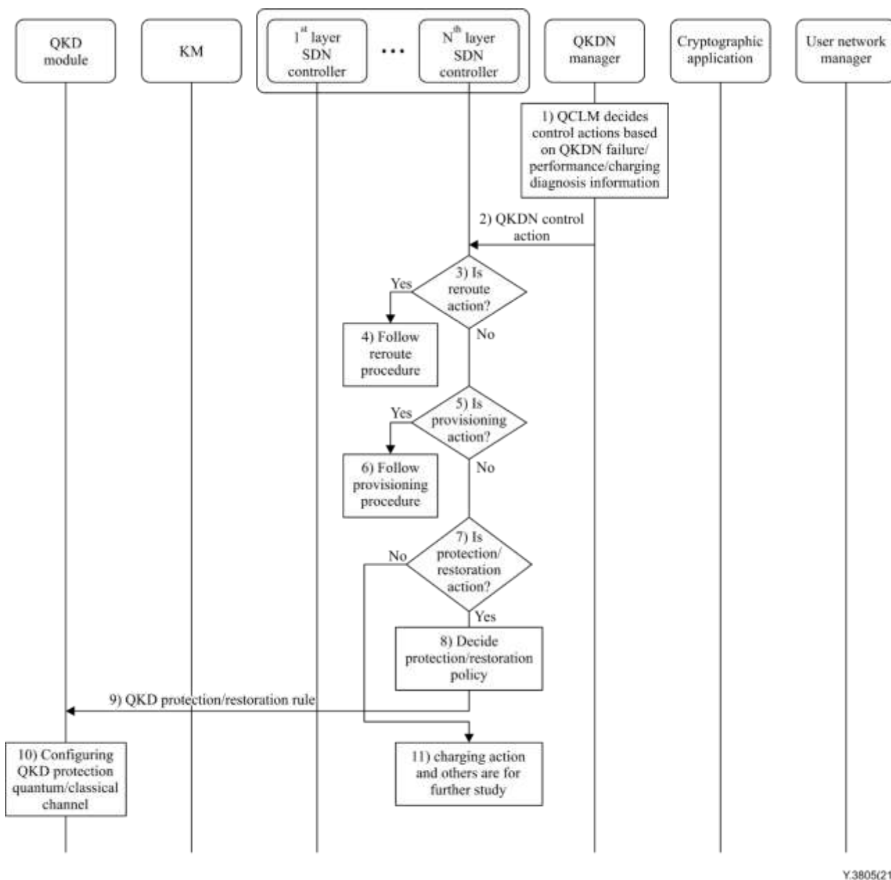
Figure 13 – An example of a QKDN control action procedure including hierarchical SDN control associated with QKDN management
