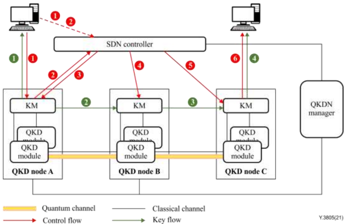
Figure II.3 – Diagram of control method in SDN-based QKDN with an SDN controller
