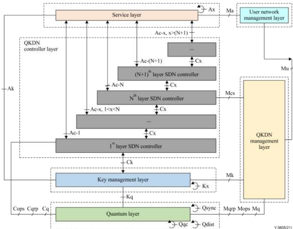
Figure 2 – A hierarchical SDN controller in a QKDN
