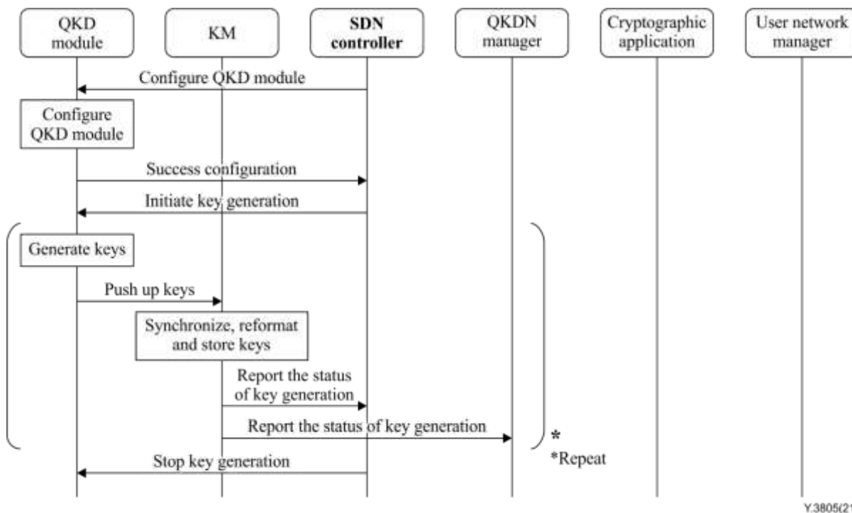
Figure 6 – An example of a key generation phase
