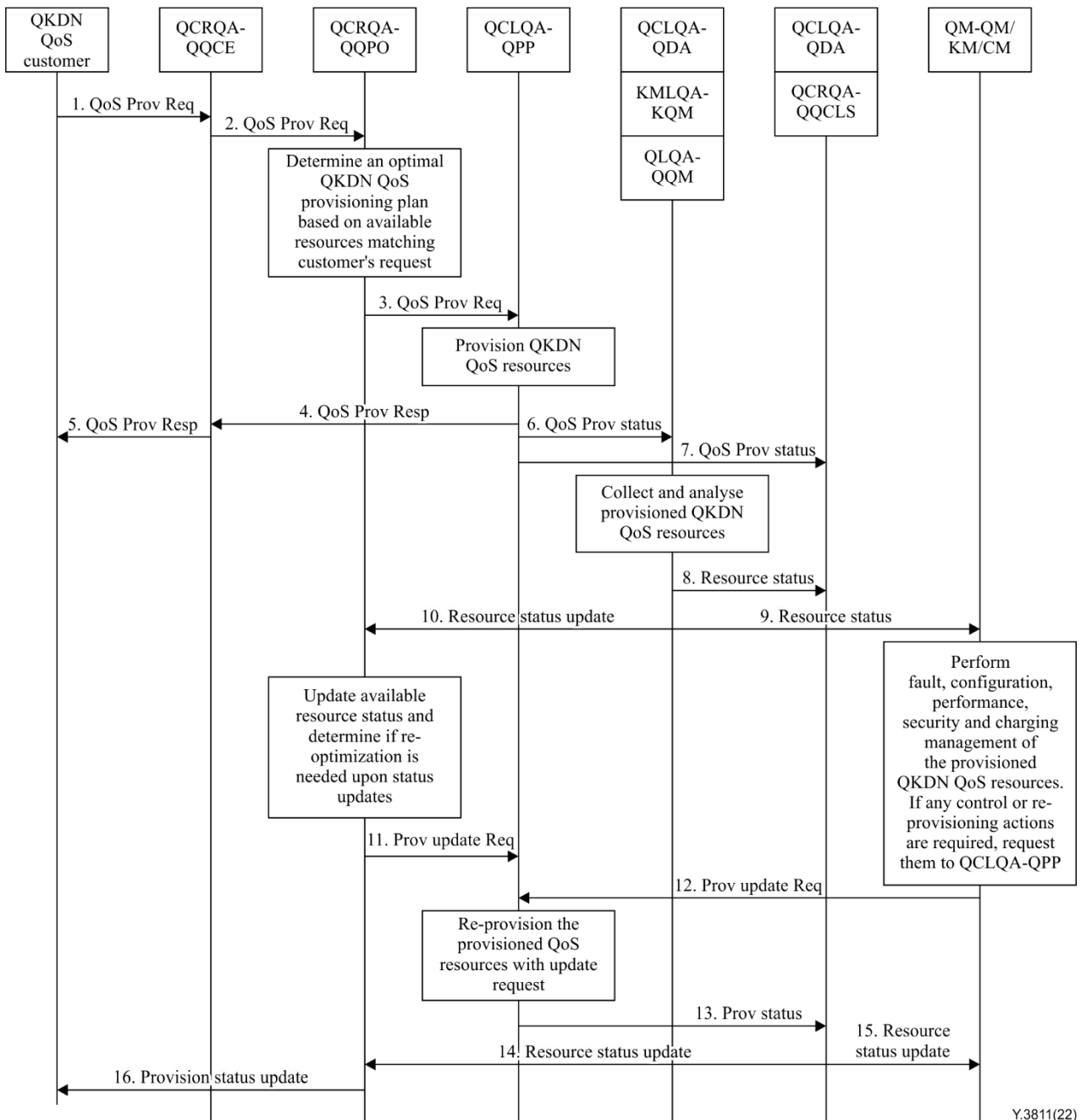
Figure 3 – A basic operational procedure for QKDN QoS assurance
