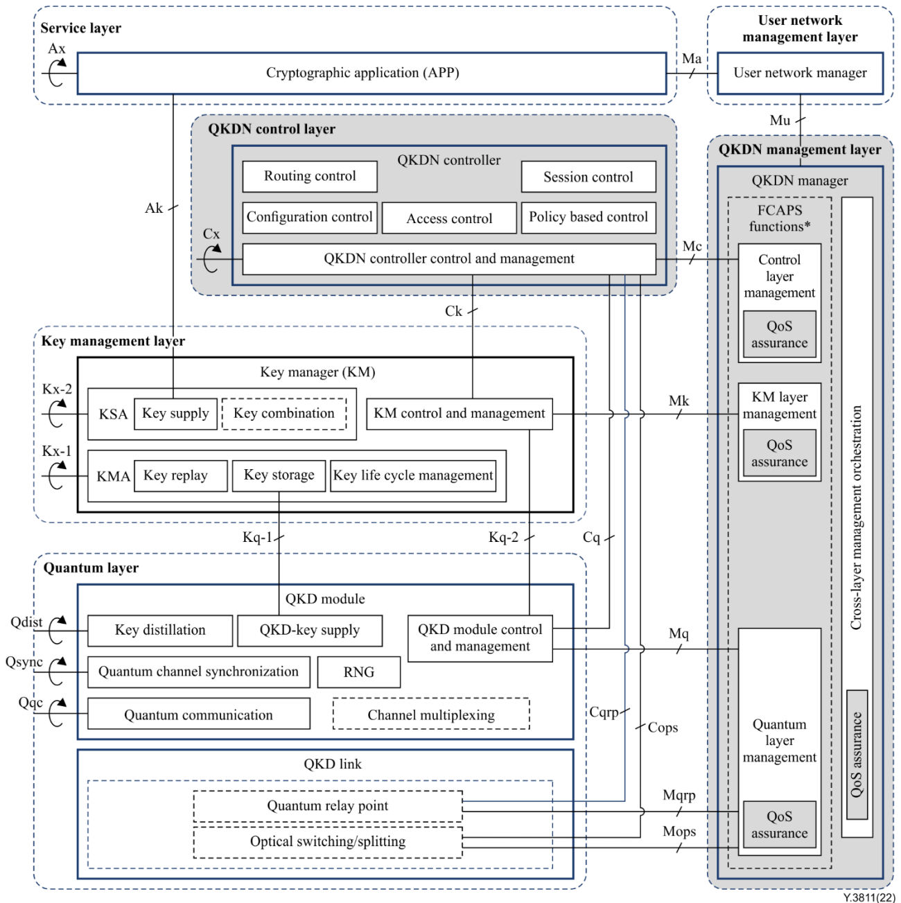
Figure 1 – Functional architecture of QoS assurance for QKDN
