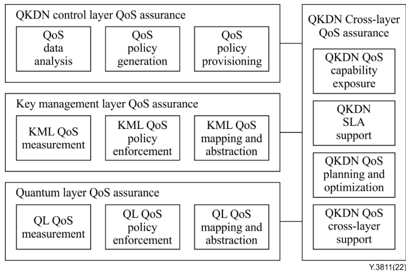
Figure 2 – QKDN QoS assurance functional entities
