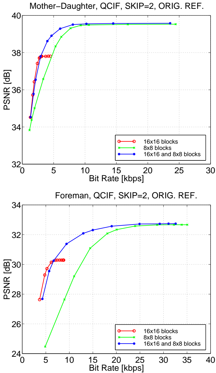
Figure 3: Prediction gain vs. MV bit rate for the sequence Mother & Daughter (top) and Foreman (bottom) when employing H.263 MV median prediction and original frames as reference frames.
