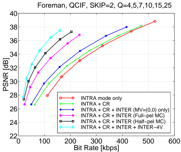
Figure 2: Coding performance for the sequence Mother & Daughter (top) and Foreman (bottom).
