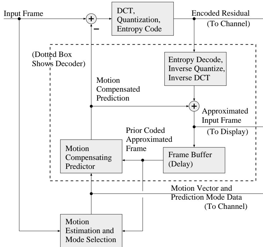
Figure 1: Typical Motion Compensated DCT Video Coder
