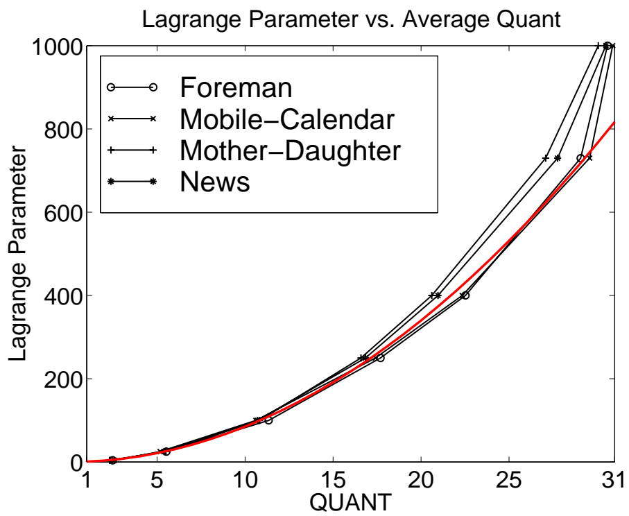
Figure 6: Lagrange parameter \lambda_{\text{MODE}} vs. average macroblock QUANT.
