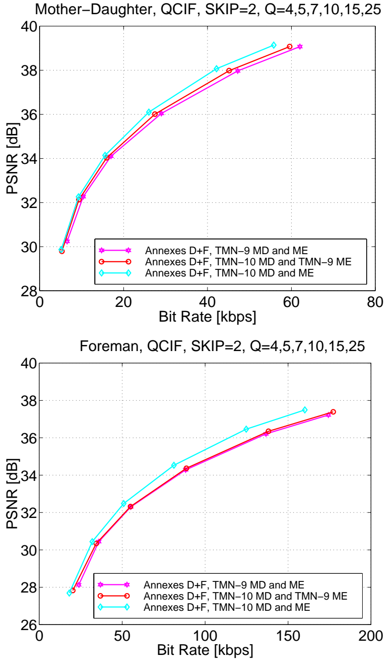
Figure 7: Coding performance for the sequence Mother & Daughter (top) and Foreman (bottom) when comparing the TMN-9 to the TMN-10 encoding strategy.
