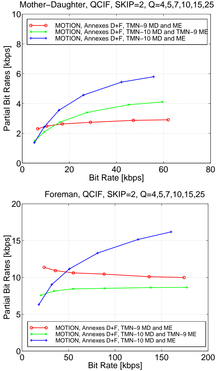
Figure 8: Bit rate partition of MVs vs. bit rate for the sequence Mother & Daughter (top) and Foreman (bottom) when employing TMN-10 mode decision and motion estimation.
