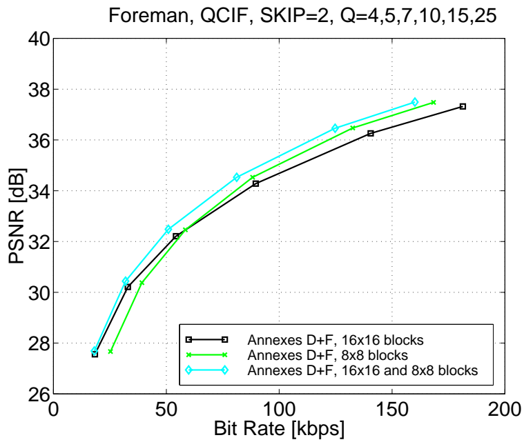
Figure 4: Coding performance for the sequence Mother & Daughter (top) and Foreman (bottom) when employing variable block sizes.
