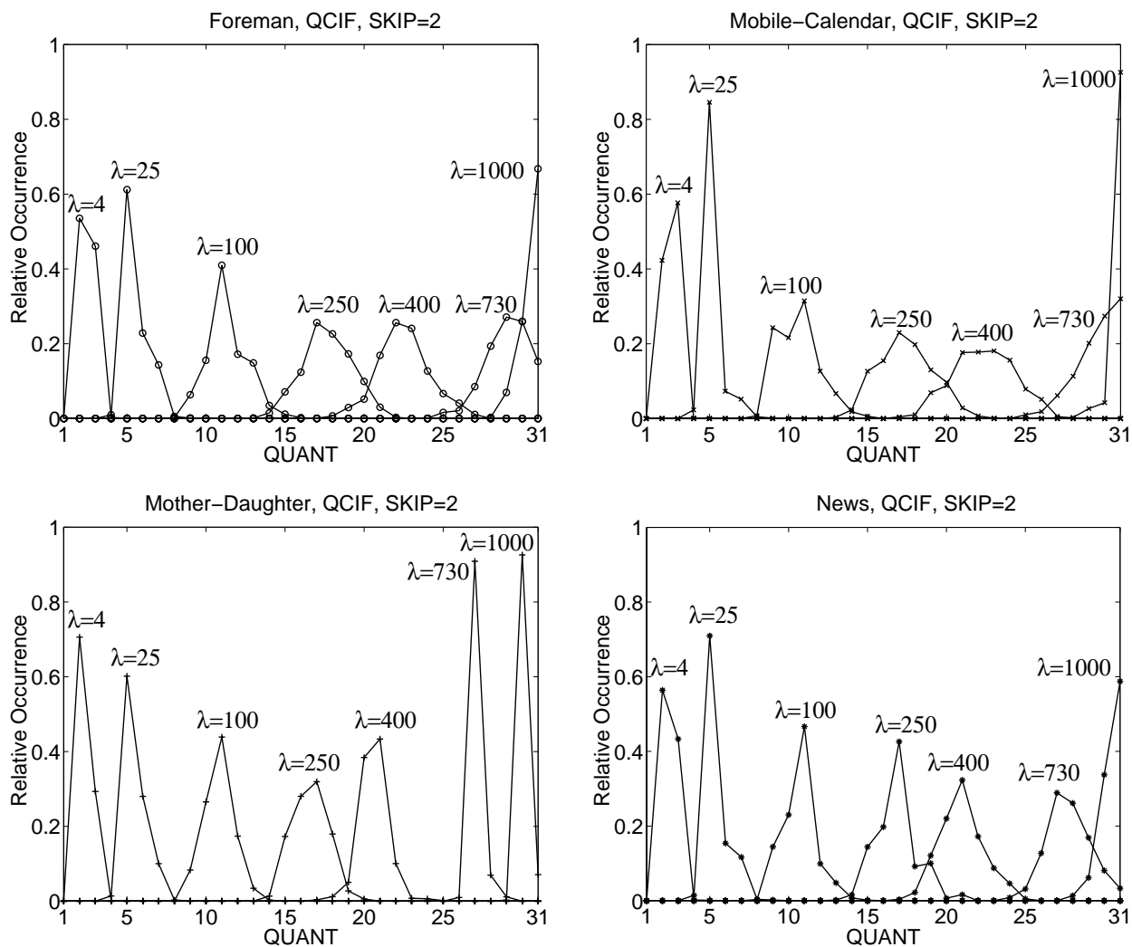
Figure 5: Relative occurrence vs. macroblock QUANT for various Lagrange parameter settings. The relative occurrences of macroblock QUANT values are gathered while coding 100 frames of the video sequences Foreman (top left), Mobile & Calendar (top right), Mother & Daughter (bottom left), and News (bottom right).
