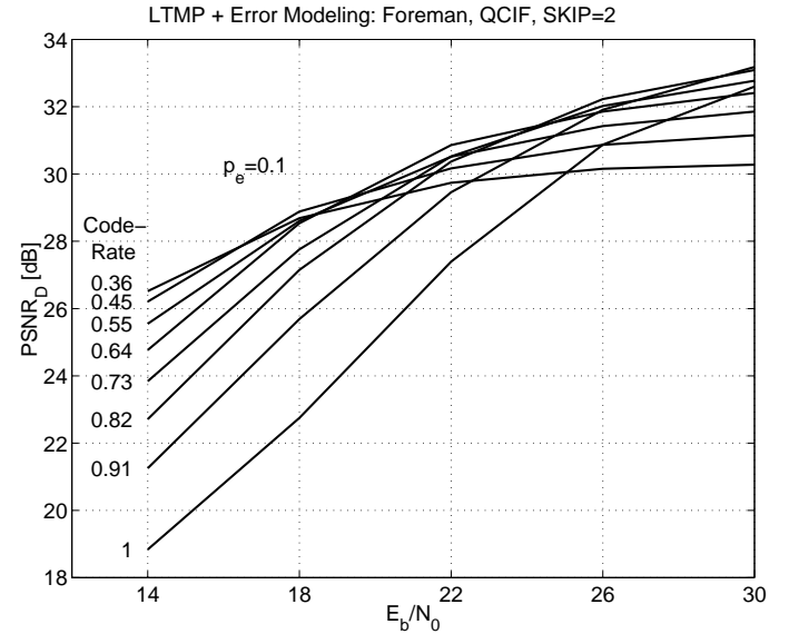
Fig. 8. Average decoder PSNR vs. E_b/N_0 for the sequence Foreman when running the LTMP coder.
