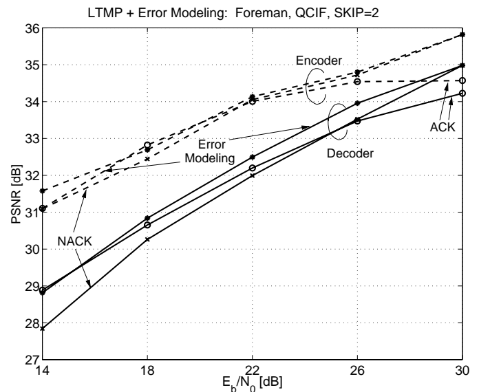
Fig. 11. Average PSNR vs. E_b/N_0 for the sequence Foreman running the TMN-10 codec (top) and the LTMP codec (bottom) when feedback is utilized. The various curves correspond to decoder and encoder PSNR for three different feedback handling strategies.
