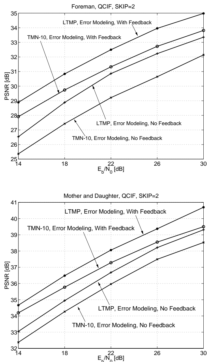
Fig. 12. Average PSNR vs. E_b/N_0 for the sequences Foreman (top) and Mother and Daughter (bottom) for the optimal feedback strategy.
