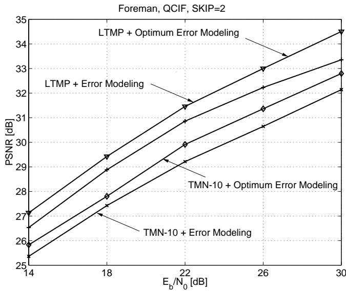
Fig. 10. Average decoder PSNR vs. E_b/N_0 for the sequence Foreman (top) when comparing the results of optimal code-rate and error model parameter p_e for our approximative error modeling to optimum error modeling.
