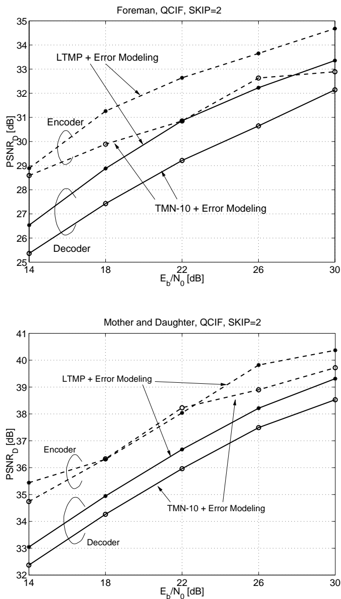
Fig. 9. Average decoder PSNR vs. E_b/N_0 for the sequences Foreman (top) and Mother and Daughter (bottom) for the optimal code-rate and error model parameter p_e without feedback.
