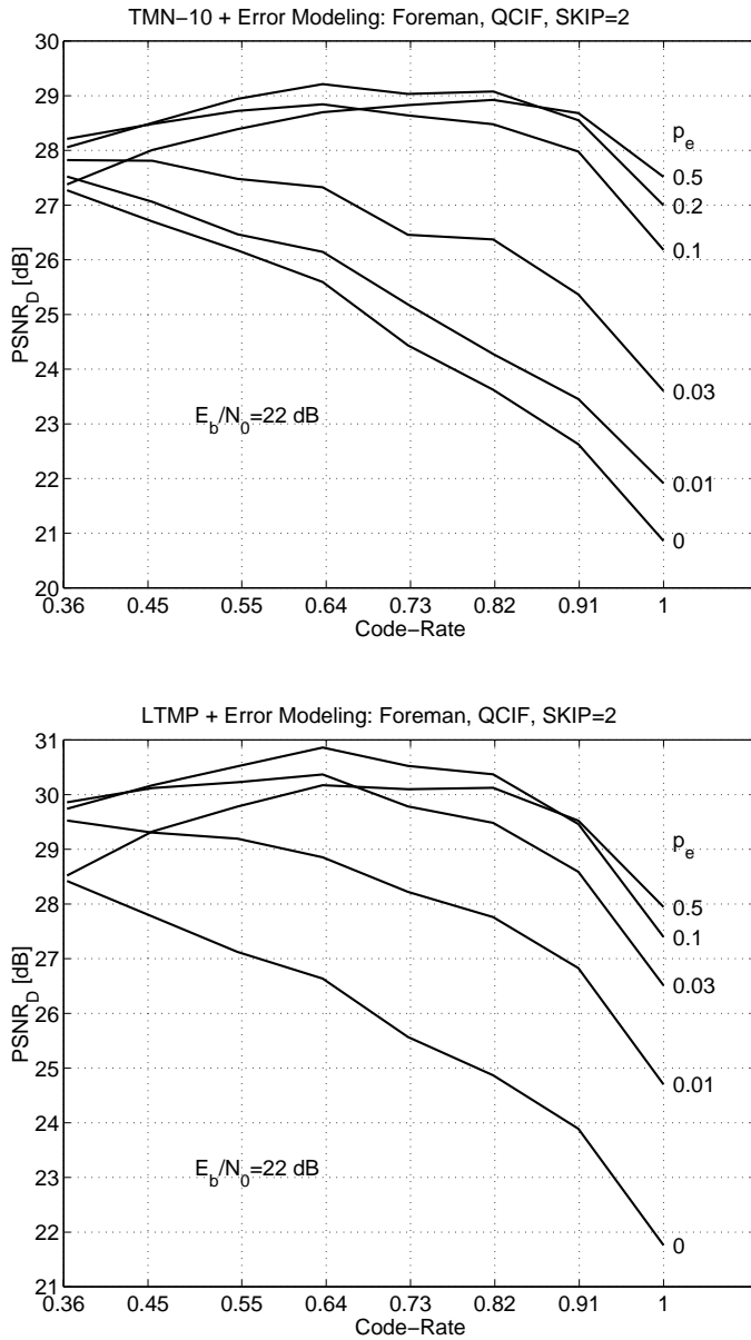
Fig. 7. Average decoder PSNR vs. code-rate for the sequence Foreman when running the TMN-10 coder (top) and the LTMP coder (bottom).
