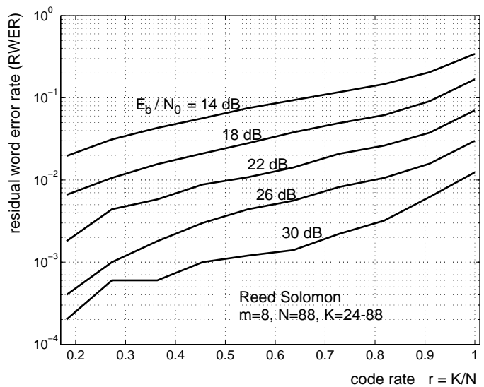
Fig. 4. Residual word error rate (RWER) after channel coding for a Rayleigh fading channel (Doppler frequency f_D = 2.5 Hz) with Gaussian Frequency Shift Keying.
