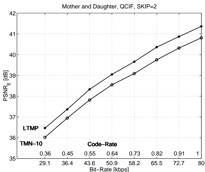
Fig. 5. Average PSNR vs. average bit-rate or code-rate for the sequences Foreman (top) and Mother and Daughter (bottom). The two curves relate to the two coders compared: (i) TMN-10, the test model of the H.263 standard with Annexes D, F, I, J, T enabled; (ii) LTMP: the long-term memory prediction coder with 10 frames also utilizing Annexes D, F, I, J, T.
