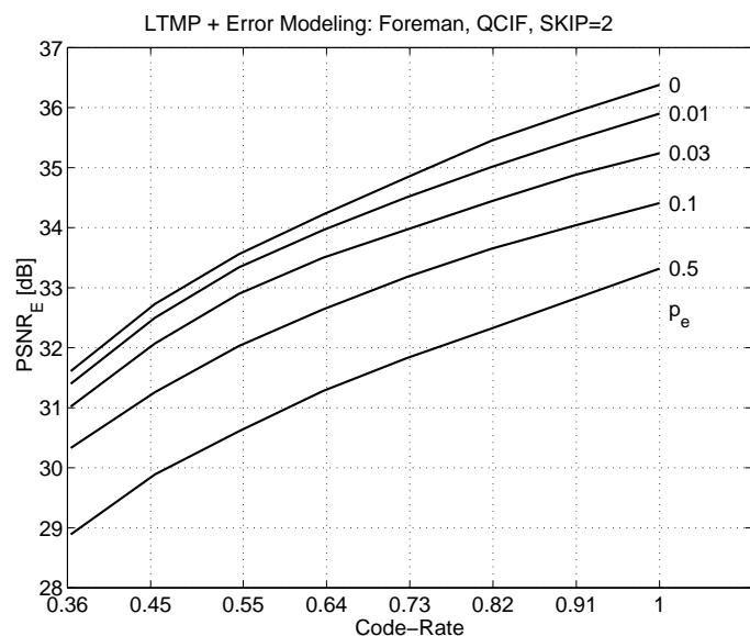
Fig. 6. Average encoder PSNR vs. code-rate for the sequence Foreman when running the TMN-10 coder (top) and the LTMP coder (bottom).
